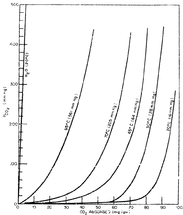
Fig. 11 - CO 2 equilibrium curves for amine resin containing 45 percent water (DET + Epon 562). (Water vapor pressure in equilibrium with amine resin given in parentheses for each temperature plotted.)
