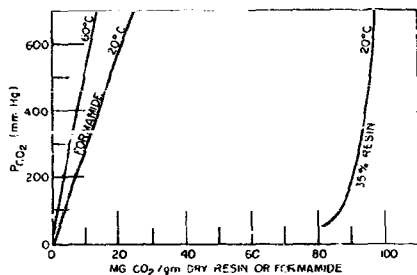
Fig. 12 - \text{CO}_2 equilibrium curves for formamide and formamide-swelled resin
