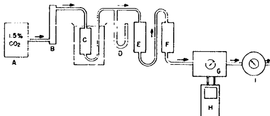
Fig. 4 - Amine resin absorption rate apparatus: A - supply tank; B - flowmeter; C - saturator tube filled with water-soaked porous \text{Al}_2\text{O}_3 beads in a constant-temperature water bath; D - water manometer; E - absorption tube; F - drying tube filled with Drierite; G - Liston-Becker infrared \text{CO}_2 analyzer (Model II); H - Esterline-Angus recorder; I - wet test gas meter
