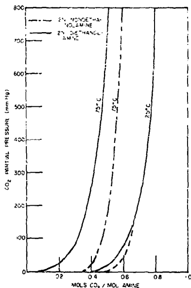
Fig. 15 - \text{CO}_2 equilibrium curves for two monomeric amines (from J. W. Mason and B.F. Dodge, Trans. Am. Inst. Chem. Engrs. 32:27, 1936)
