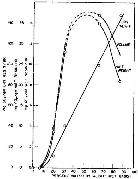
Fig. 6 - Absorption rate vs water content. Resin: DET + Epon 562, less than 30 mesh when dry.
