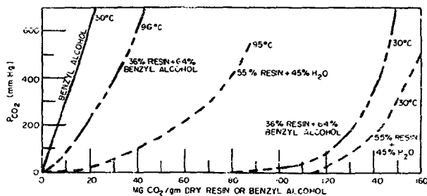
Fig. 14 - \text{CO}_2 equilibrium curves for benzyl alcohol, benzyl-alcohol-swelled resin, and water-swelled resin
