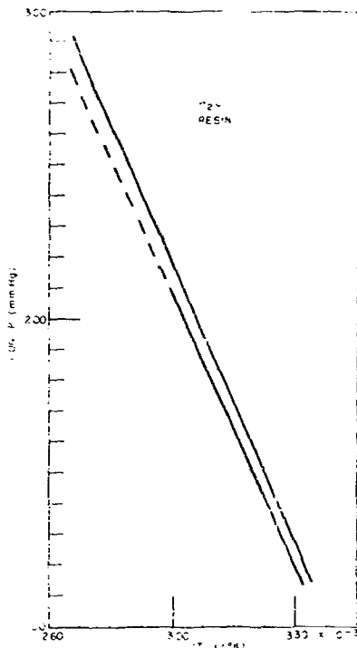
Fig. 10 - Water vapor pressure vs temperature for amine resin containing 45 percent water: (DET + Epon 562)
