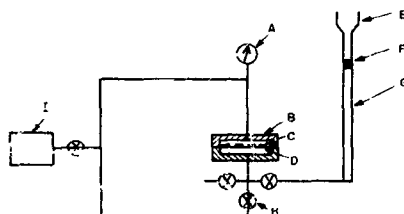
Fig. 2 - Apparatus to measure membrane permeabilities: A - vacuum gage; B - frame to hold test membranes; C - coarse screen backing for test membranes; D - test membrane; E - mercury trap; F - mercury drop; G - calibrated glass capillary tube; H - Hoke valve; I - vacuum pump
