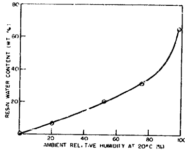
Fig. 5 - Water content vs relative humidity. Resin: DET + Epon 562, less than 30 mesh when dry.
