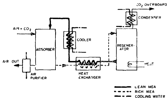
Fig. 1 - A typical ethanolamine scrubber
