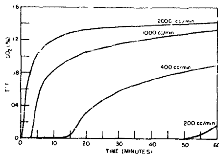
Fig. 7 - Absorption efficiency vs time at various flow rates. Resin: DET + Epon 562.
