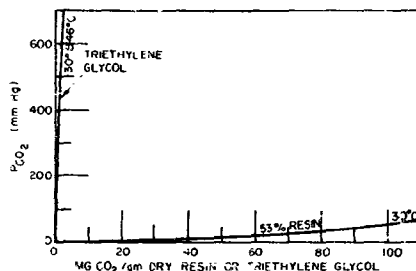
Fig. 13 - \text{CO}_2 equilibrium curves for triethylene glycol and triethylene-glycol-swelled resin
