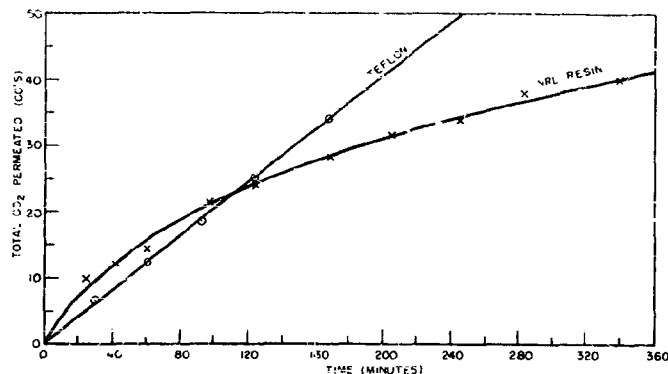
Fig. 3 - CO 2 permeability of Teflon and of an NRL resin
