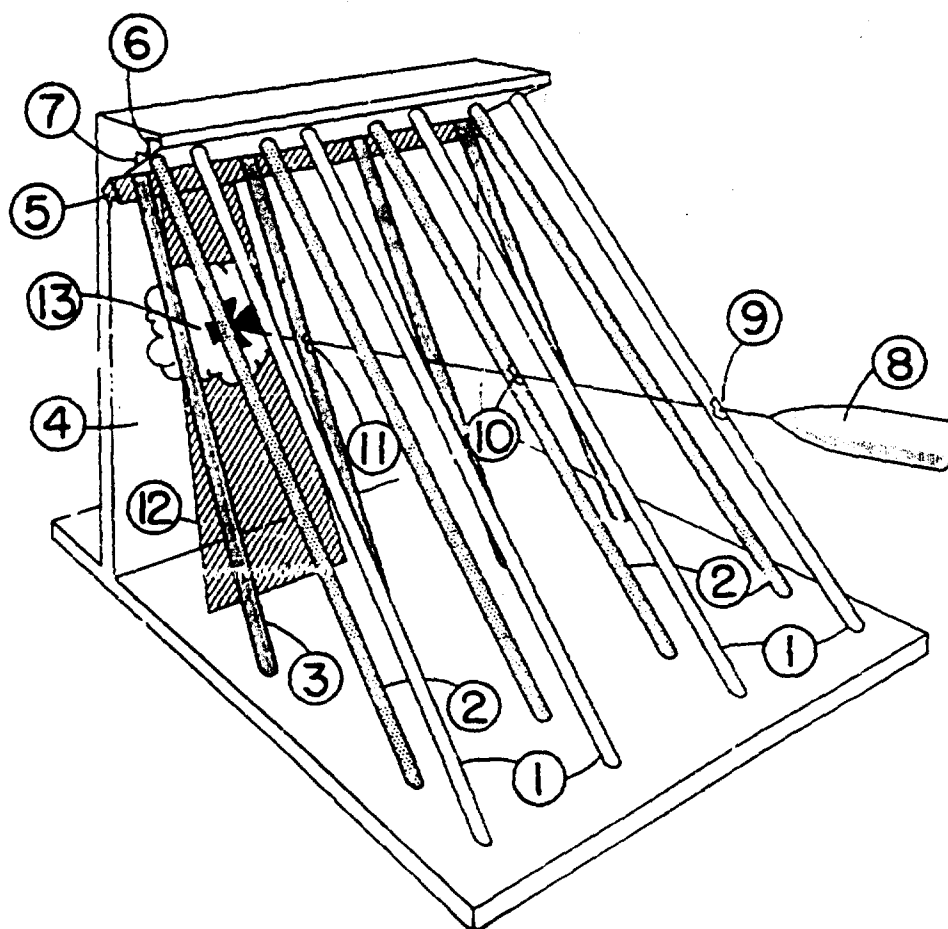
Figure 1. Diagram of dynamic armor sensing system.
