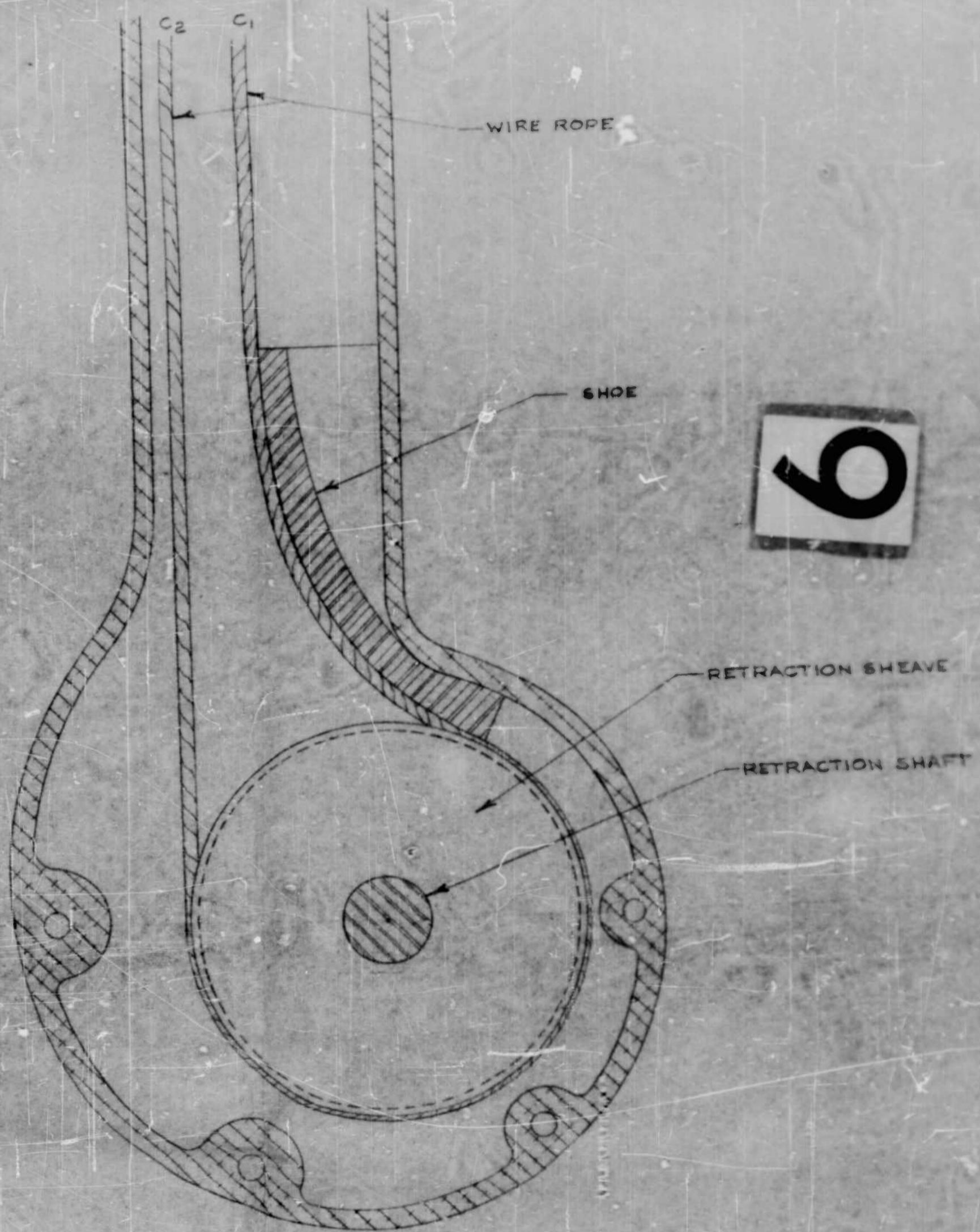
SECTION C-C
