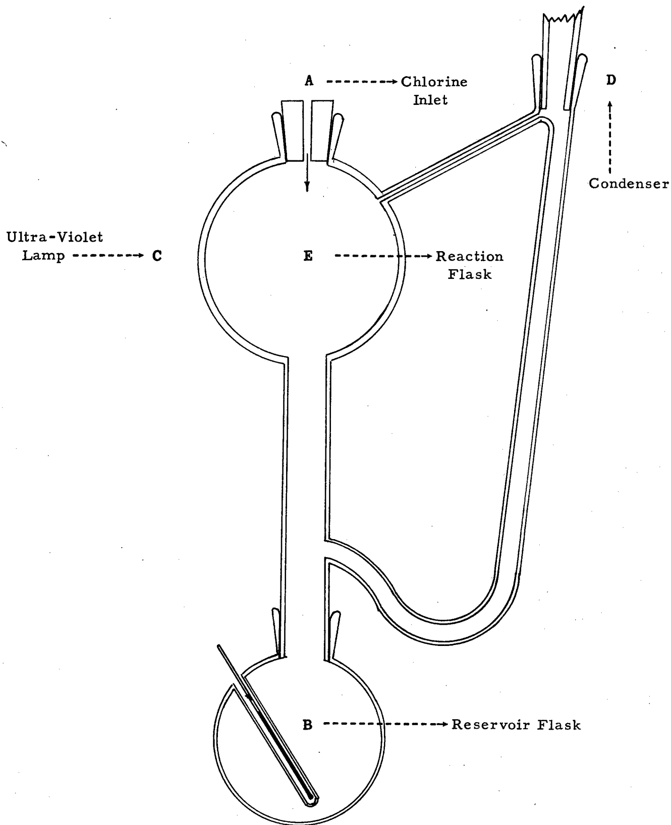
FIGURE 1. Chlorination Apparatus
