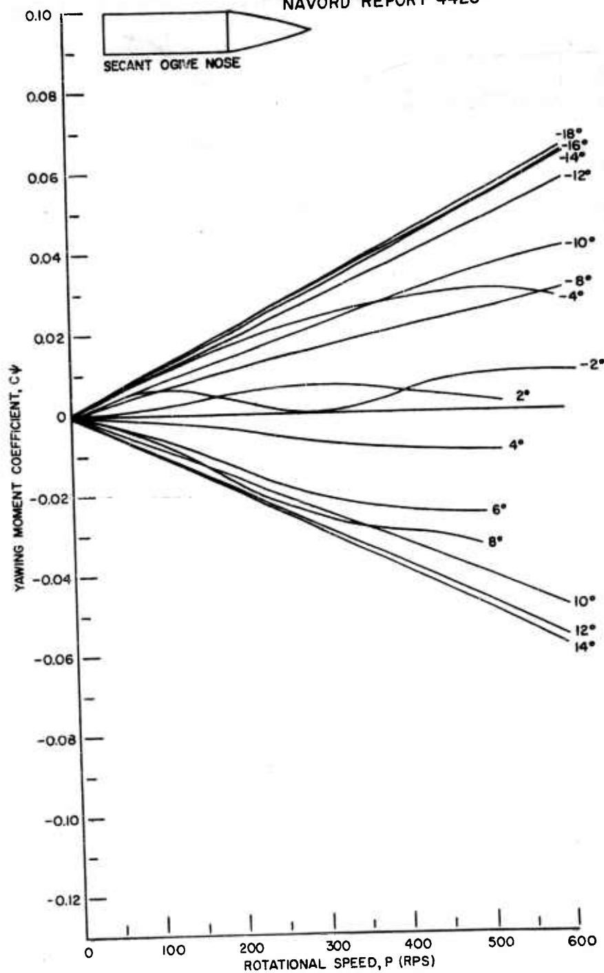
FIG. 25 YAWING MOMENT COEFFICIENT, C \psi , VS ROTATIONAL SPEED, P,-SECANT OGIVE NOSE
