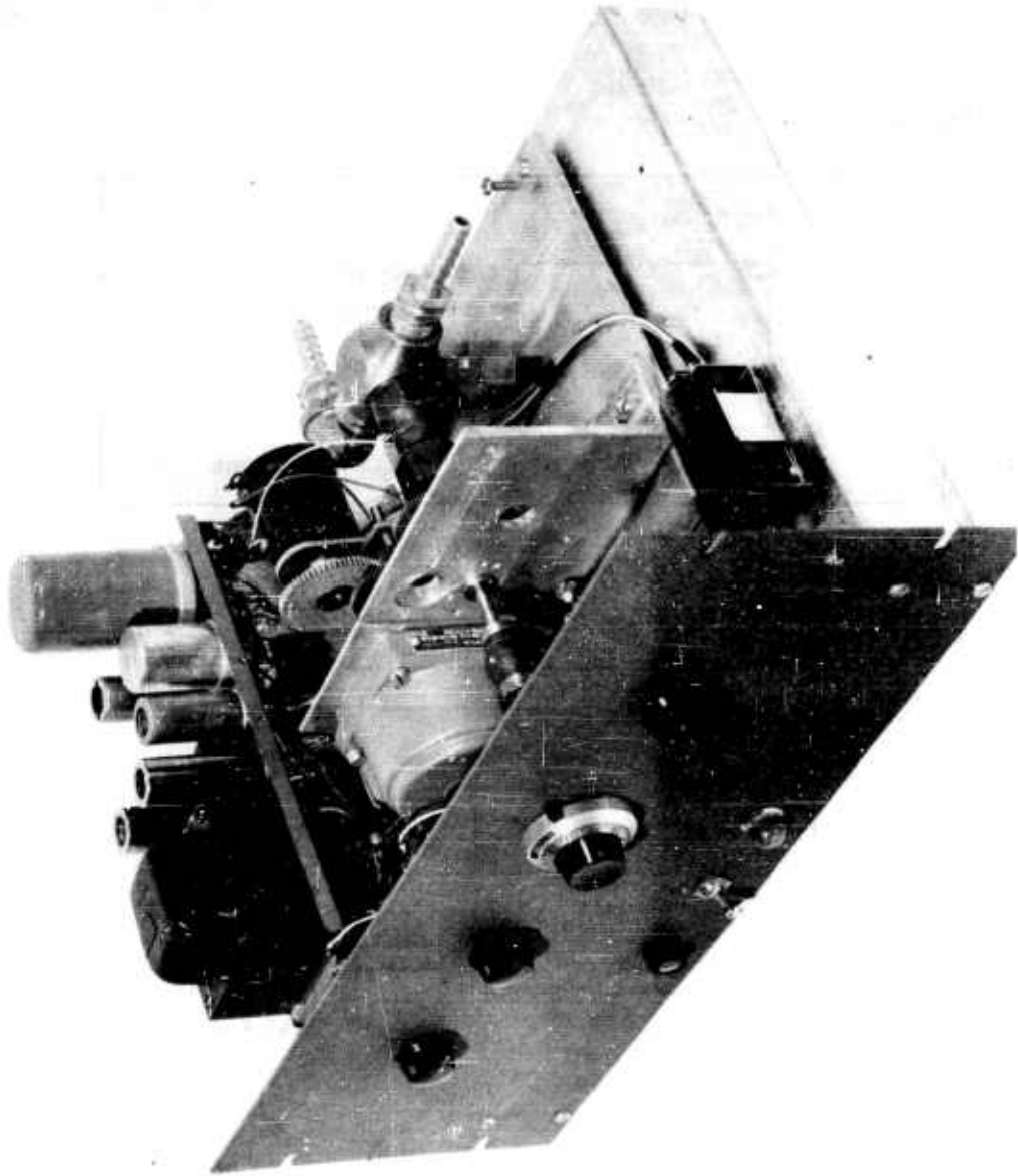
FIG. 10 SERVO-SPEED CONTROL
