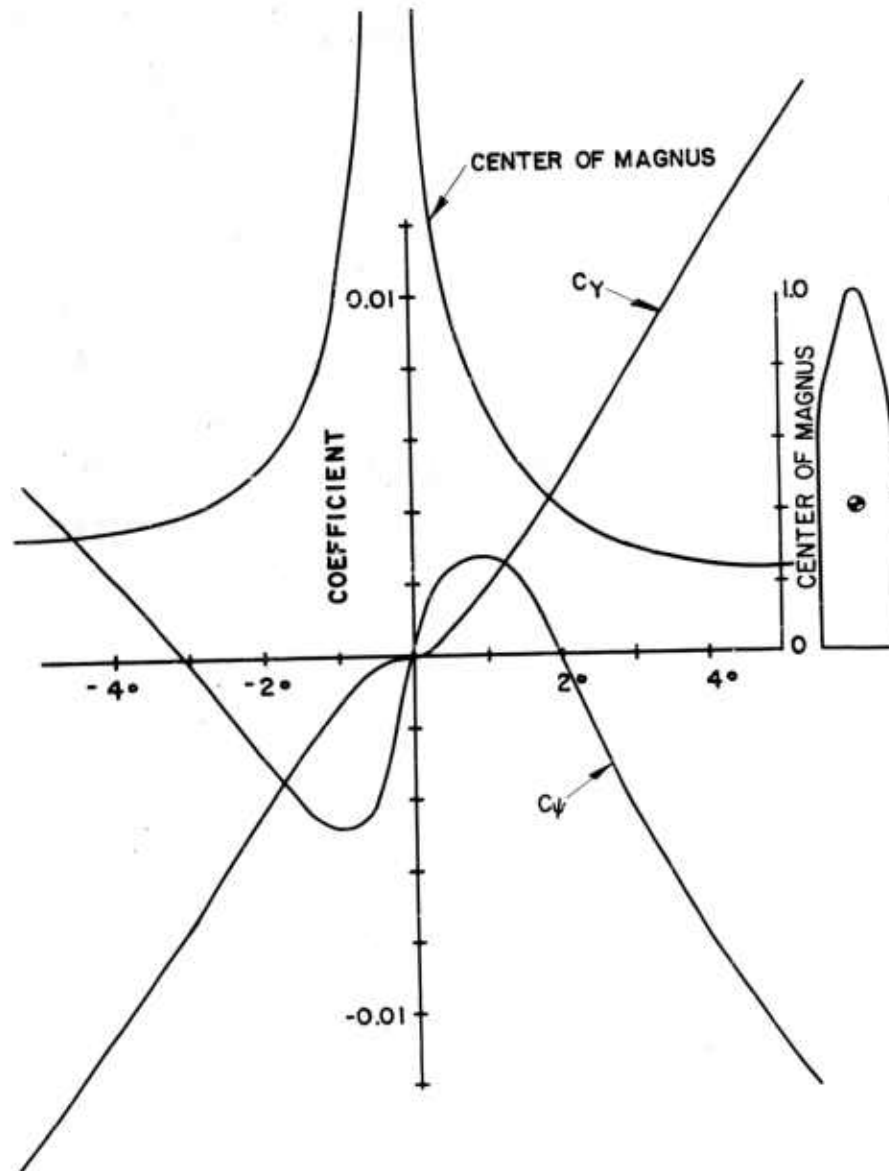
FIG. 53 C_Y , C_\Psi , AND CENTER OF MAGNUS VS \alpha_1 FOR THE TYPICAL PROJECTILE NOSE (P=309 RPS)
