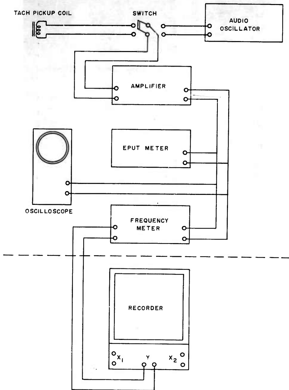
FIG. 8 DIAGRAMATIC SKETCH OF THE FREQUENCY CONSOLE
