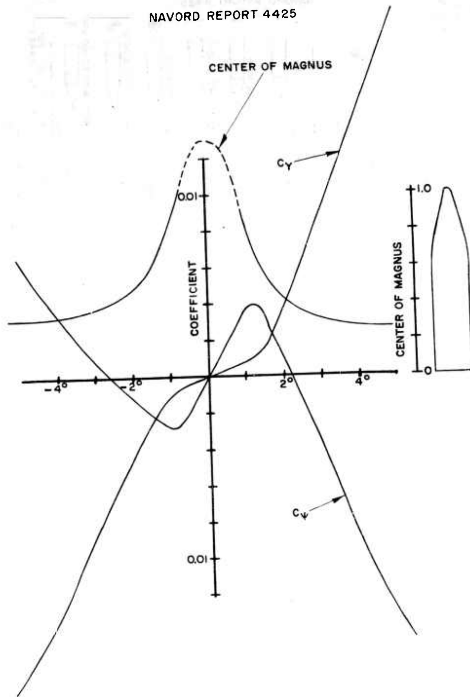
FIG. 55 C_Y , C_\Psi AND CENTER OF MAGNUS VS \alpha_1 FOR THE TYPICAL PROJECTILE NOSE P=468 RPS
