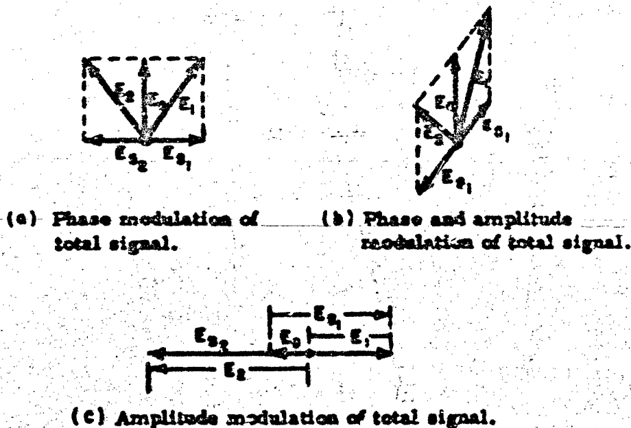
Fig. 2. Effect of relative phase of signal components on total back scattered signal.
