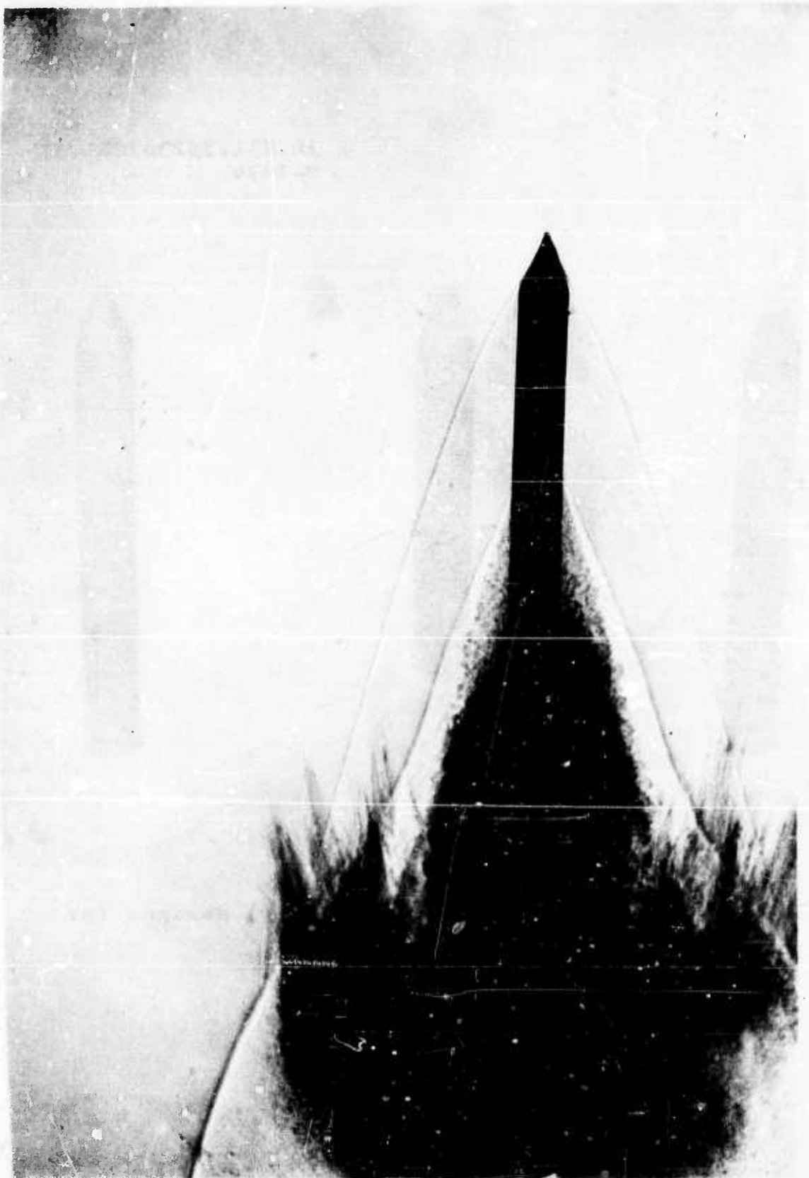
Figure 9. Shadowgraph of model 14 projectile fired at 4900 fps, showing turbulence
