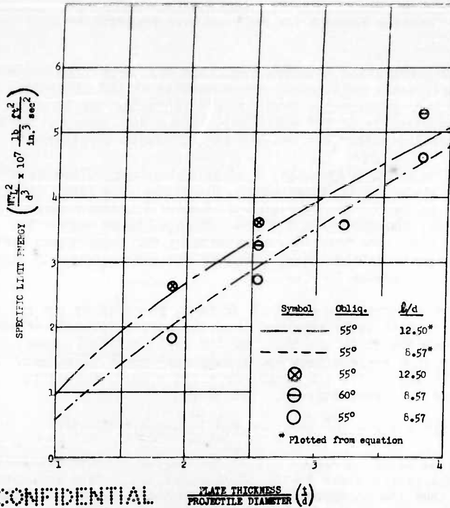
Figure 5. Perforation energy vs plate thickness for 40 mm (T82E16, E22, E23) arrow-type monobloc steel projectiles vs R4 armor at 55° and 60° obliquity
