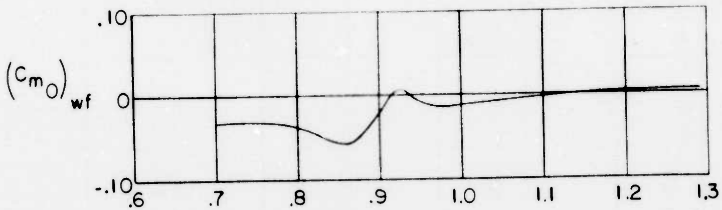
Fig.16 Variation of wing-fuselage parameters with Mach number. X-1 airplane
