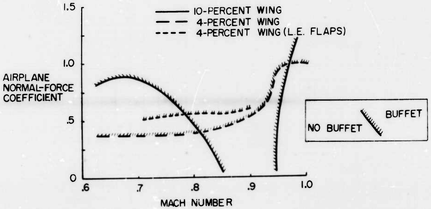
Fig. 19 Effects of airfoil thickness on buffeting
