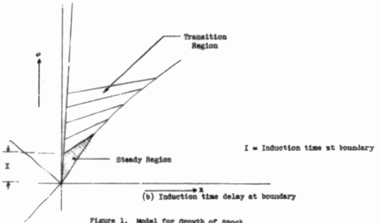
Figure 1. Model for Growth of Shock
