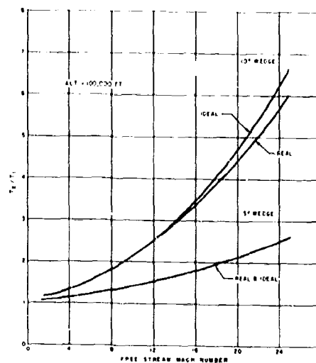
Figure 14. Static Temperature Ratio vs Mach Number
