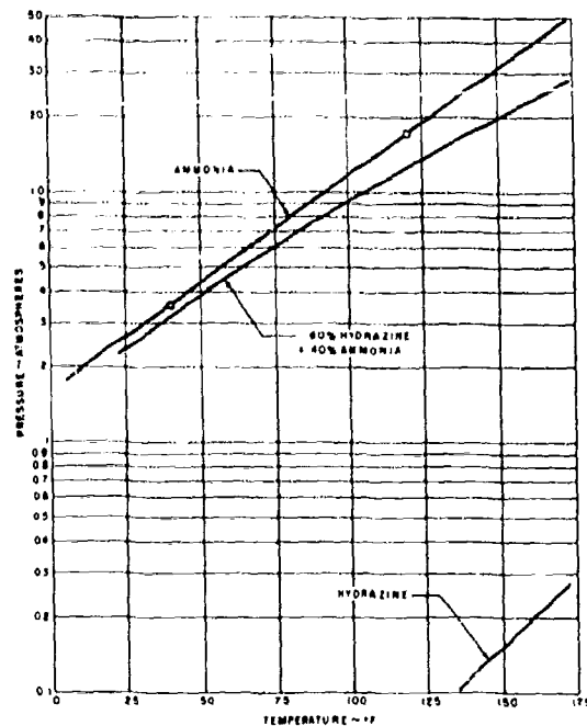
Figure 81. Vapor Pressure vs Temperature for Ammonia, Hydrazine, and Hydrazine-Ammonia Mixture
