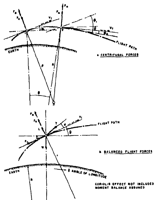
Figure 50. Flight Forces
