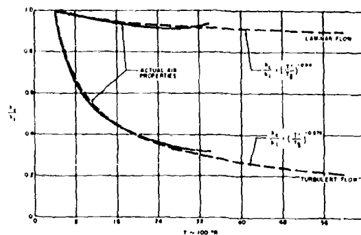
Figure 26. Heat Transfer Coefficient Correction Factor
