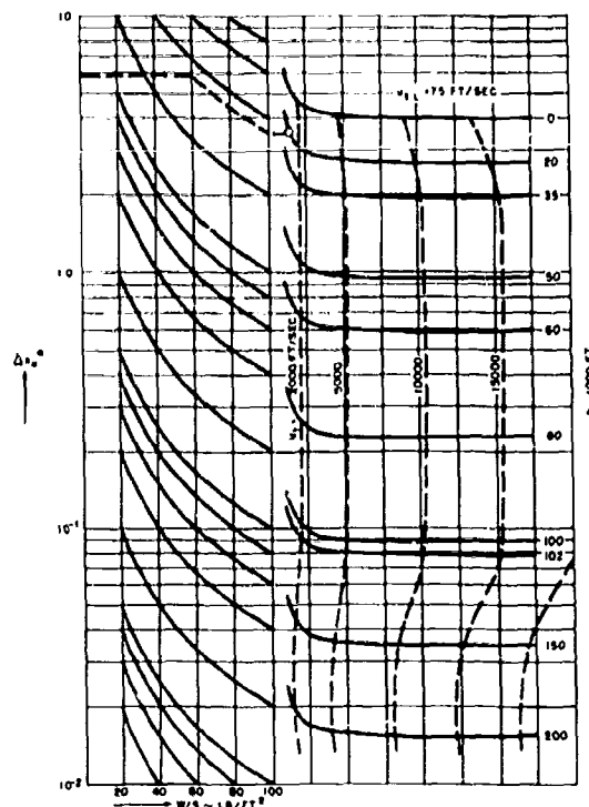
Figure 47. Gust Load Nomogram
