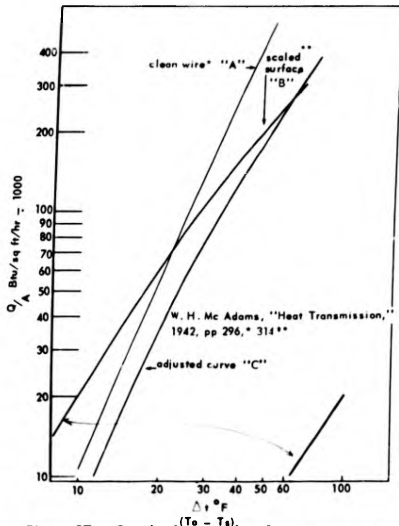
Figure 27. Graph of assumed surface temperature with boiling in engine.
