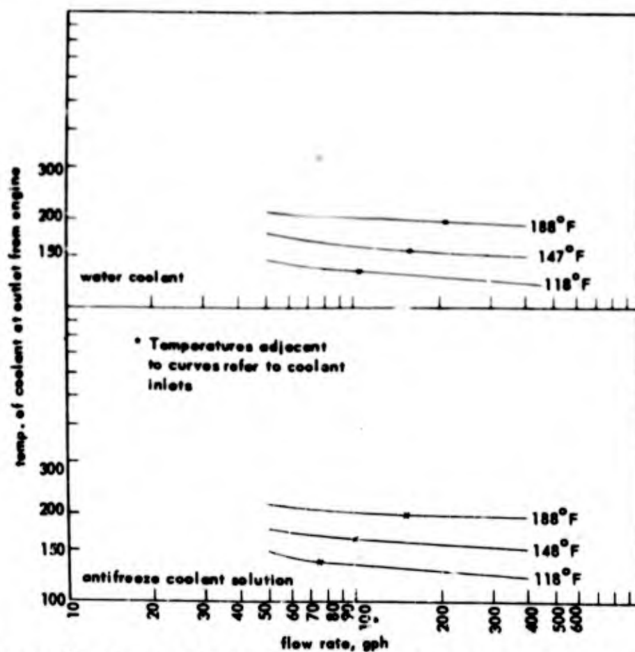
Figure 31. Graphs of data from Figure 25 replotted to log-log scale with approximate points of discontinuities.
