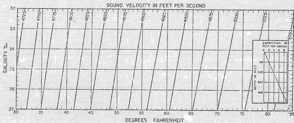
FIGURE 3. Effect of temperature, salinity, and pressure on the speed of sound in sea water.
