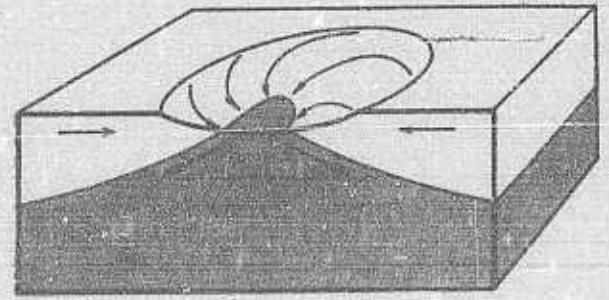
FIGURE 10. Diagram of water movements resulting from localized cooling of the sea surface.
