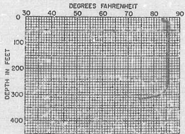
FIGURE 11. Bathythermogram showing positive temperature gradient at the surface due to rain.
