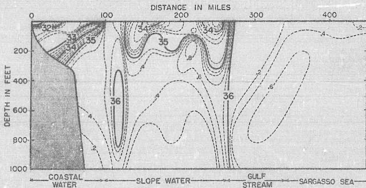
FIGURE 5. Salinity profile, Montauk Point to Bermuda.
