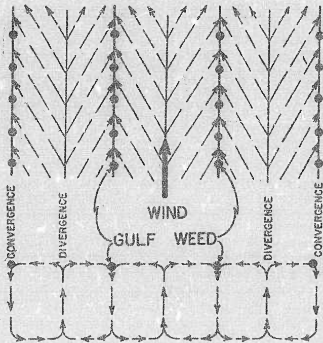
FIGURE 29. Diagrammatic representation of convection cells.
