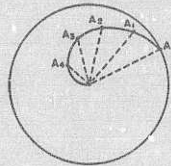
FIGURE 11. Movement of water into a cold center, showing direction of pressure and the resulting motion as modified by Coriolis force.
