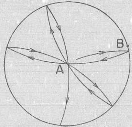
FIGURE 2. Diagram illustrating Coriolis force—apparent motion of a swinging pendulum on a rotating earth.
