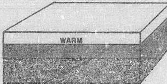
FIGURE 8. Equilibrium that results when movements shown in Figure 7 are carried to completion.
