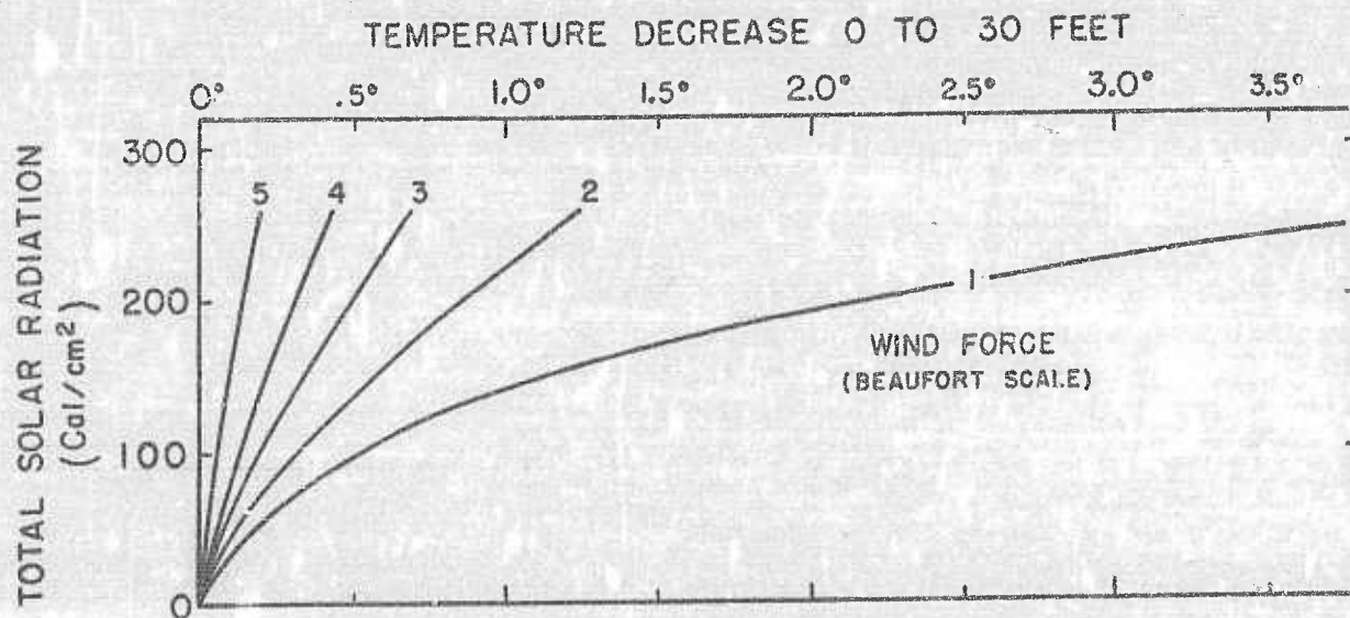
FIGURE 20. Effect of wind on diurnal warming.
