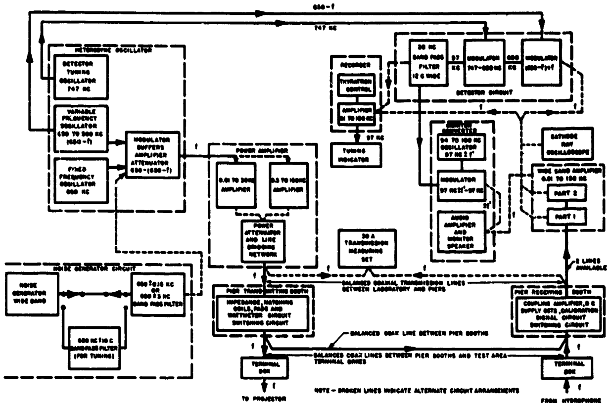
FIGURE 7. Block diagram of 15 c to 150 kc System 2.
