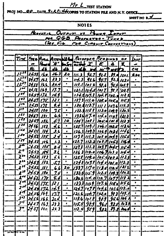
FIGURE 35. Typical data sheet, showing projector output versus electric power input.
