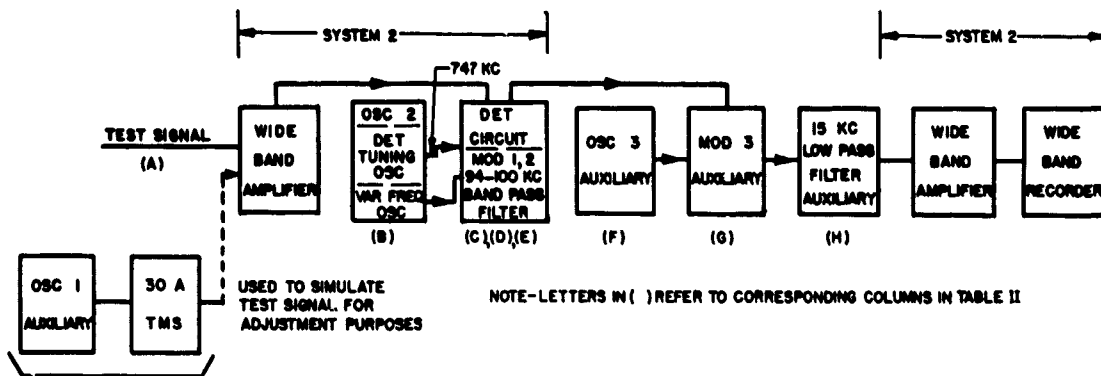
FIGURE 39. Simplified circuit arrangement using System 2 with auxiliary apparatus for obtaining a band-pass filter adjustable in width up to 6 kc and with a mid-band frequency variable between 3 and 150 kc.
