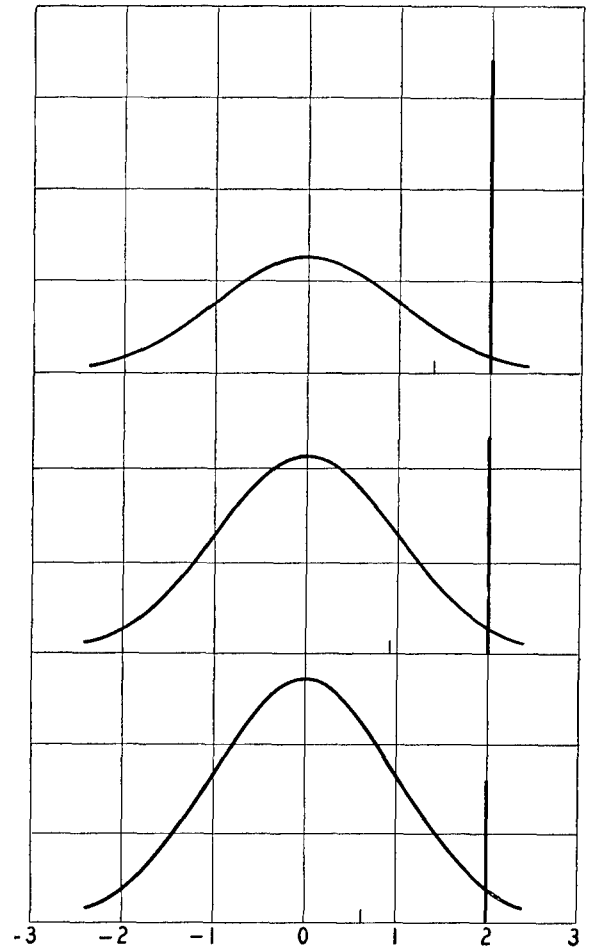
FIGURE 1. Probability distribution of future position of target, assuming piecewise analytic courses.
