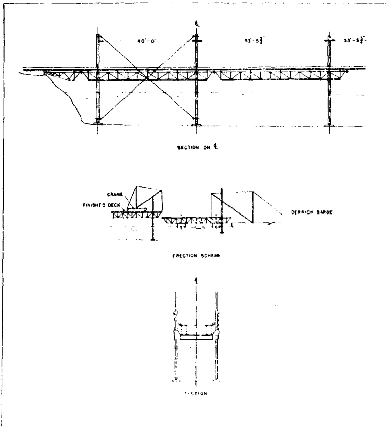
FIGURE 2. Design of London pier.
