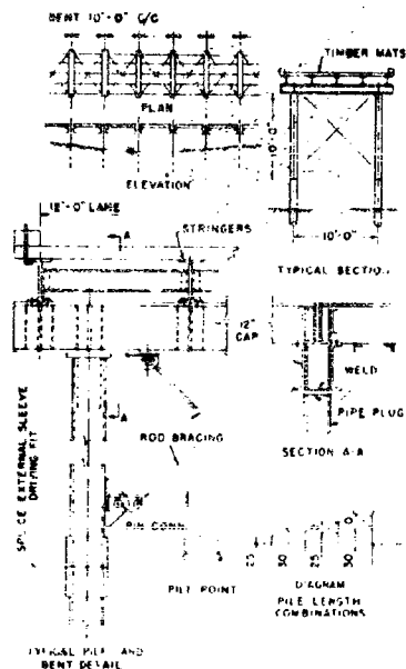
FIGURE 13. Design of temporary highway trestle steel pipe construction.
