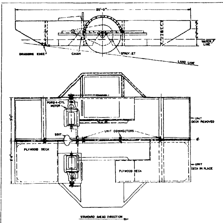
FIGURE 21 Amphibious ponton (wheel) boat, plan I.
