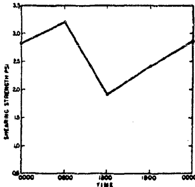
FIGURE 10. Typical "chert cool spring to summer day" changes in shearing strength of snow over 24-hour period.
