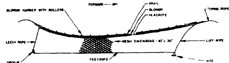
FIGURE 1. General arrangement of torpedo net defense (NSD) on a ship. This type is designed to catch up to 35-knot torpedoes moving at speeds above 5 knots to be effective, and is able to catch torpedoes only by the tail.
