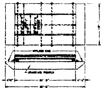
FIGURE 7. Ponton modified with molded ends to serve as 30-ton tank ferry.
