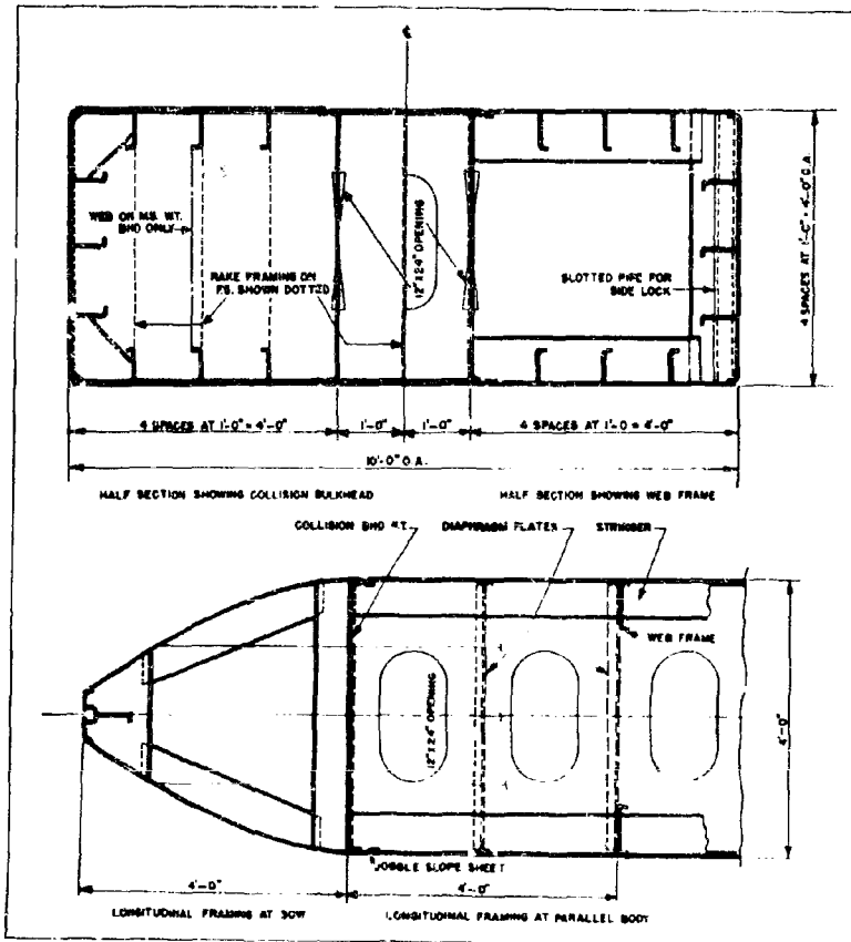
FIGURE 18. Plan and side elevation of pontoon for 10-ton tank ferries.
