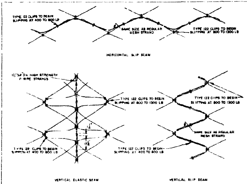
FIGURE 9. Diagrams of horizontal and vertical seams.
