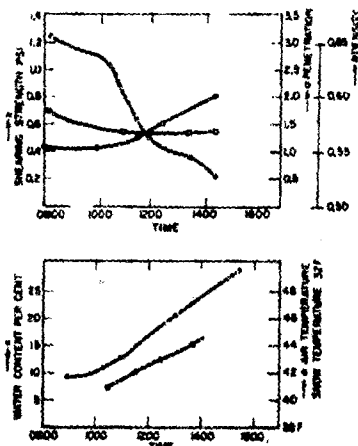
FIGURE 3. Changes in shearing strength, penetration, density, water content, and air temperature (snow temperature = 32 F) from about 0800 to 1600 hours on bright sun, shiny day with no winds or clouds, August 5, 1942, on Saskatchewan Glacier.
