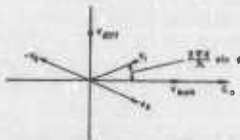
FIGURE 24. Vector diagram of doublet voltages.
