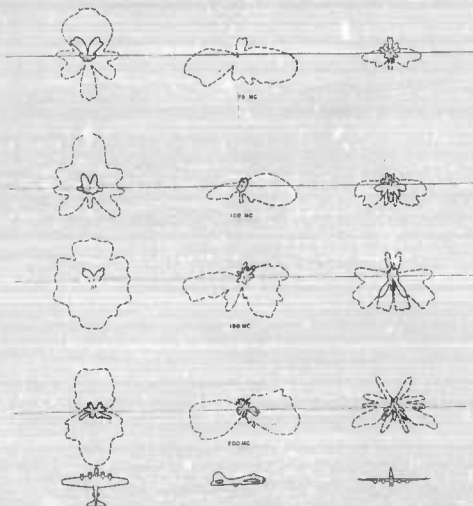
FIGURE 3. Antenna patterns of a 4 stub on belly of B-17F directly in front of bomb bays. Dotted lines indicate vertical polarization, E_v ; full lines indicate horizontal polarization, E_h .
