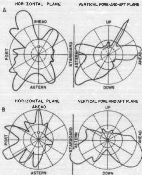
Figure 3. Antenna pattern versus location: 1/4 inch at 100 m; located as follows: A, wing of vertical stabilizer; B, wing tip; 100 m not from centerline of ship.
