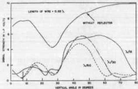
FIGURE 7. Vertical response characteristics of 1/2 dipole with 90° corner reflector with different spacings between reflector wires.
