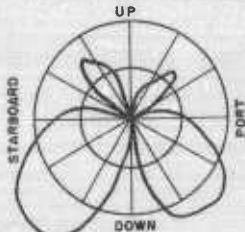
FIGURE 11. Effect of loading 40- to 60-mc antenna in same location as an antenna for 50 to 40 mc. Same antenna, overall length 8.25 ft, sleeve length 2.125 ft, 40 mc; vertical polarization; location forward along fuselage on centerline 11.5 ft forward of leading edge of horizontal stabilizer on B-36.
