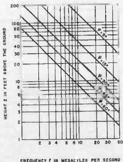
FIGURE 6. Maximum height above perfect ground at which |E_{\theta}/E_{\phi}| = |E_{\theta d}/E_{\phi d}| .
