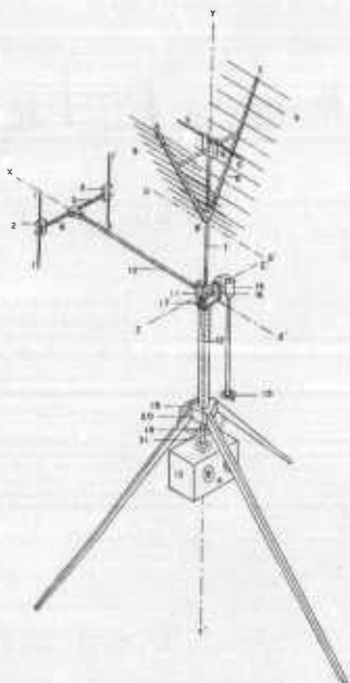
FIGURE 1. Sketch of d-f instrument.
