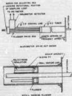
FIGURE 20. Measuring equipment used in experiment. L = 150 CM. (60 CM).
