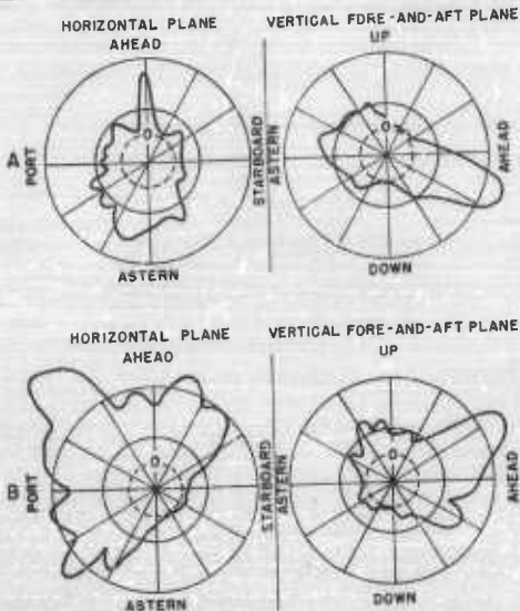
FIGURE 10. Antenna patterns versus location: \lambda/4 dipole at 100 mts located as follows: A, underside hull below tail; 100 mts forward of tip of tail; B, reverse of A.
