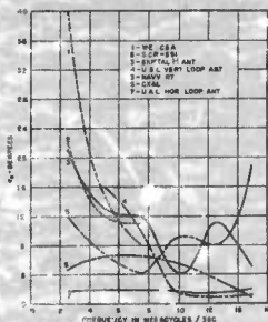
FIGURE 12. \epsilon_{45} versus frequency for direction finders tested.
