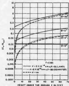
FIGURE 4. Ratio of resultant horizontal to vertical electric field components when plane wave with equal parallel and normal components is incident on ground at angle of elevation \psi .
