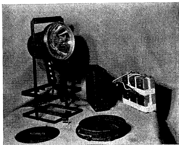
FIGURE 5. Gallium lamp portable assembly. Upper —Assembled, complete with batteries and carrying stand. Lamp and one battery when removed form one complete unit for code communication. Spare battery is for prolonged operation. Lower —Disassembled unit showing component parts.
