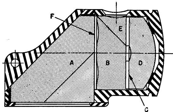
FIGURE 12. Assembly of Type L; A , roof prism; B , front element; C , separator plate; D , back element; E , eyepiece segment; F , red filter.
