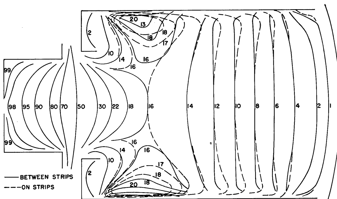
FIGURE 18. Potential distribution of the single-voltage image tube (U-41).
