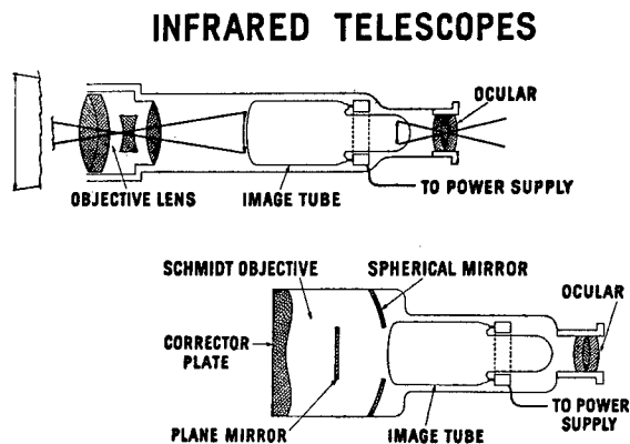
FIGURE 1. Two forms of the infrared telescope, one employing a refracting objective and the other a Schmidt system.
