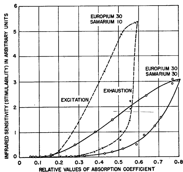
FIGURE 11. Sensitivity against absorption during excitation and exhaustion.
