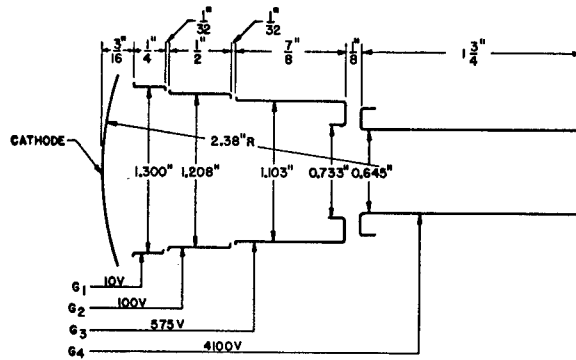
1P25 ELECTRODE DIMENSIONS AND VOLTAGES
