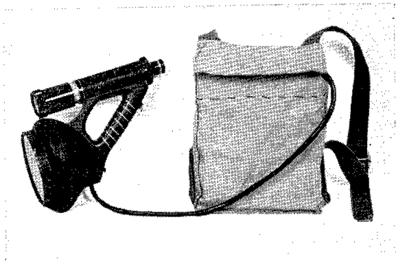
FIGURE 39. The snooperoscope.
