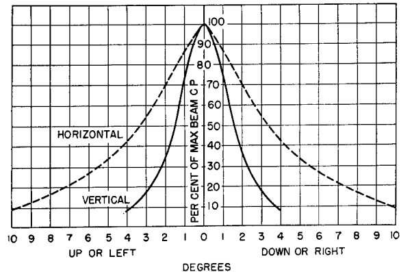
FIGURE 36. Percentage candlepower distribution for the 7-inch 400-watt A-H10 mercury lamp, maximum candlepower 600,000.
