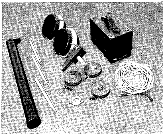
FIGURE 13. Components of airborne beacon, including collapsible mast, stakes, gey wires, and twin sources.
