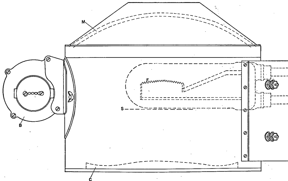
FIGURE 3. The optical system of the K-S projector.
