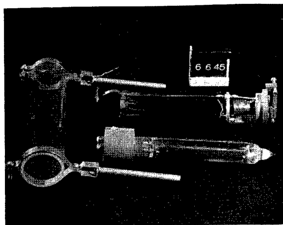
FIGURE 3. Gallium lamp. Upper —Discharge tube assembly. Lower —Disassembled unit showing discharge tube, thermostat and jacket.
