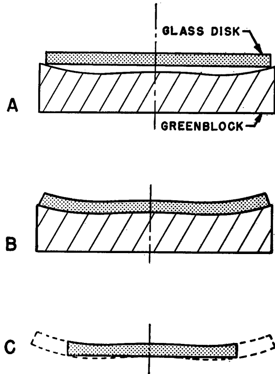
FIGURE 16. A. Sectional view of mold and blank before heating. B. Appearance after temperature cycle. C. Finished plate edged to diameter, lower surface ground and polished flat.
