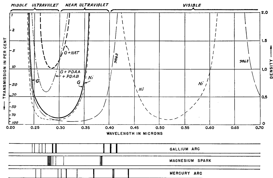
FIGURE 14. Density and transmission curves for G-filter alone, components of G-filter, and G-filter plus NAT filter. Spectra of sources to show radiation in ultraviolet region.
