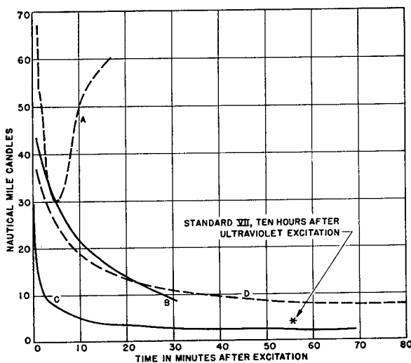
FIGURE 5. Threshold sensitivities of various phosphors in Type A metascope. A. Early sample of Standard VII. B. Standard VII, ultraviolet-excited. C. Standard VII, radium-excited. D. B-1.
