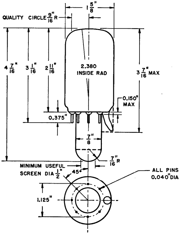
FIGURE 12. Glass envelope of the 1P25 image tube.
