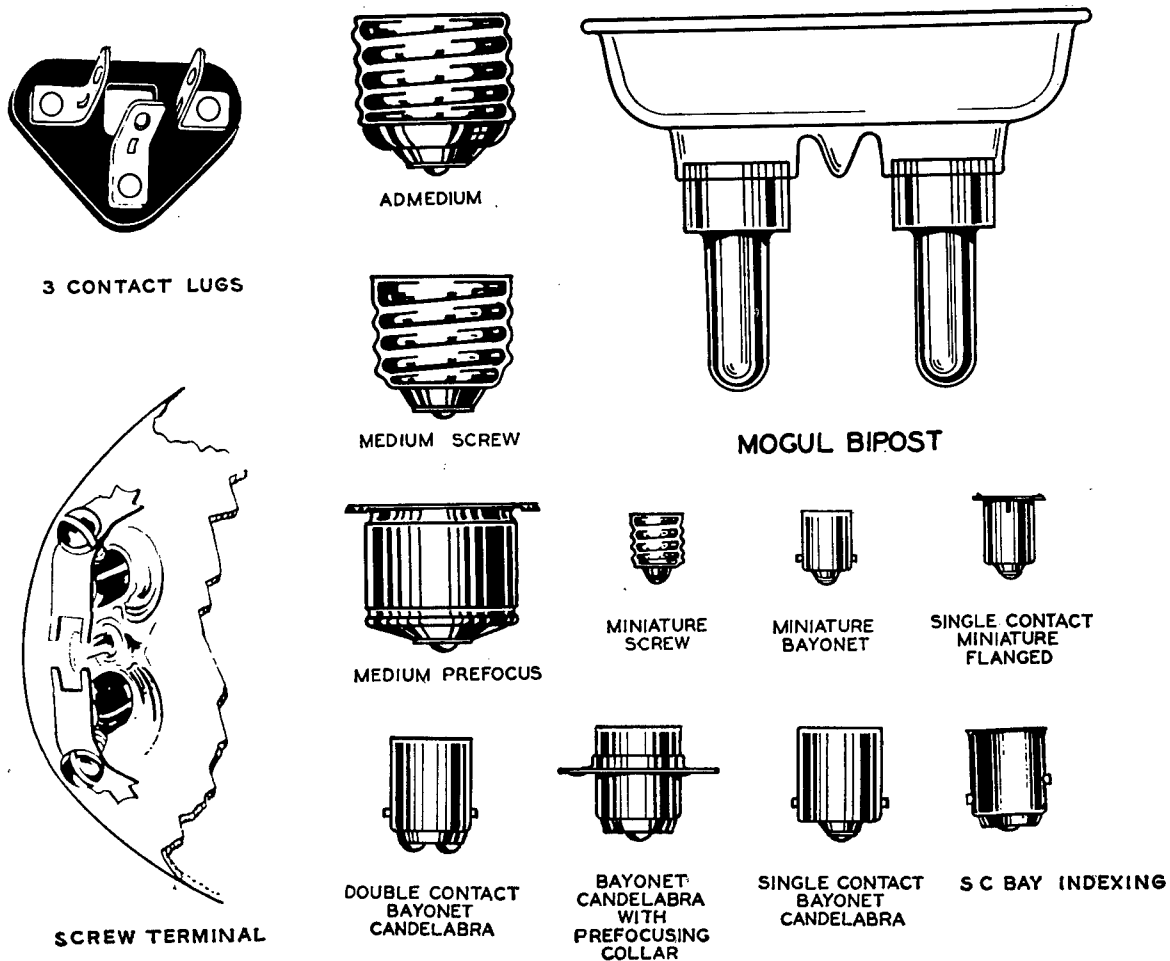
FIGURE 2. Bases used on incandescent and conventional mercury lamps described in this chapter.
