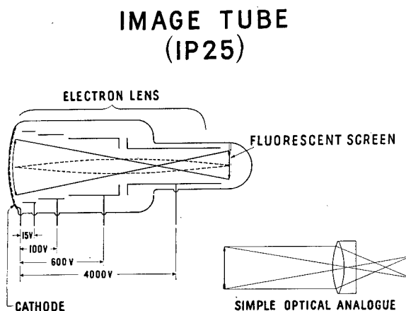
FIGURE 2. Schematic diagram of the standardized image tube.
