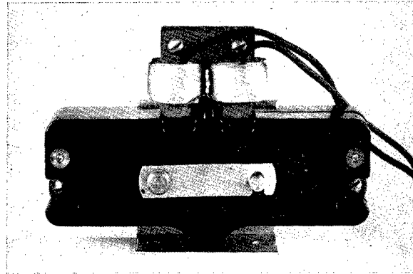
FIGURE 32. The Z-12146 magnetic starter used for the A-H10 and B-H10 mercury lamps.
