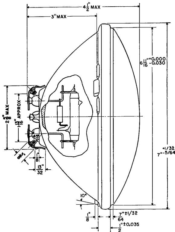
FIGURE 31. Construction details of the 100-watt J-H4 mercury lamp.
