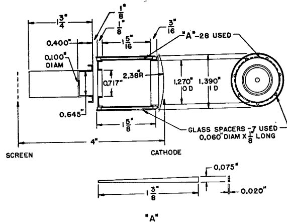
UNPOTENTIAL IMAGE TUBE-ELECTRODE ARRANGEMENT AND DIMENSIONS
