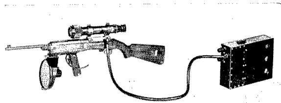
FIGURE 40. The sniperscope.
