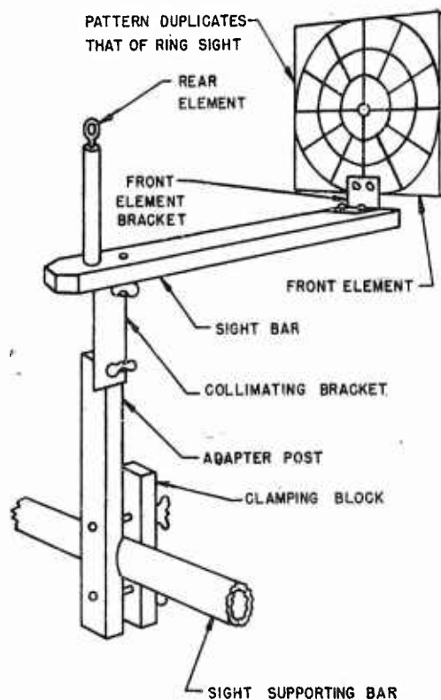
FIGURE 5. Plexiglas checksight.
