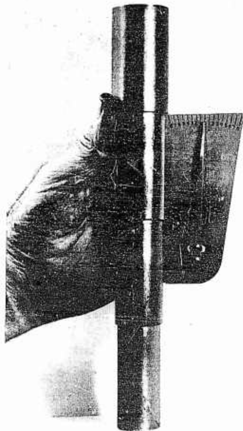
FIGURE 4. A caliper gauge in use. The accuracy of the spacing between shoulders on the sampler is being measured.
