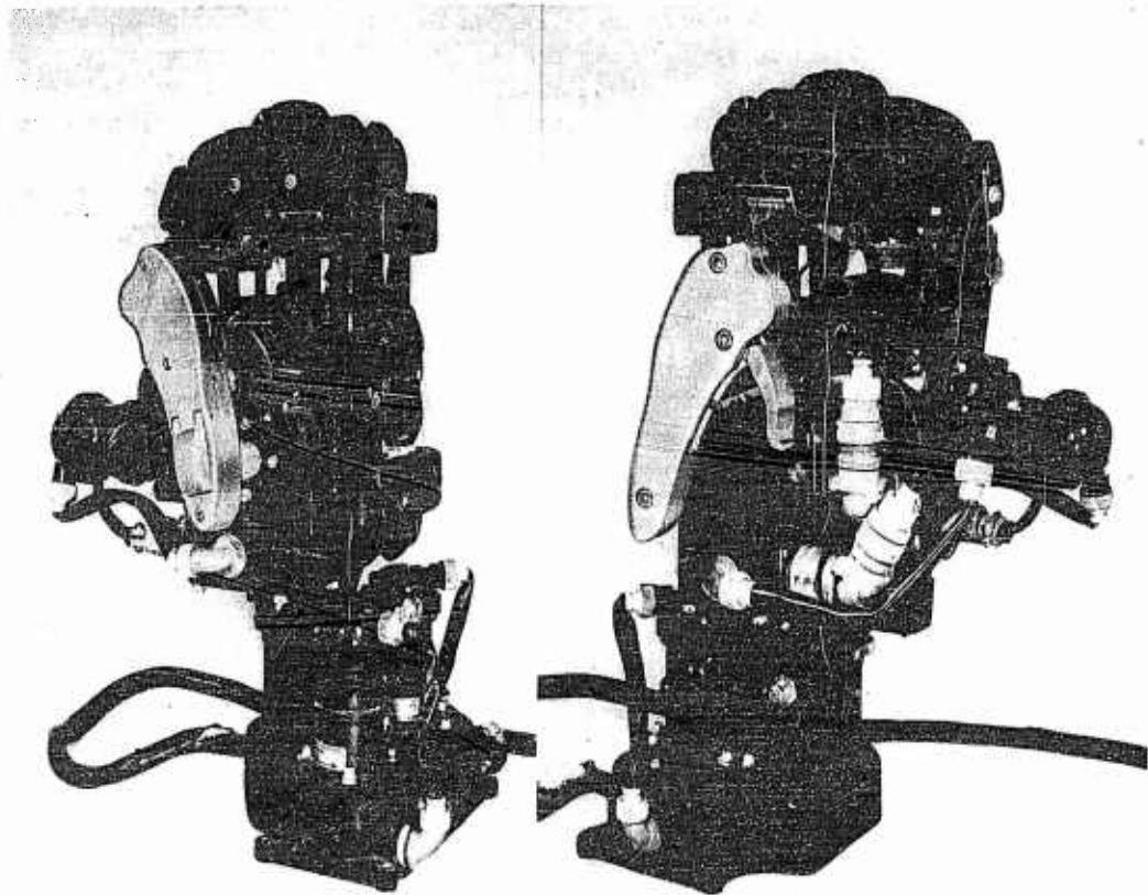
FIGURE 5. Modified B-29 gunsight controls. The left figure shows the left handgrip on which the trigger and action switch are mounted. The right figure shows the right handgrip on which a pressure-type ranging control is mounted. Both handgrips control azimuth and elevation tracking.
