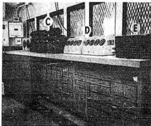
FIGURE 9. Interior of recording truck, right bench. C sound scribers; D panoramic telescope indicators; E electric cable junction box.
