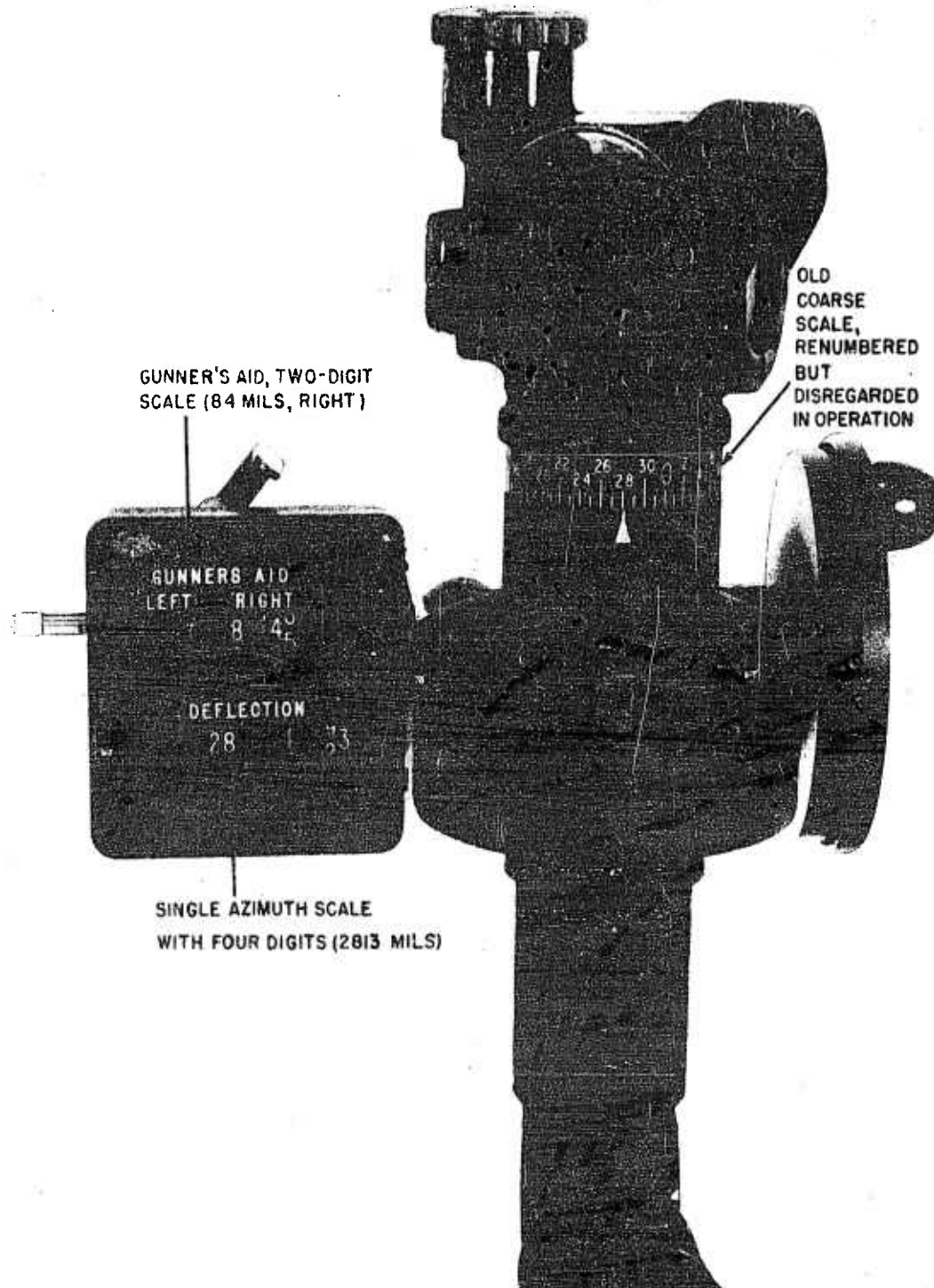
FIGURE 5. Panoramic telescope M-12 (T-138).
