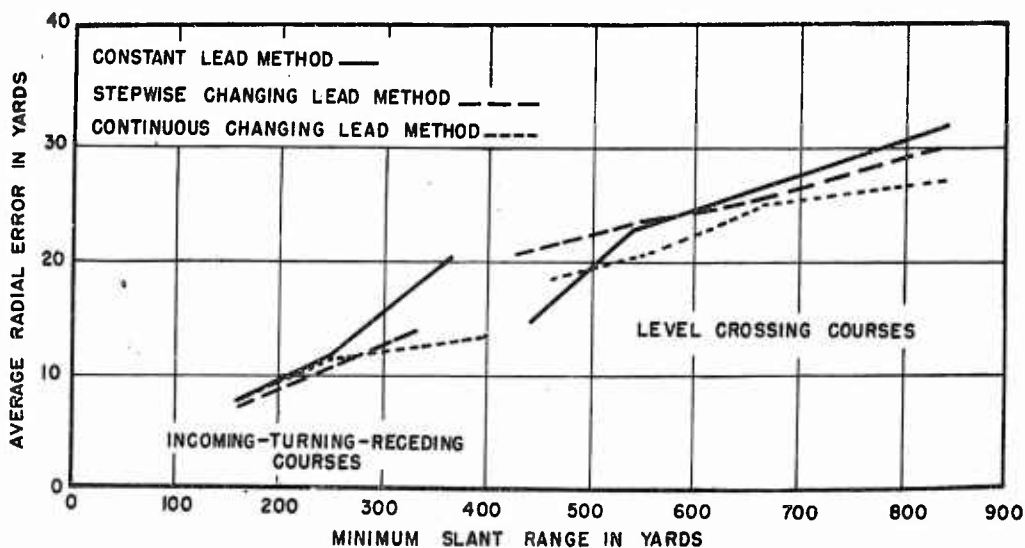
FIGURE 9. Effect of minimum slant range upon average radial firing error: A comparison of three speed ring methods for 40 mm operation.
