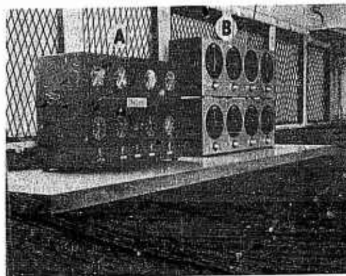
FIGURE 8. Interior of recording truck, left bench. A Range quadrant indicators; B tube position indicators.
