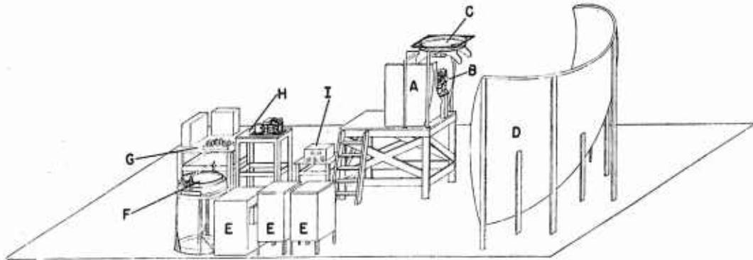
FIGURE 2. The remotely controlled test device.
