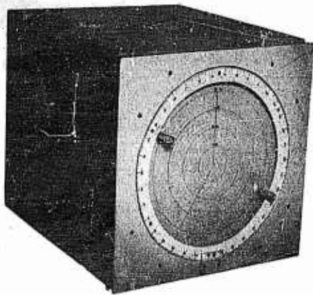
FIGURE 2. Mechanical PPI tracking trainer, scope face.
