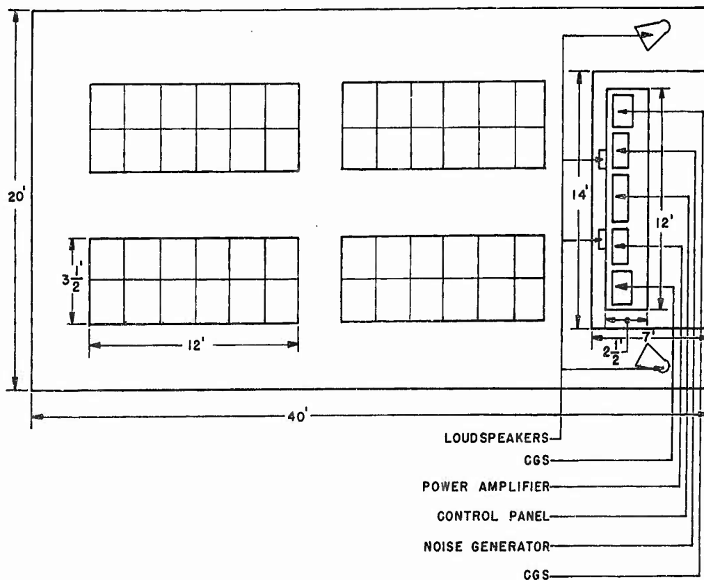
FIGURE 1. Diagram of recommended classroom.
