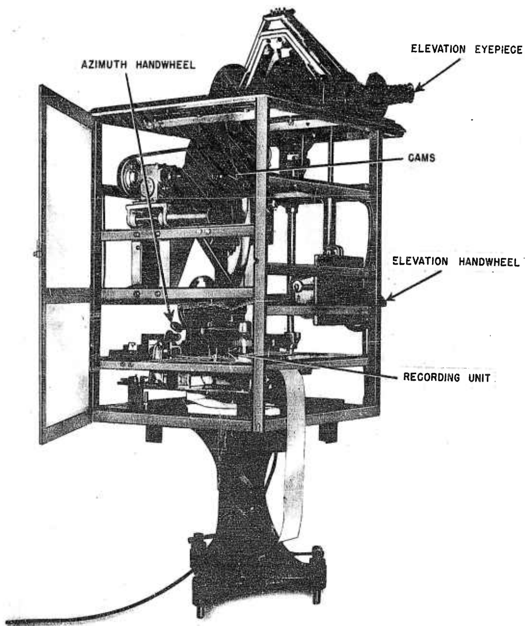
FIGURE 15. Tufts tracking trainer with housing removed, front view.
