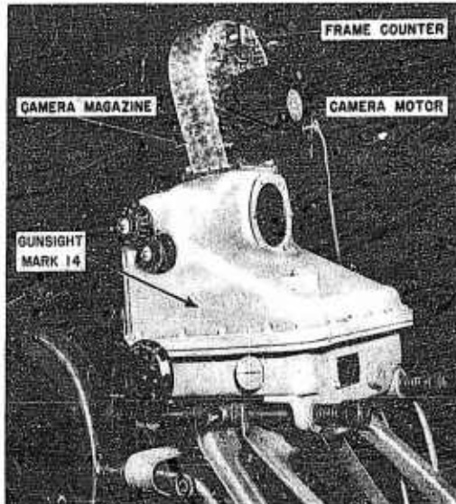
FIGURE 1. Gunsight Mark 14 with camera attached, front view.
