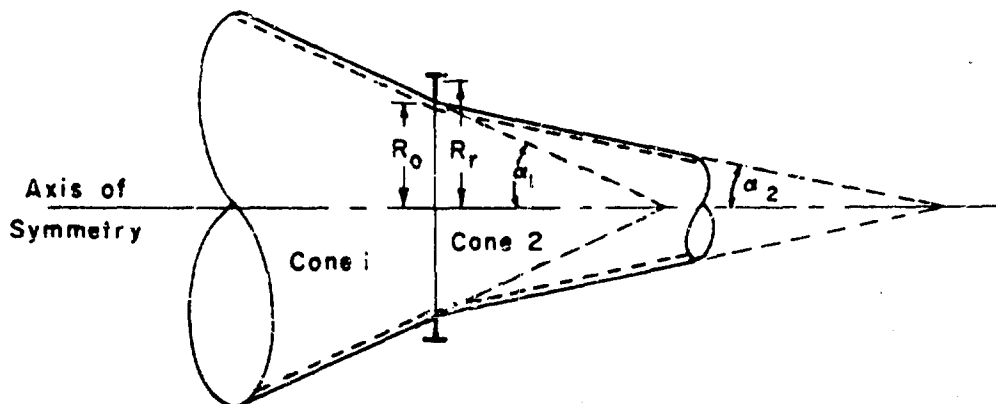
Figure 5 - Reinforced Cone-Cone Junction
