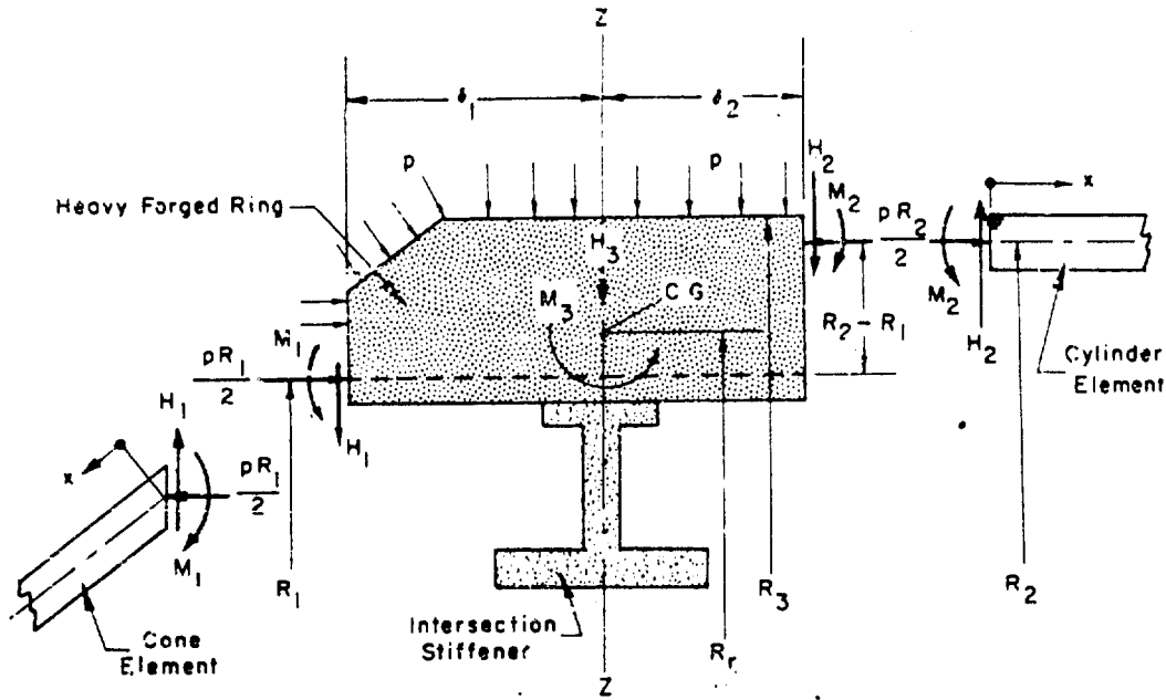
Figure 6 - Notation for Reinforcement at Cone-Cylinder Juncture
