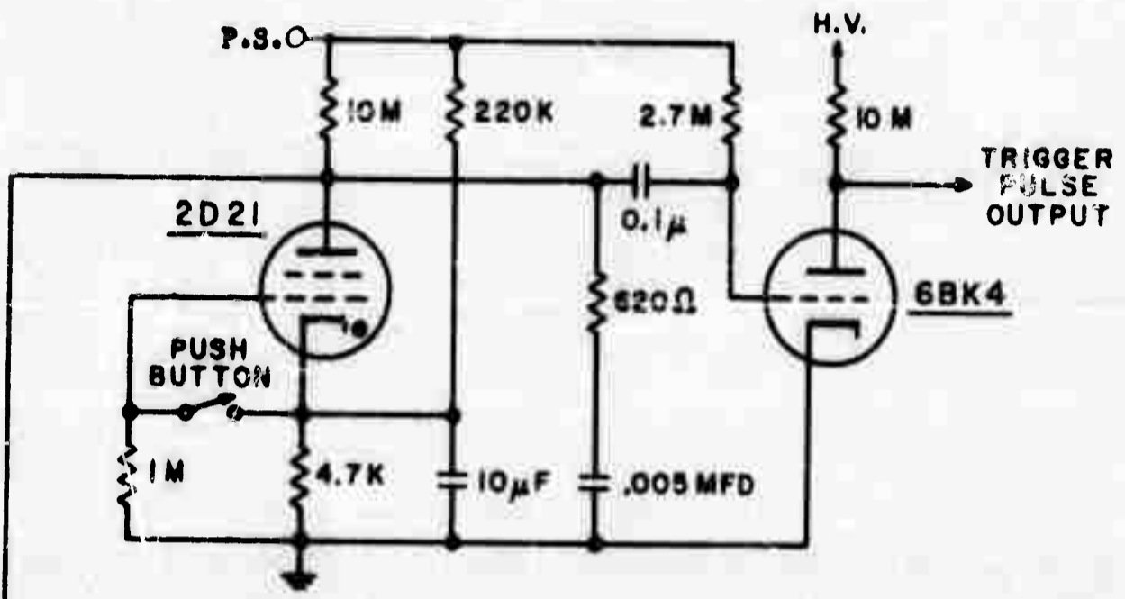
TRIGGER CIRCUIT
