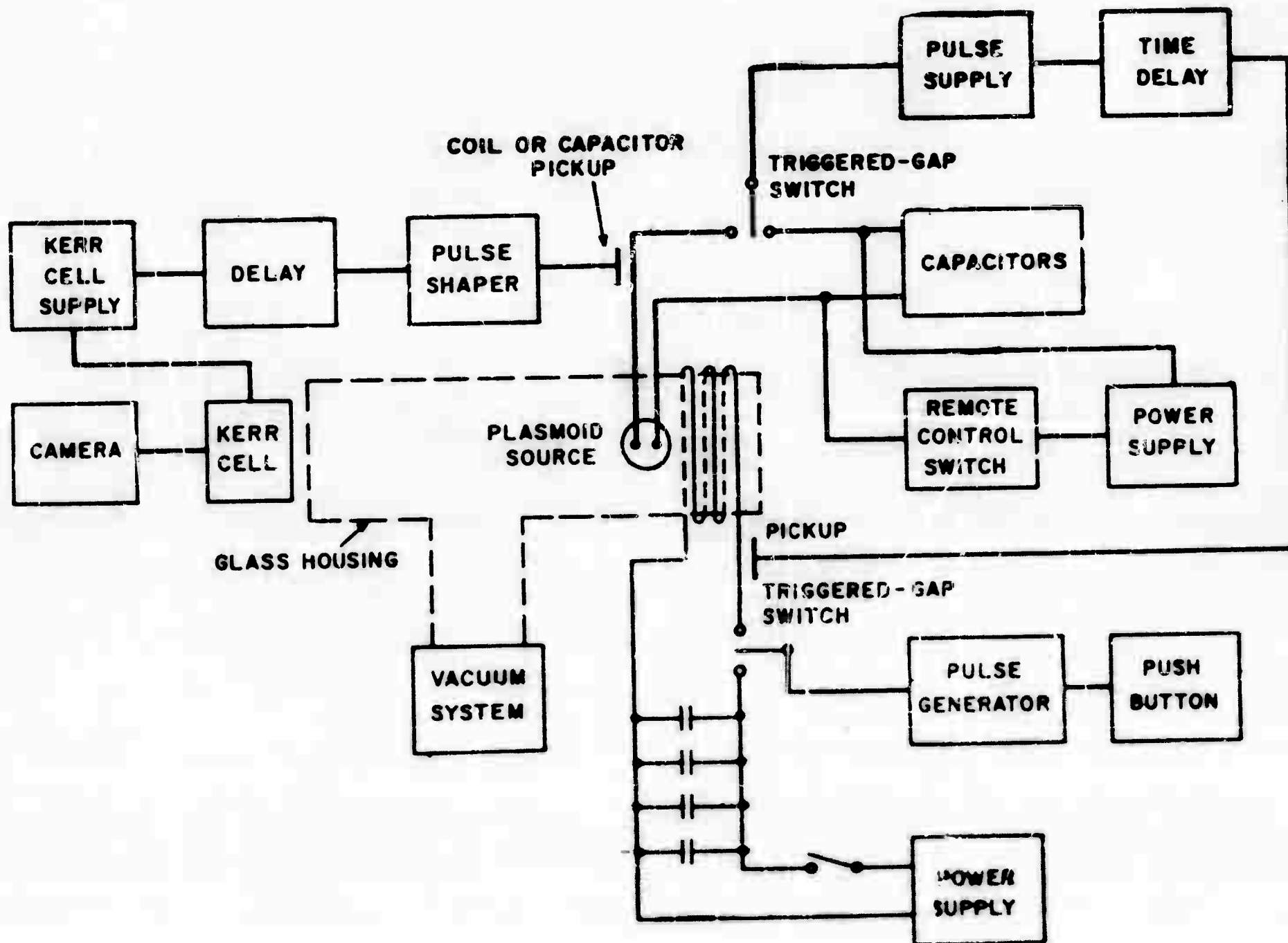
Figure 1. Block Diagram of Over-All Experimental System.
