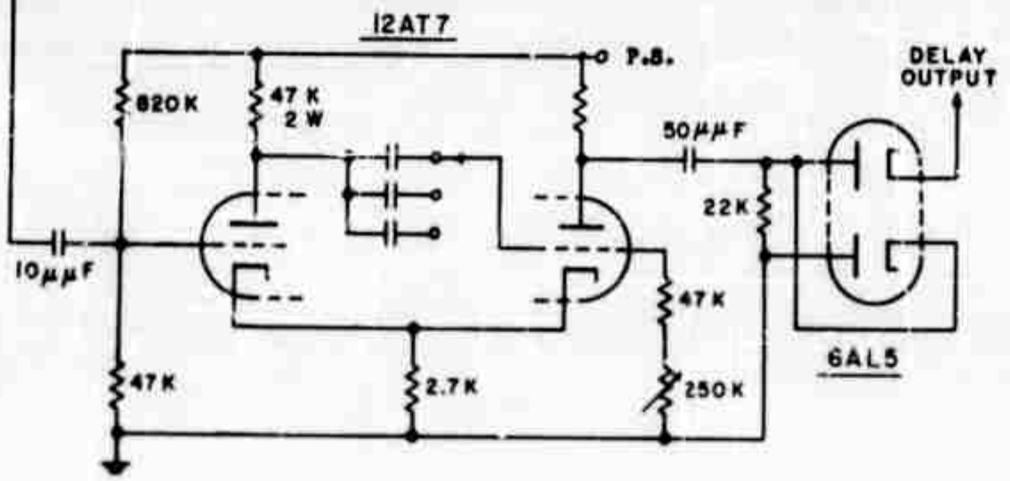
TIME DELAY
