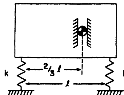
Figure 1-7. Systems with Coupled Natural Frequencies
