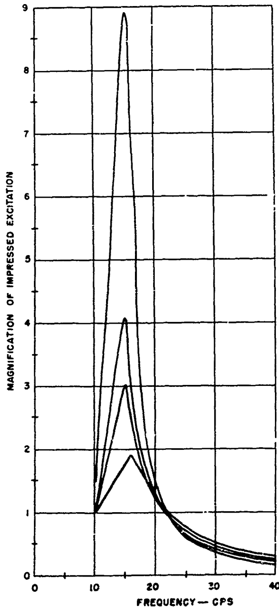
Figure 5-7. Typical Transmissibility Curves for a Vibration Isolator With and Without Friction Dampers
