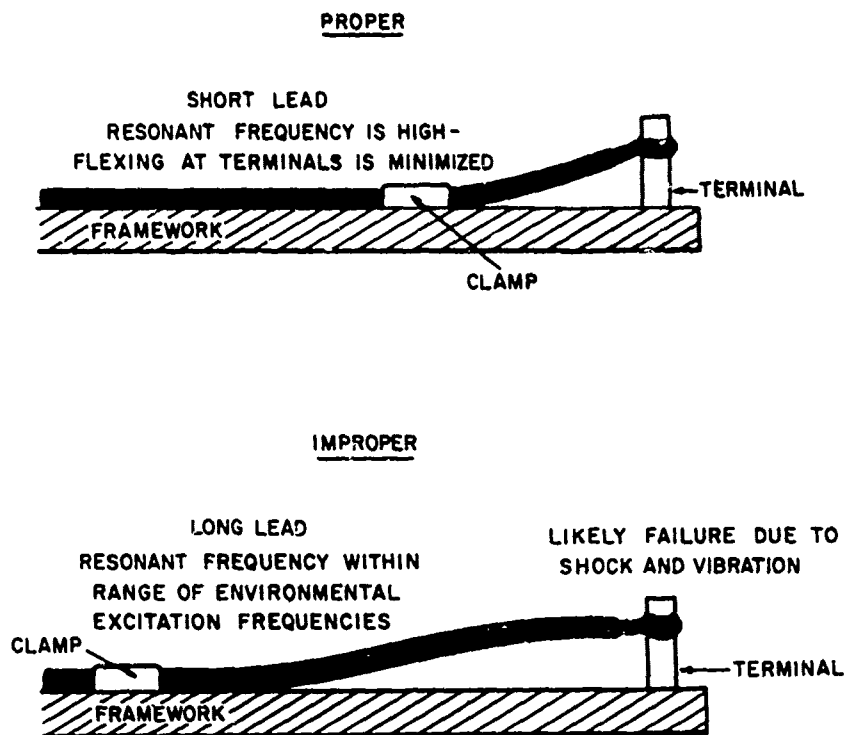
Figure 3-3. Proper Clamping of Cable End
