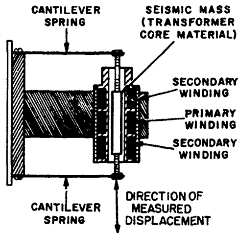
Figure 6-17. Cross Section of Differential-Transformer-Type Displacement Pickup
