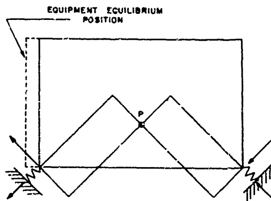
Figure 9-20. Inclined-Isolator Mounting System
