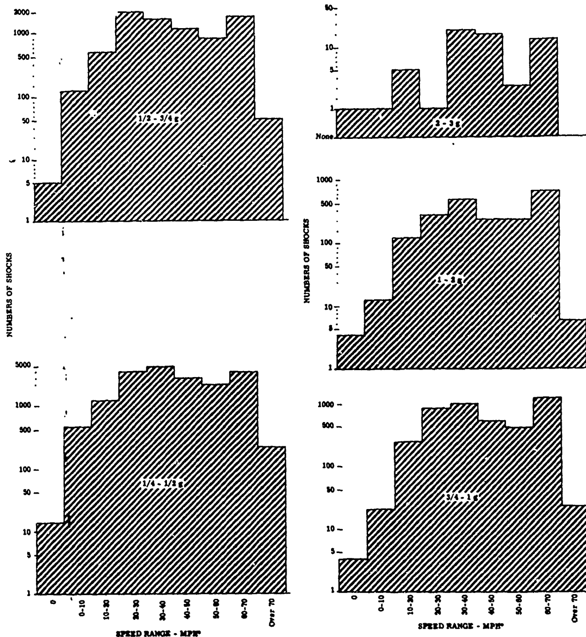
Figure 2-16. Vertical Shocks Measured on Freight Car Floor
