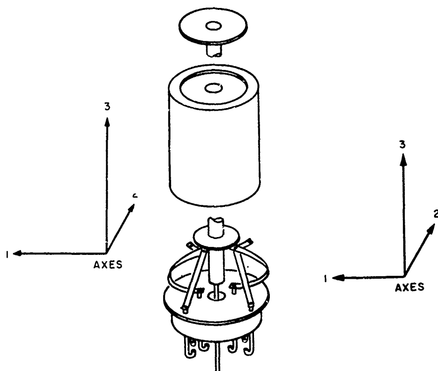
Figure 3-8. Rotary-Type Relay
