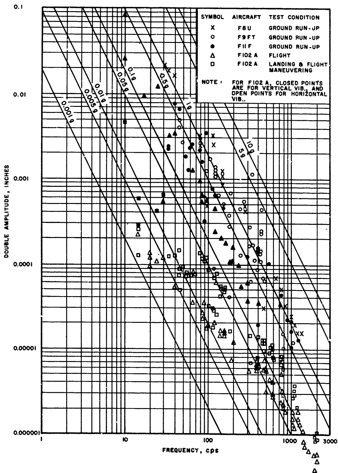
Figure 2-1. Vibration Data for Jet-Engine Fighter Aircraft
