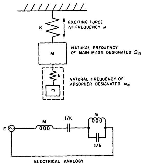
Figure 5-11. Dynamic Vibration Absorber
