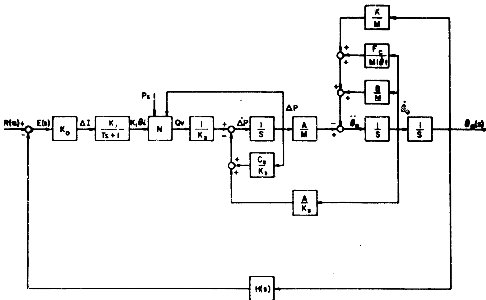
Figure 34. Block Diagram of Over-all System
