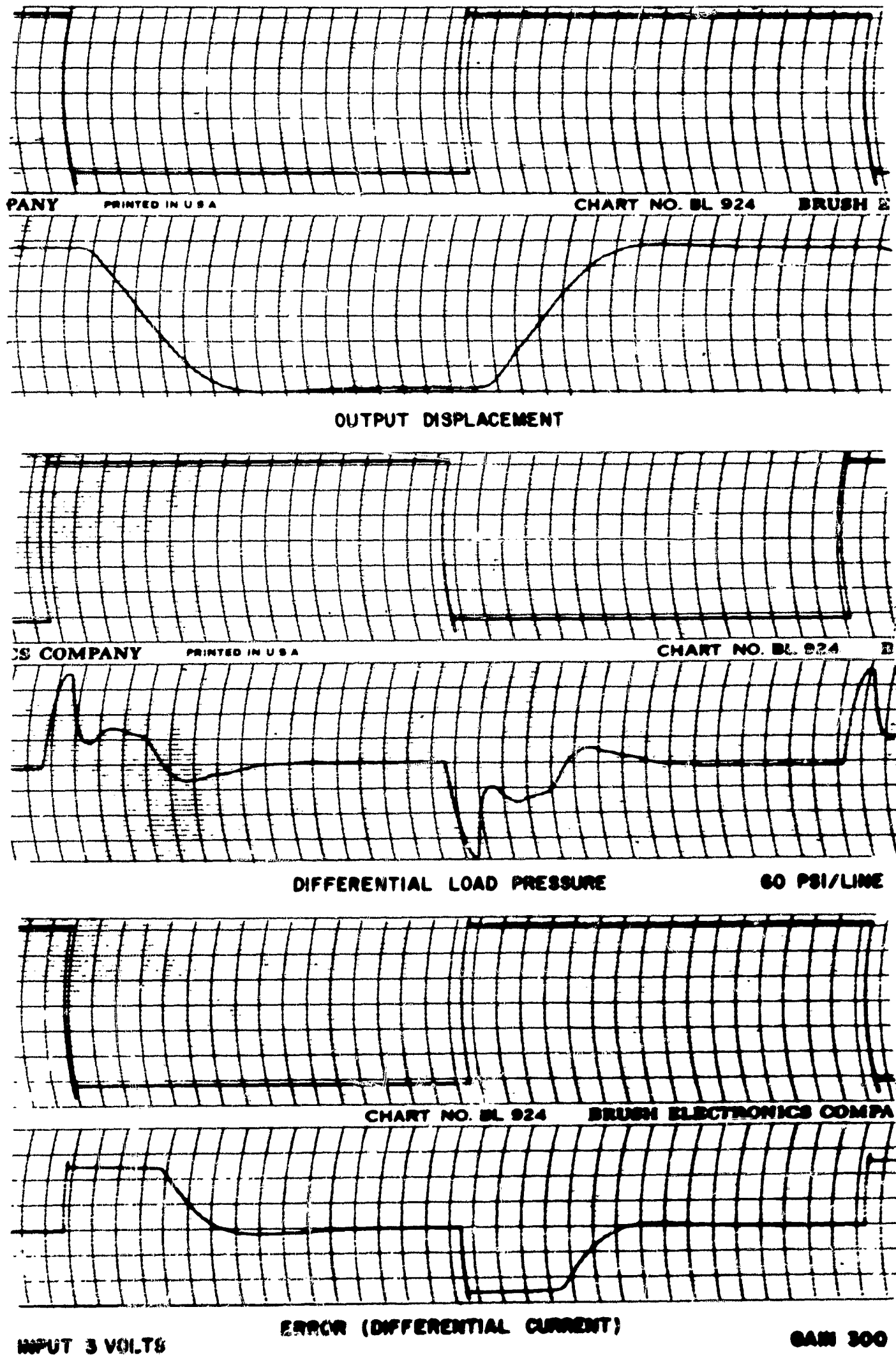
Figure 49. Transient Response of Analog System - FC-2 - 3.0 Input
