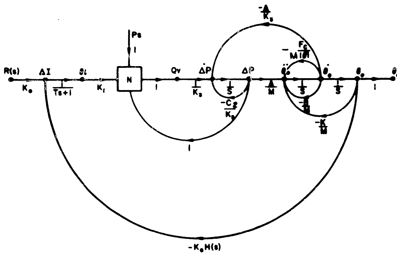
Figure 33. Signal Flow Graph of Over-all System
