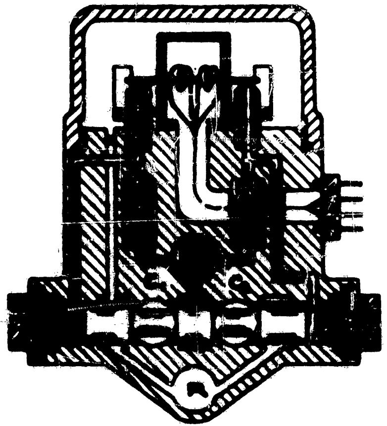
Figure 55. Schematic of Bendix Pacific HR-9 Valve
