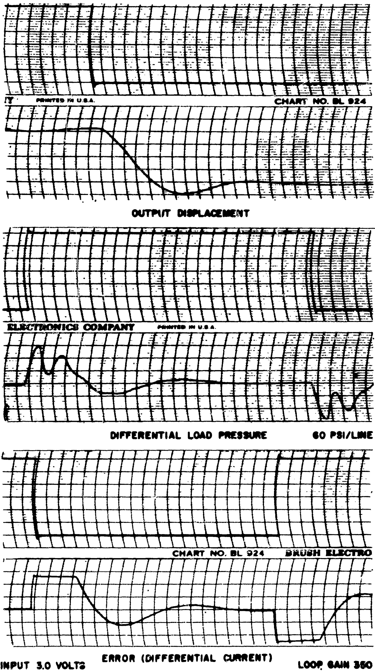
Figure 45. Transient Response of Analog System - 1402C - 3.0 Input
