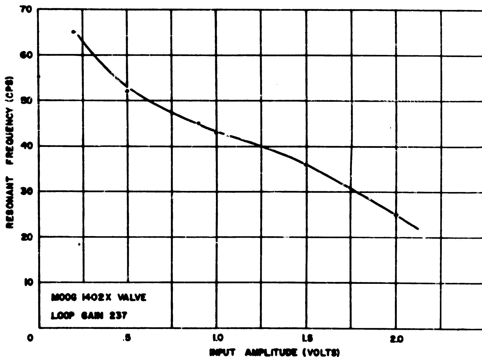
Figure 20. Moog 1402X Resonant Frequency vs. Input Amplitude
