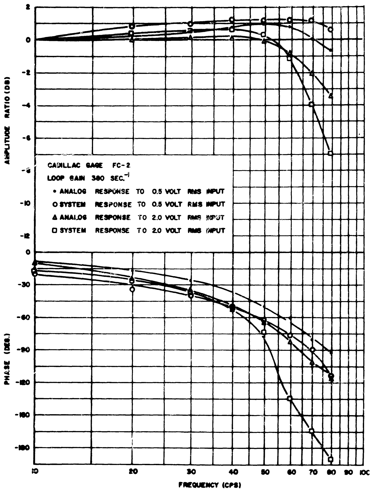
Figure 40. Closed-Loop Frequency Response of Analog and Reference Systems - FC-2 - 0.5 and 2.0 Input
