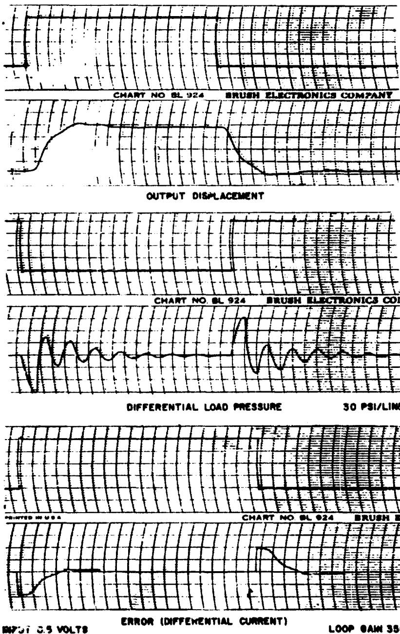
Figure 42. Transient Response of Analog System - 1402C - 0.5 Input
