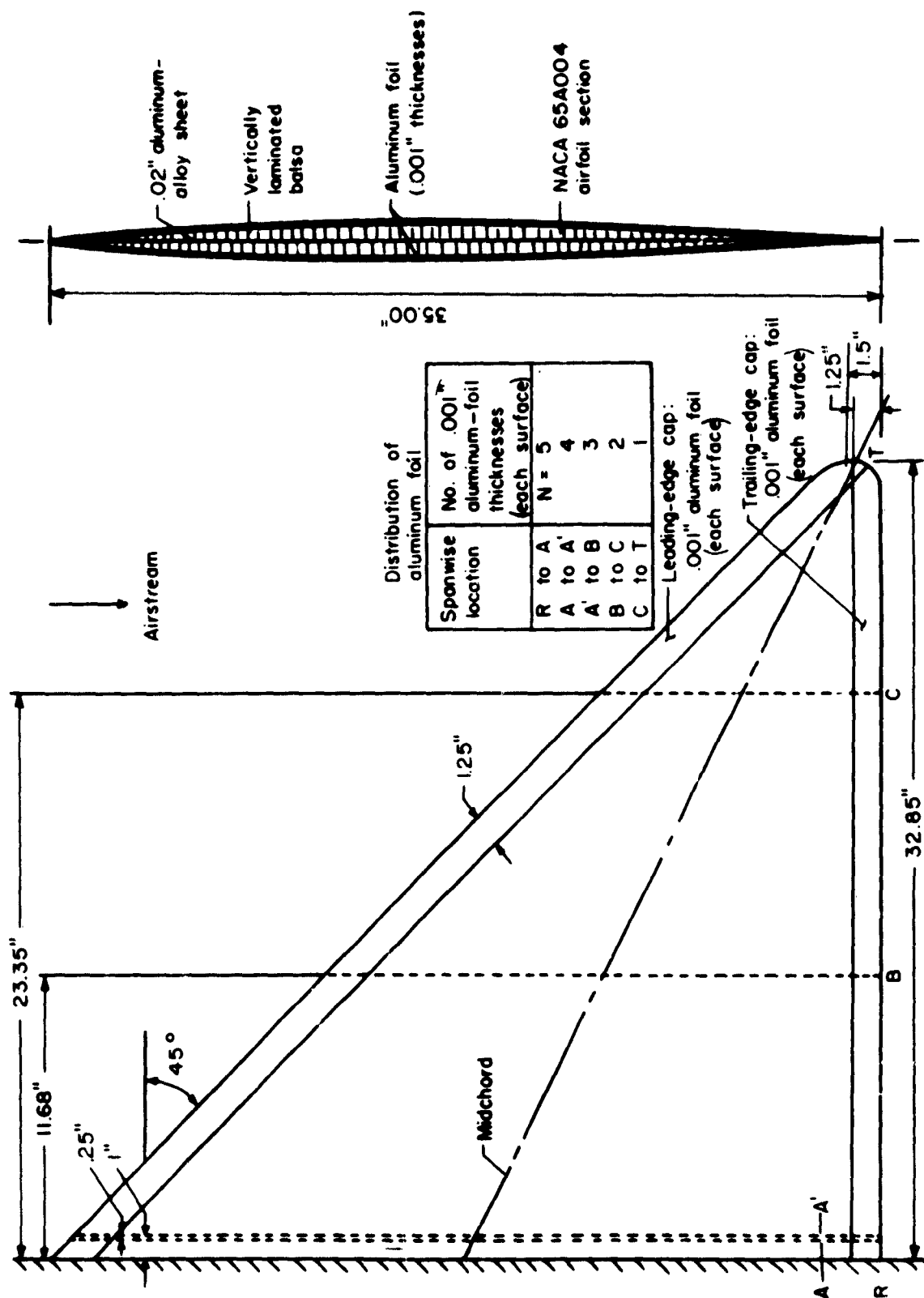
Figure 2.- Construction details of delta-wing model.
