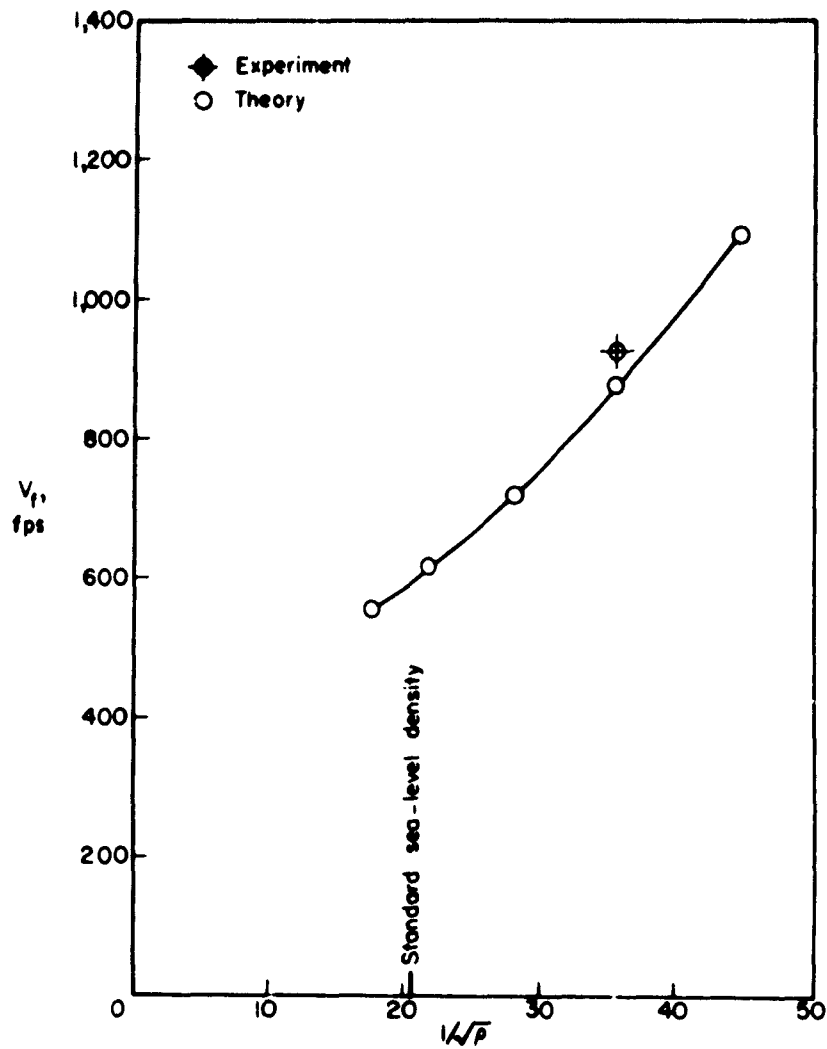
Figure 5.- Effect of density on calculated flutter speed for a Mach number of 0.85.
