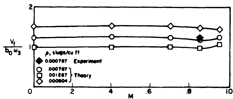
Figure 6.- Effect of Mach number on calculated flutter speed for various densities.
