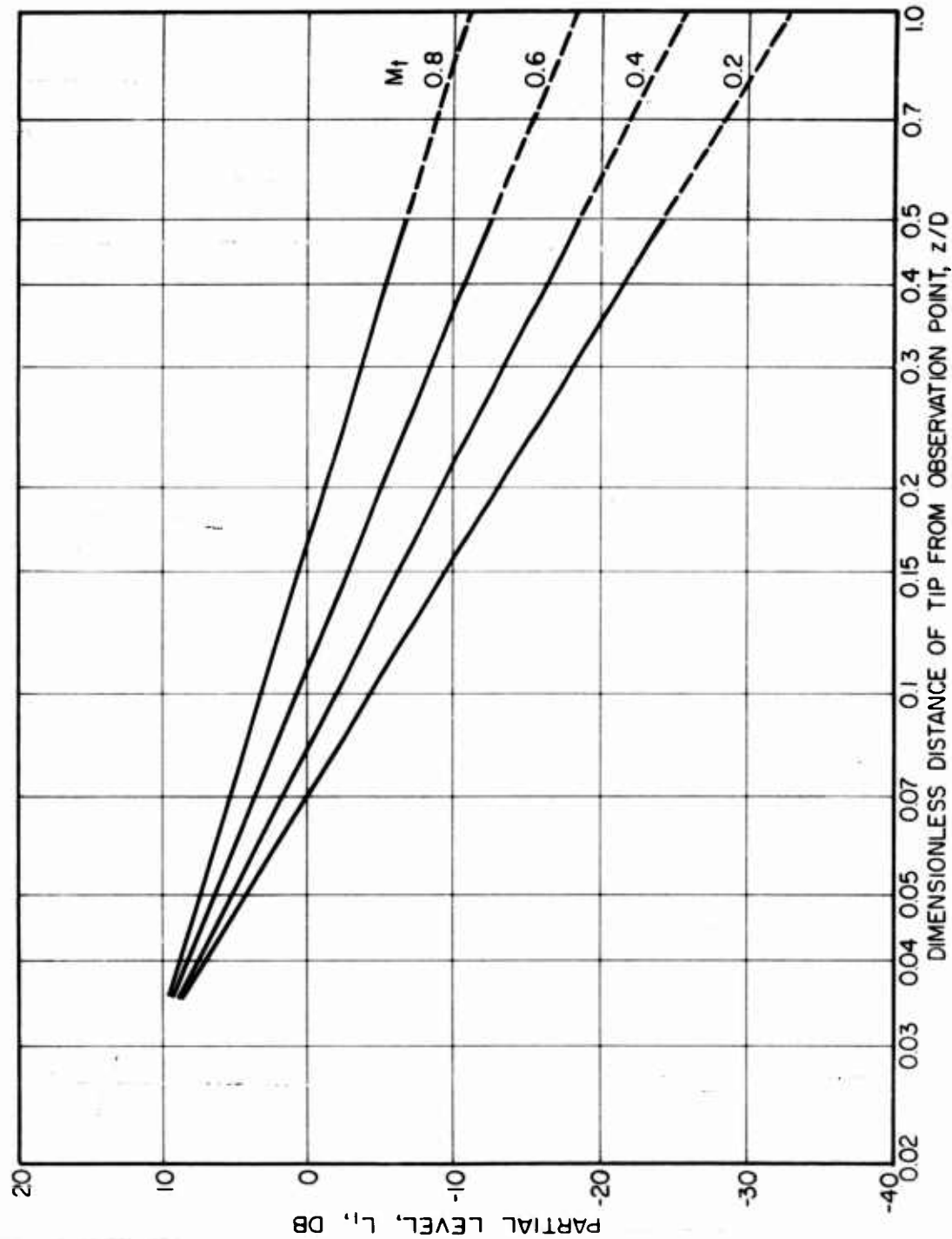
FIG. 3 NEAR FIELD PROPELLER NOISE CHART - 2.
