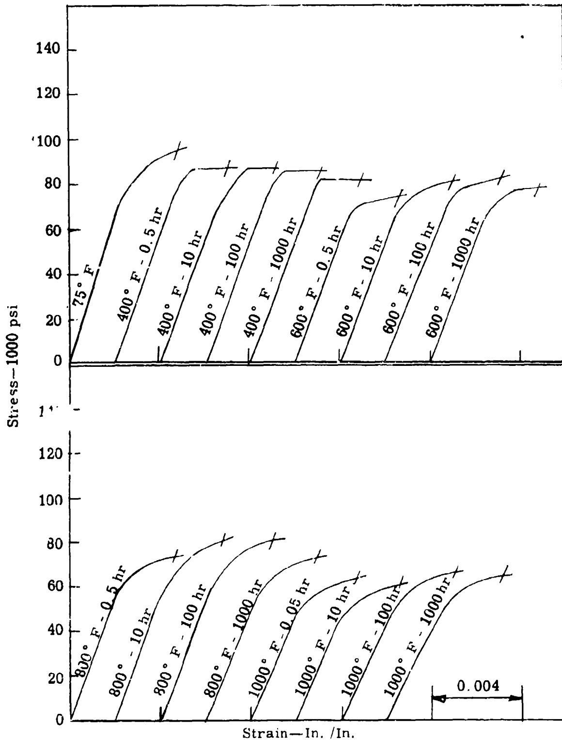
Fig. 130. Compressive stress-strain curves for quenched and tempered 17-22 A (S) alloy steel at various temperatures and exposure times.
