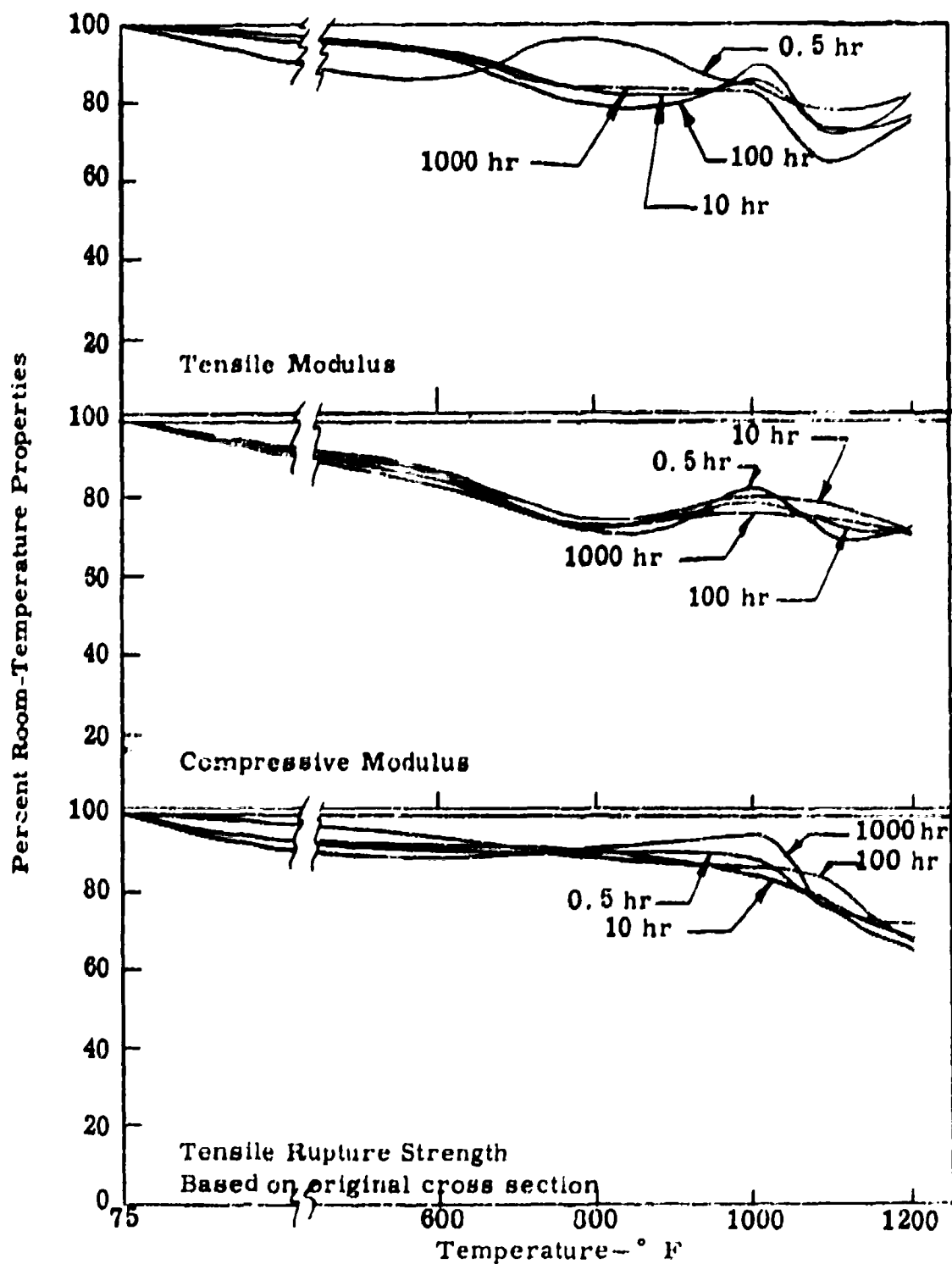
Fig. 23. Elevated-temperature properties as percent of room-temperature properties for quenched and tempered A-286 austenitic alloy sheet at different exposure times
