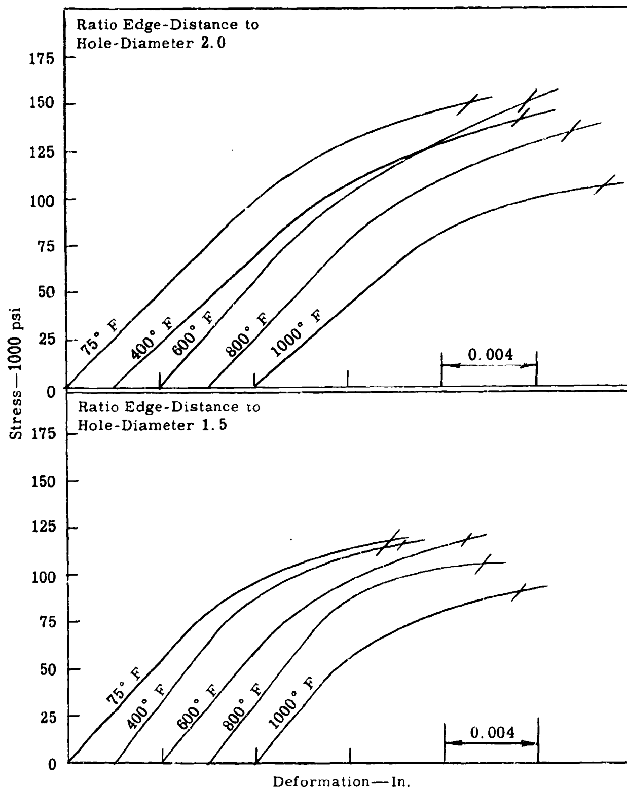
Fig. 131. Bearing stress-deformation curves for quenched and tempered 17-22 A (S) alloy steel sheet at various temperatures and one-half-hour exposure time.
