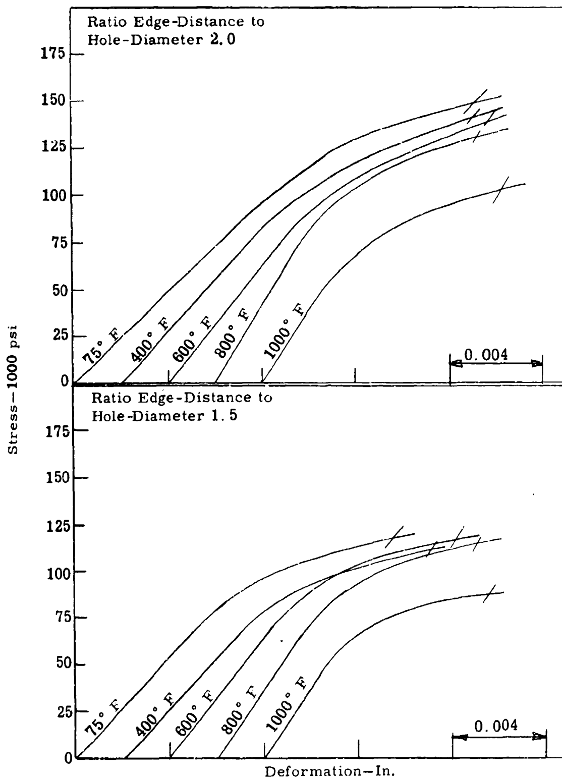
Fig. 132. Bearing stress-deformation curves for quenched and tempered 17-22 A (S) alloy steel sheet at various temperatures and ten-hour exposure time
