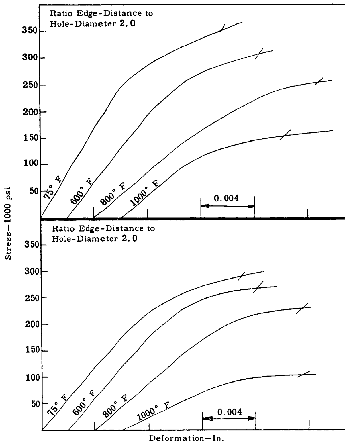
Fig. 51. Bearing stress-deformation curves for 17-7 PH stainless steel sheet (RH 950 condition) at various temperatures and one-half-hour exposure time.
