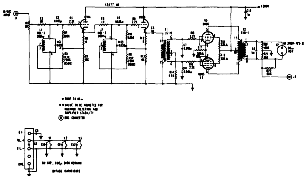
Fig. 11 - 60-cps generator-amplifier schematic
