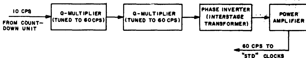
Fig. 10 - 60-cps generator-amplifier block diagram
