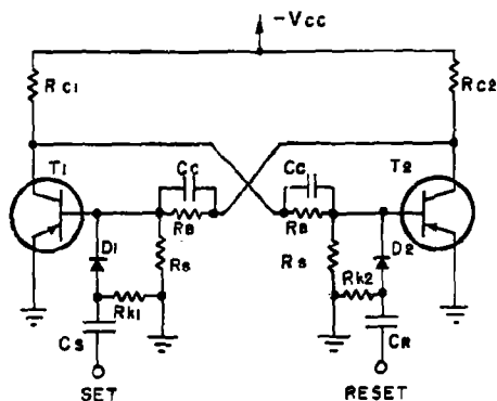
Figure 1. Two-Transistor Flip-Flop With Set and Reset Networks
