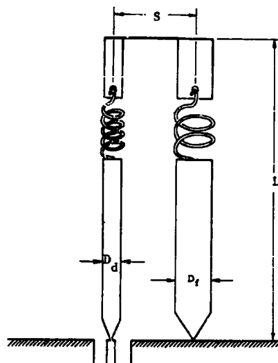
Figure 4. Inductively loaded, single-folded monopole.
