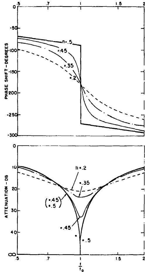
Figure 17.-Attenuation and phase characteristics of a parallel-T network with various values of n .
