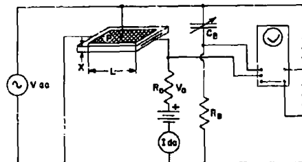
Figure 3. Field Effect Experiment.
