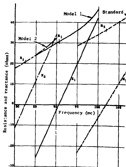
Figure 8. Resistance and reactance vs frequency for two ferromagnetically loaded monopoles and an unloaded standard monopole.
