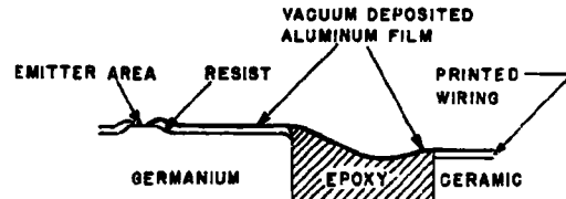
2d CROSS-SECTIONAL VIEW SHOWING VACUUM DEPOSITED LEAD.
