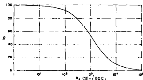
Figure 2. Grounded Emitter Current Gain ( \beta ) versus Surface Recombination Velocity S . (for assumed conditions \beta = 50 at S = 1250 )
