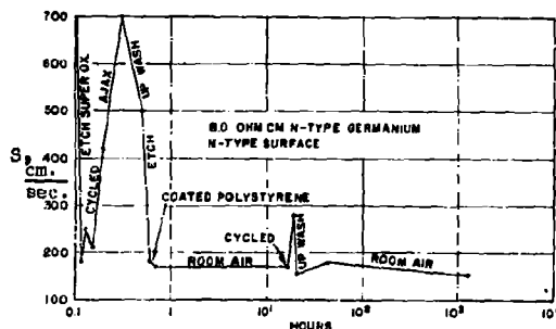
Figure 10. Surface Recombination Velocity S versus Hours Time in Room Air for Polystyrene Coated N-type Germanium.
