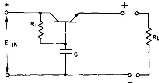
Figure 6.-Transistor-simulated series inductance.
