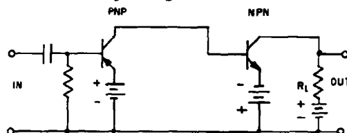
Figure 4.—Complementary symmetry direct-coupled transistor amplifier.
