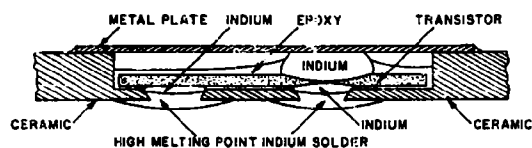
Figure 8. Cross Sectional View of Hermetically Sealed Transistor Package.
