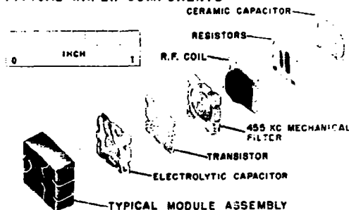
Figure 5. - Typical wafer components for micro-modules.
