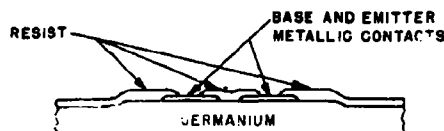
2b ENLARGED CROSS-SECTIONAL VIEW OF TRANSISTOR SURFACE
