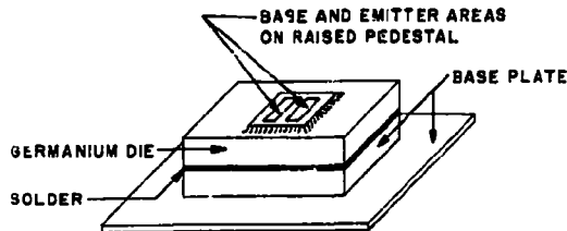
2a 3-DIMENSIONAL VIEW OF TRANSISTOR SOLDERED TO BASE PLATE.
