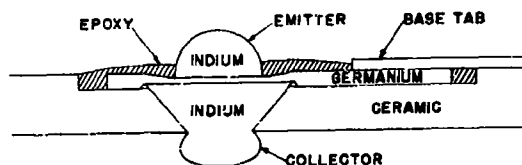
TRANSISTOR INTEGRATED INTO PRINTED CIRCUIT BOARD.
