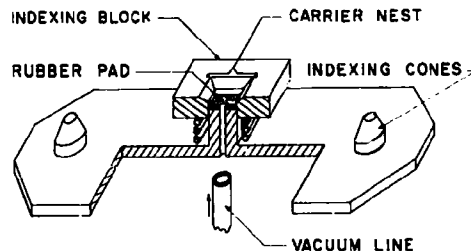
Figure 2. Carrier assembly for conveying and indexing wafers, showing spring that holds indexing block in raised position.
