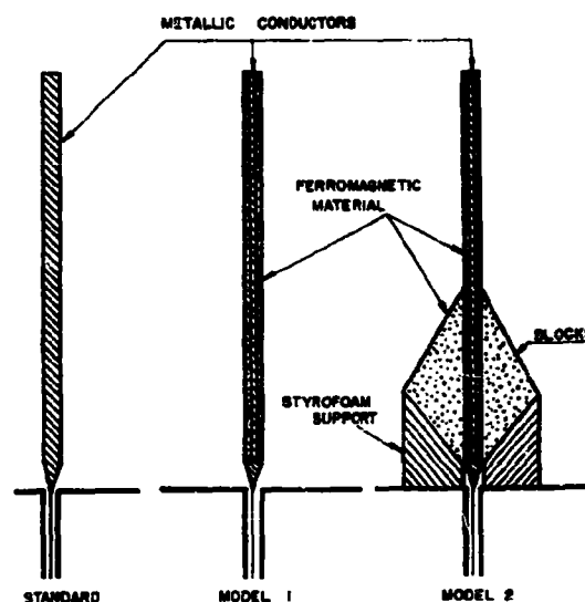
Figure 7. A standard monopole and two ferromagnetically loaded monopoles.
