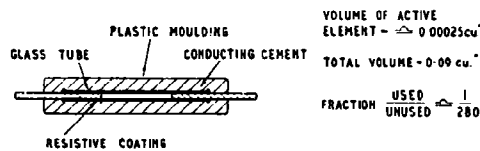
(a) GRADE 2 INSULATED RESISTOR.
