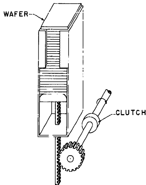
Figure 7. Stack feed with mechanism for maintaining top wafer at constant level.
