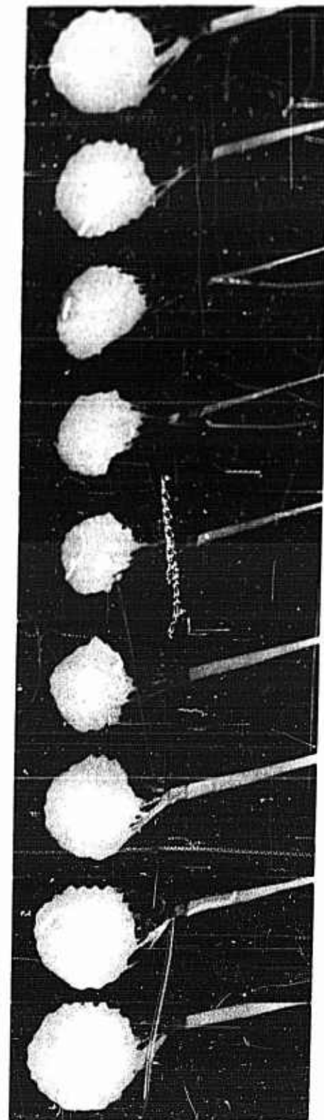
Parachute S/N 509M Diameter 3.66 ft Porosity 10.12 Percent
