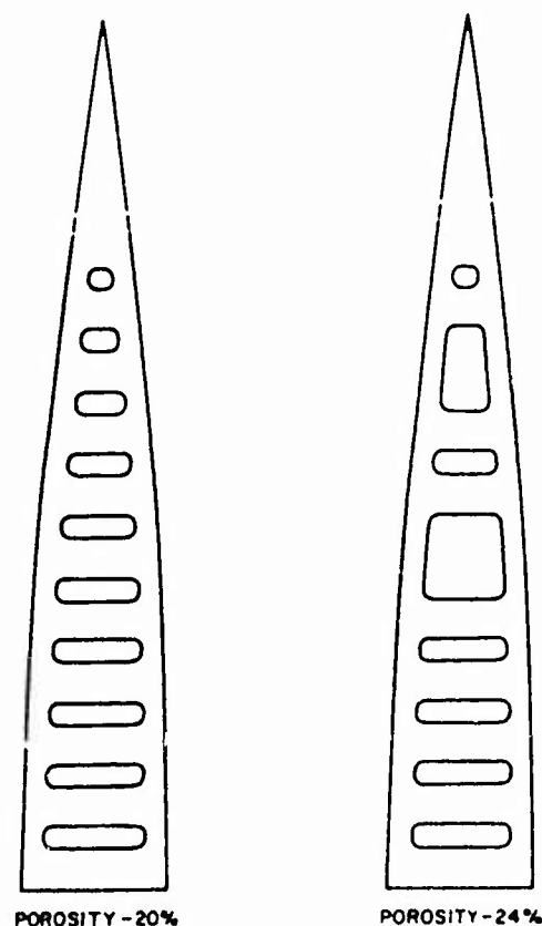
Figure 12. Typical Canopy Gore Layouts Showing Details of the Slots
