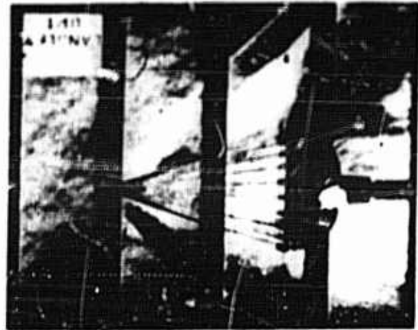
(a) Sequence of Three Consecutive Frames Showing Variation in Appearance of Bow Shock at M = 1.57 ( \alpha = 0^\circ ) (Camera Speed - 1560 frames per second)
