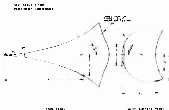
Figure 9. Panel Layout - Guide Surface Ribless Parachute
