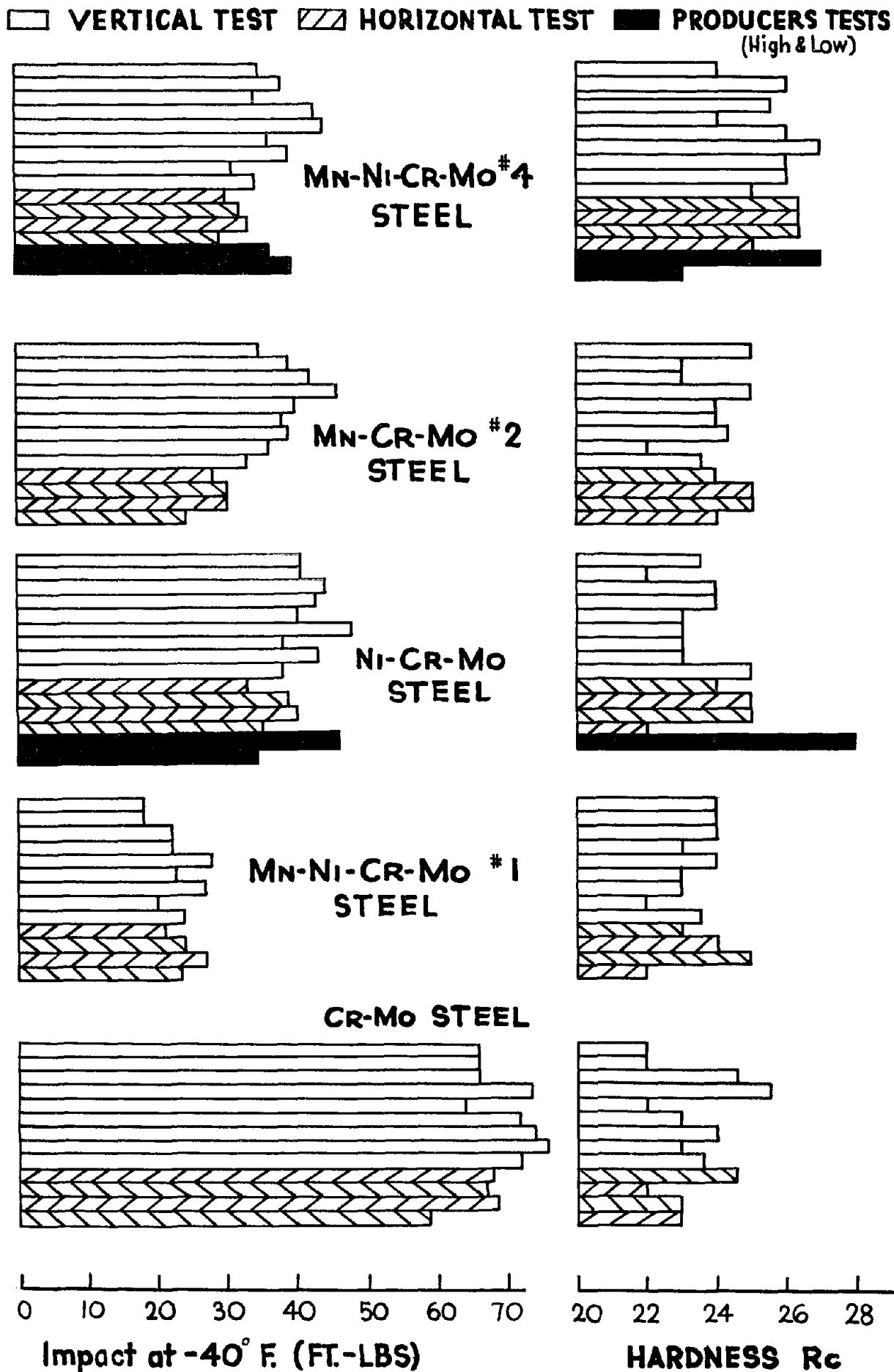
Figure 19—V-notch Charpy values at -40 degrees F for the 1 x 4-inch keel castings after quench and tempering heat treatment
