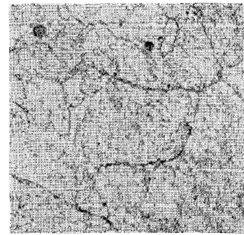
Figure 50—Microstructure of Mn-Ni-Cr-Mo cast steel, homogenized 1650 degrees F for 60 minutes. Austenitized for the conditions shown, water quenched and tempered at 1250 degrees F for 30 minutes. Zepherin chloride etch. 1000X. N.B. This condition was characteristic of heats Mn-Ni-Cr-Mo #1, #2 and #3 but not of heat #4. (See Section IX)
