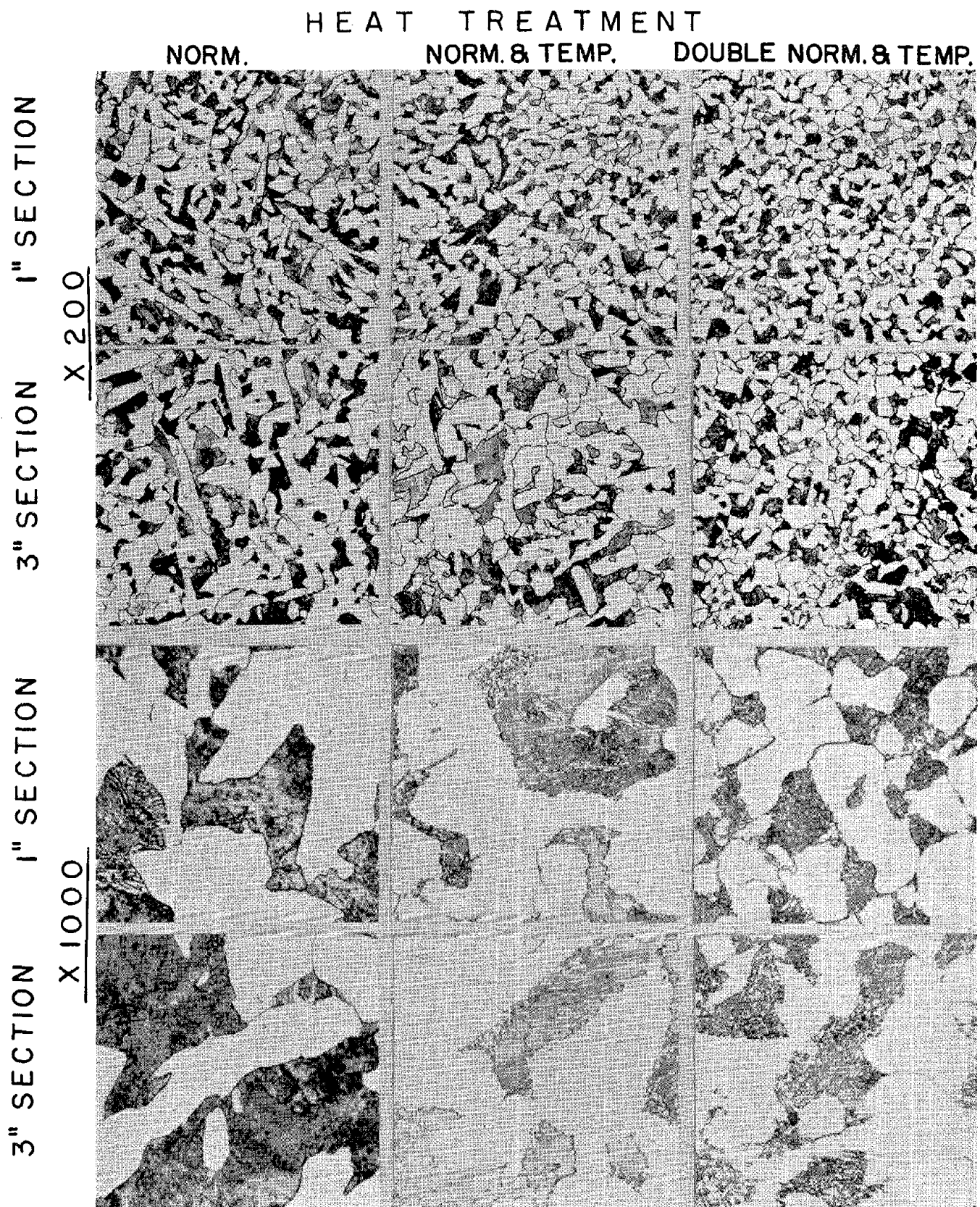
Figure 87—Normalized carbon cast steel. Comparison of microstructures from the center of one-inch and three-inch sections. Left—single normalize, 1650°F - 30 minutes Center—normalize, 1650°F - 30 minutes, and tempered, 1250°F - 60 minutes Right—double normalize, both at 1650°F - 30 minutes, and tempered, 1250°F - 60 minutes
