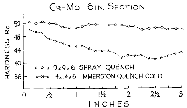
Figure 15—As-quenched hardness survey of Cr-Mo steel insert-bars in carrier blocks of 6-inch section with different severity of water quench
