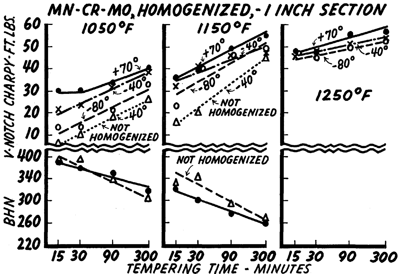
Figure 60—The effect of tempering on the Charpy V-notch impact properties of Mn-Cr-Mo cast steel - 1-inch section. Heat treatment prior to quenching: (1) none; (2) homogenization at 1750 degrees F for 300 minutes. Air cooled. Water quench from 1650 degrees F after 90 minutes. Water quenched from tempering temperature.
