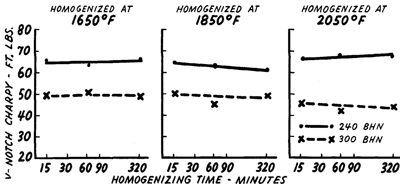
Figure 32—Cr-Mo 1-inch thick section, -40 degrees F. The effect of homogenization on the Charpy V-notch impact properties of Cr-Mo cast steel quenched 1650 degrees F and tempered to the hardnesses shown on the chart.
