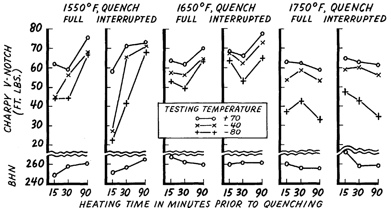
Figure 47—Cr-Mo 6-inch section. The effect of heating temperature and time prior to quenching on the impact properties of full and interrupted, quenched and tempered (250 BHN) steel.
