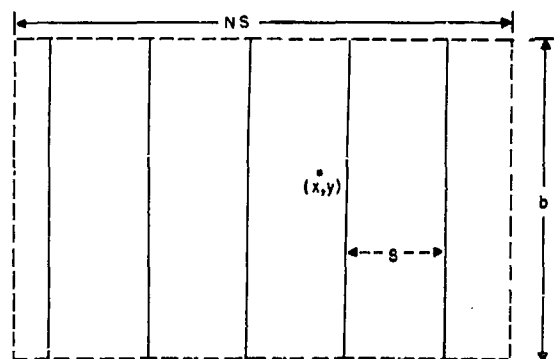
FIGURE 11. A rectangle of random sweeps.
