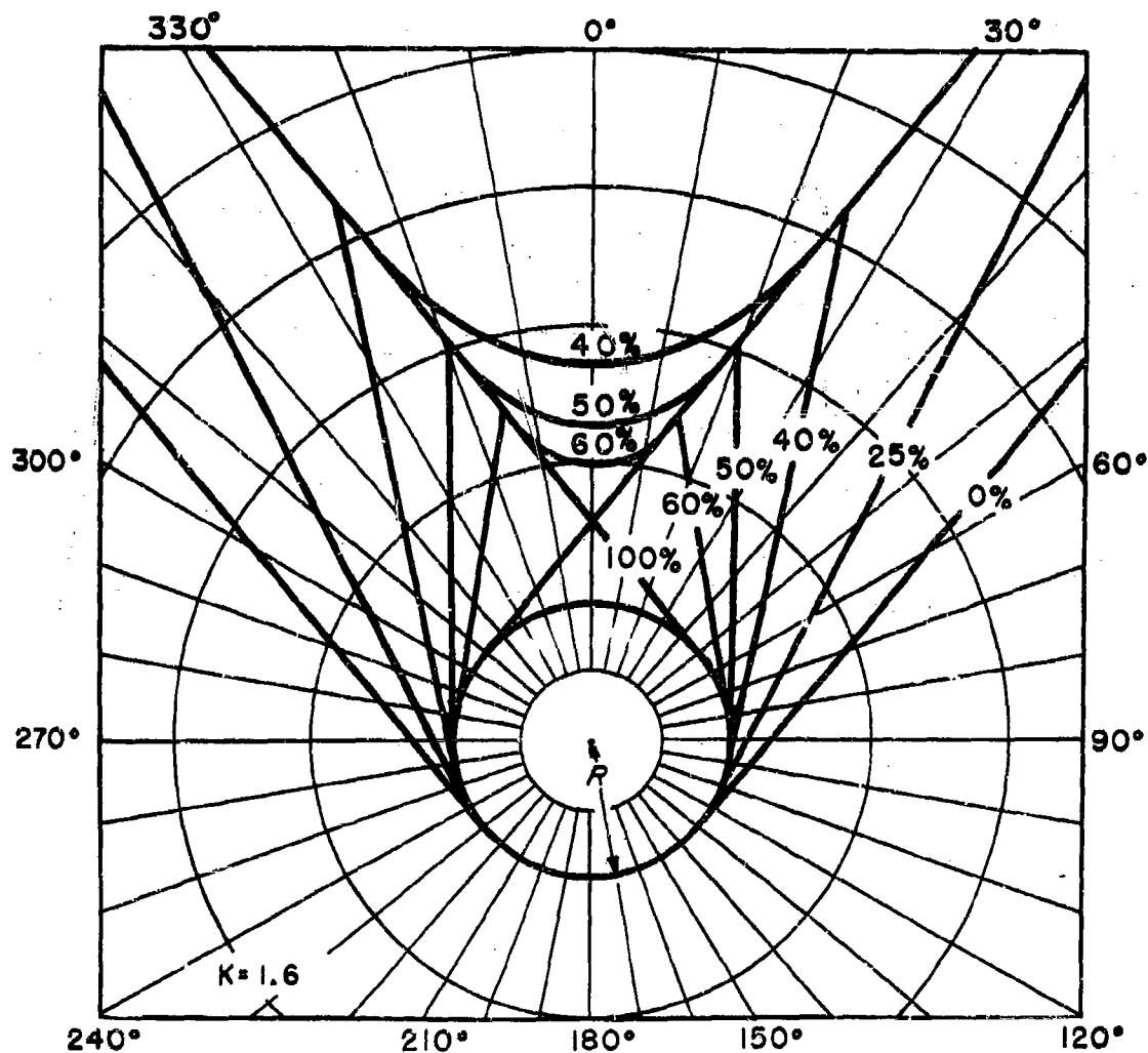
FIGURE 11. Contact probability curves. k = 1.6 .
