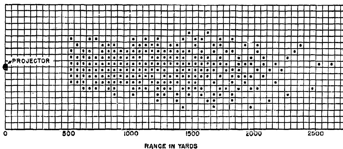
FIGURE 15. One-ping probability diagram.
