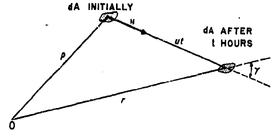
FIGURE 16. Entry of target into dA .
