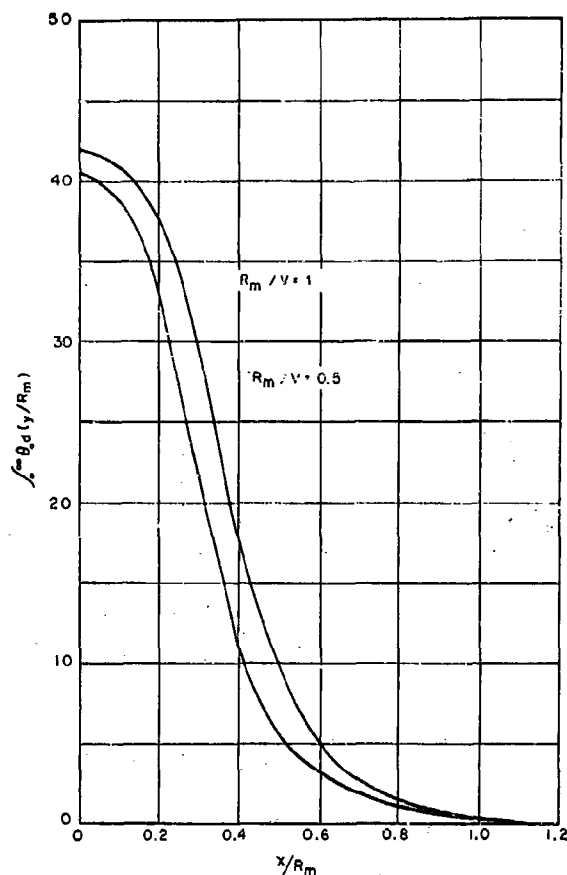
FIGURE 9. Integral of equation (27) as a function of lateral range/maximum range.
