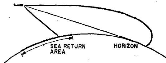
FIGURE 3. Schematic illustration of vertical antenna pattern and sea return area for airborne early warning radar.
