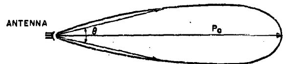
FIGURE 1. Idealized pattern of a microwave search radar. Length of radius vector is proportional to power radiated in that direction.
