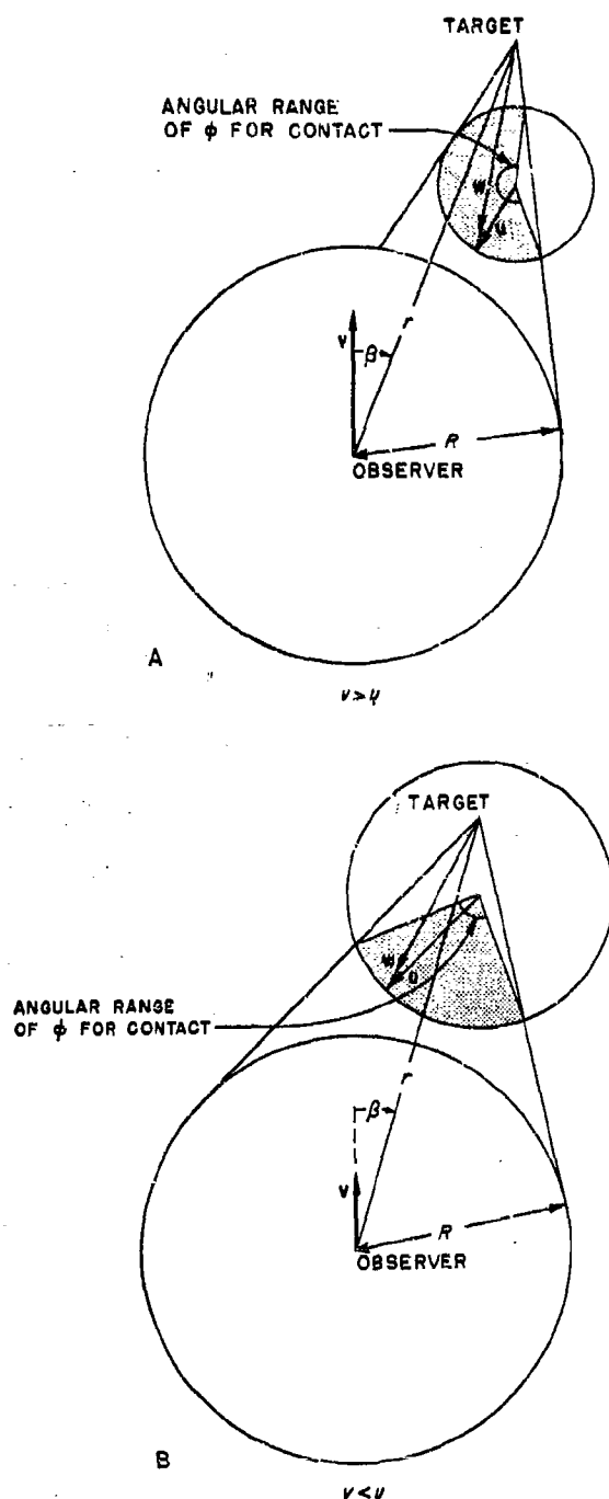
FIGURE 10. Probability of entering circle.
