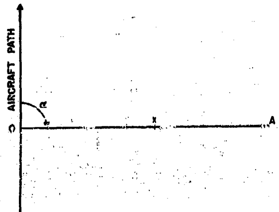
FIGURE 9. Straight aircraft path: averaging process. ( a = OA .)
