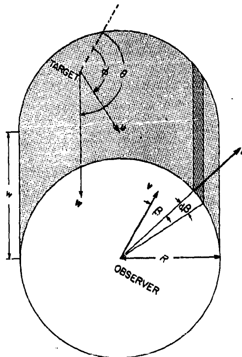
FIGURE 8. Area of targets entering a circle.
