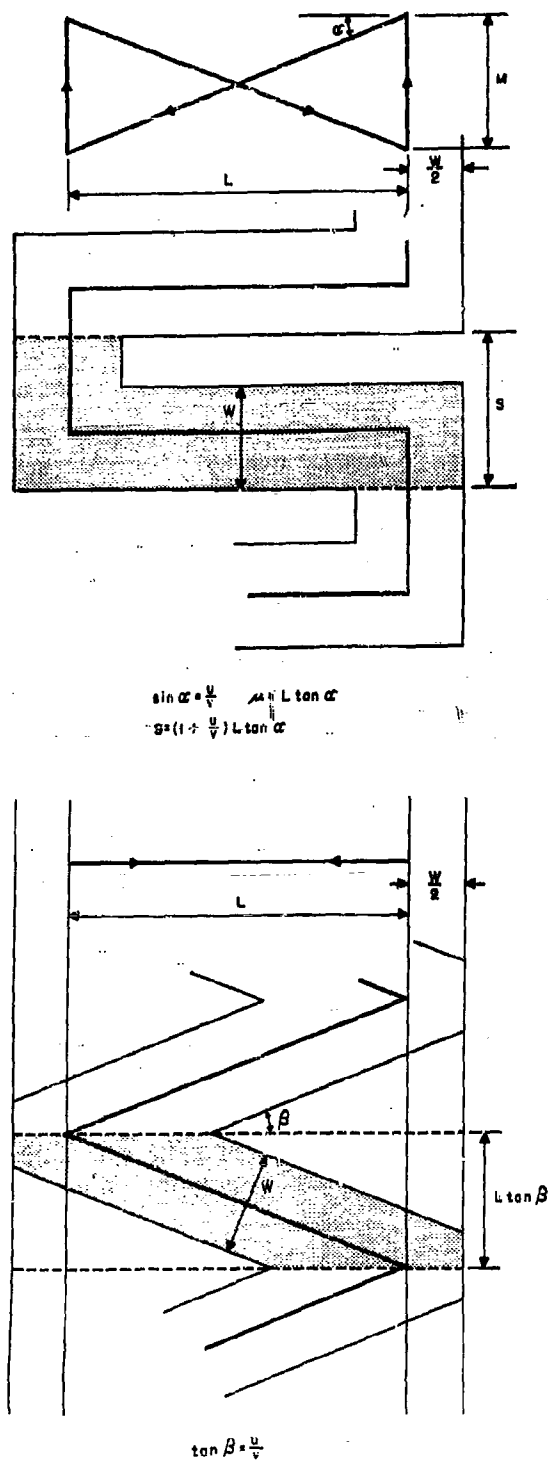
FIGURE 6. A comparison of barriers.
