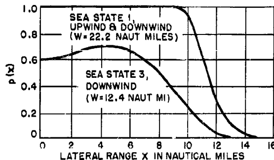
FIGURE 13. Lateral range distribution. Computed using blip-scan data of Figure 9.
