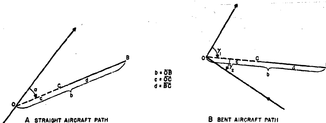
FIGURE 11. General disposition of target with respect to aircraft path.
