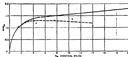
FIGURE 8. Path swept/maximum range as a function of maximum range—comparison of computed (solid line) and operational (dotted line) results (surfaced submarines).
