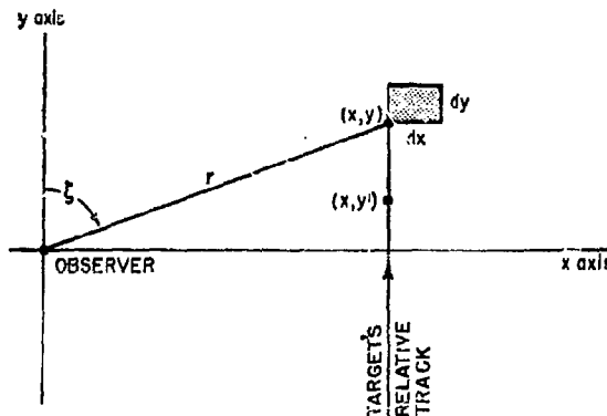
FIGURE 7. Target detection at given relative position.
