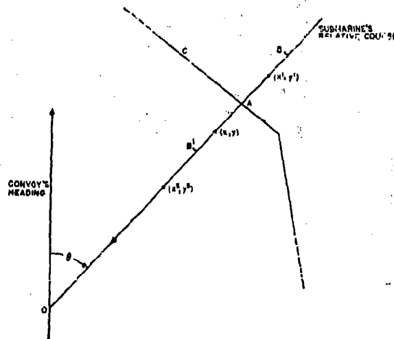
FIGURE 5. Successive positions seen during approach.
