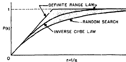
FIGURE 12. Probabilities with parallel sweeps.
