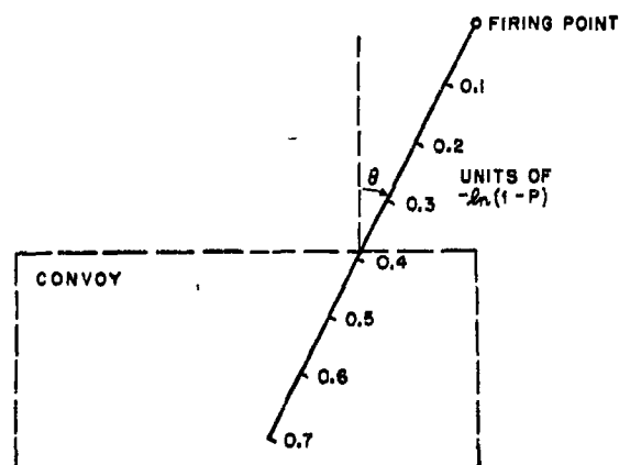
FIGURE 11. Graphical calculation of probability of hitting.
