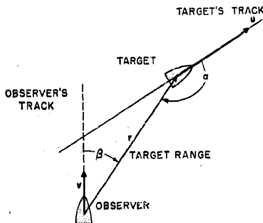
FIGURE 3. Geographic tracks, ranges, and bearings.
