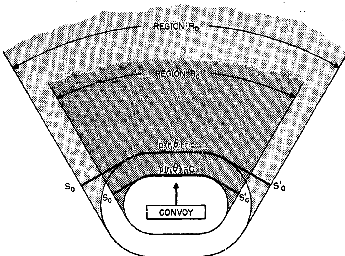
FIGURE 23. Placement of screen.
