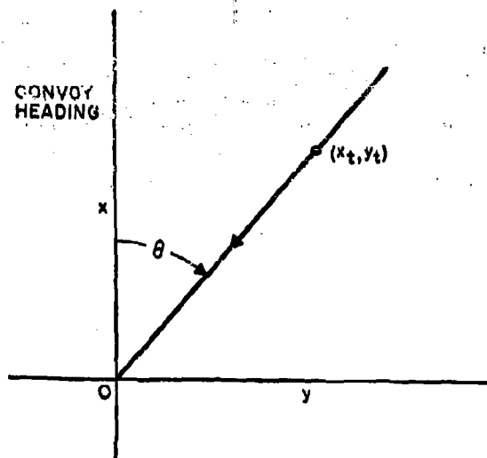
FIGURE 3. Collision approach: the coordinate system.
