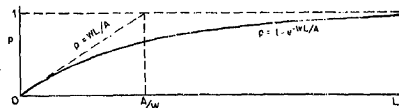
FIGURE 9. Detection with random search.
