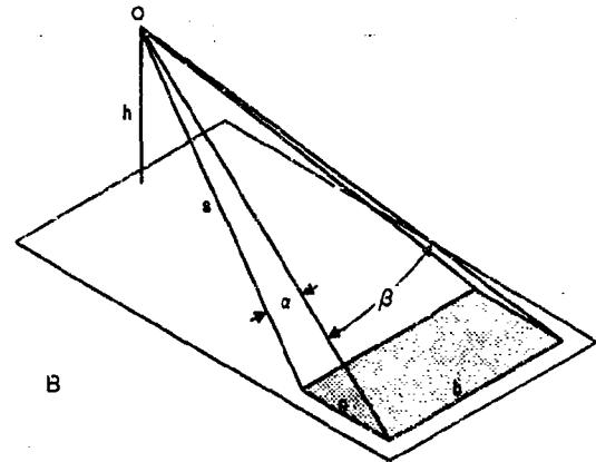
FIGURE 3. Solid angle subtended by wake.
