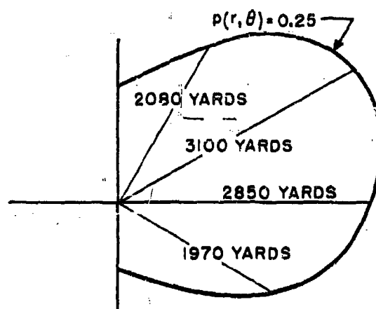
FIGURE 20. Danger zone template.
