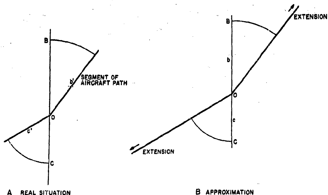
FIGURE 16. The geometrical principles of path and track approximation.
