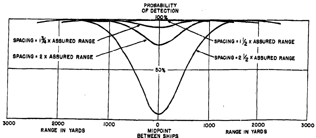
FIGURE 22. Probability versus lateral range for a pair of ships with various spacings.
