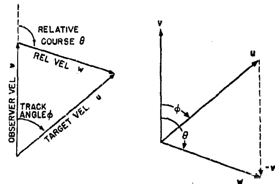
FIGURE 1. True and relative velocities and angles.
