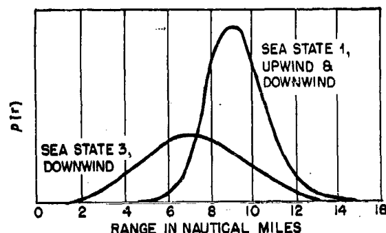
FIGURE 11. True range distribution for search ahead only. Computed using blip-scan data of Figure 9.
