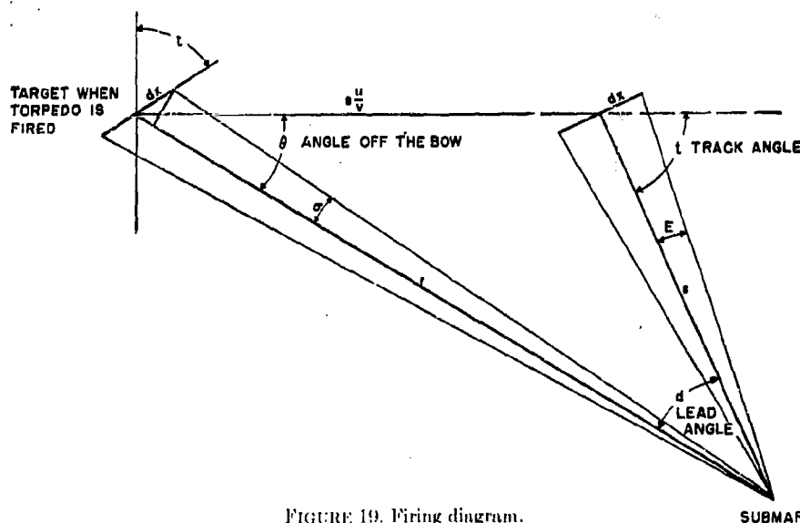
FIGURE 19. Firing diagram.
