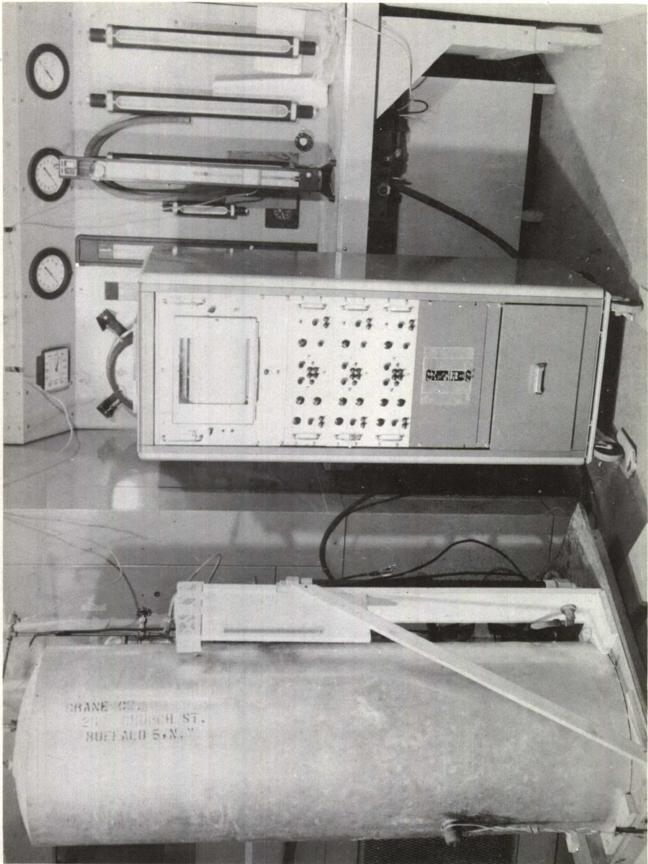
Figure 10. Photograph, CAPSULE VOLUME TANK & INSTRUMENTATION
