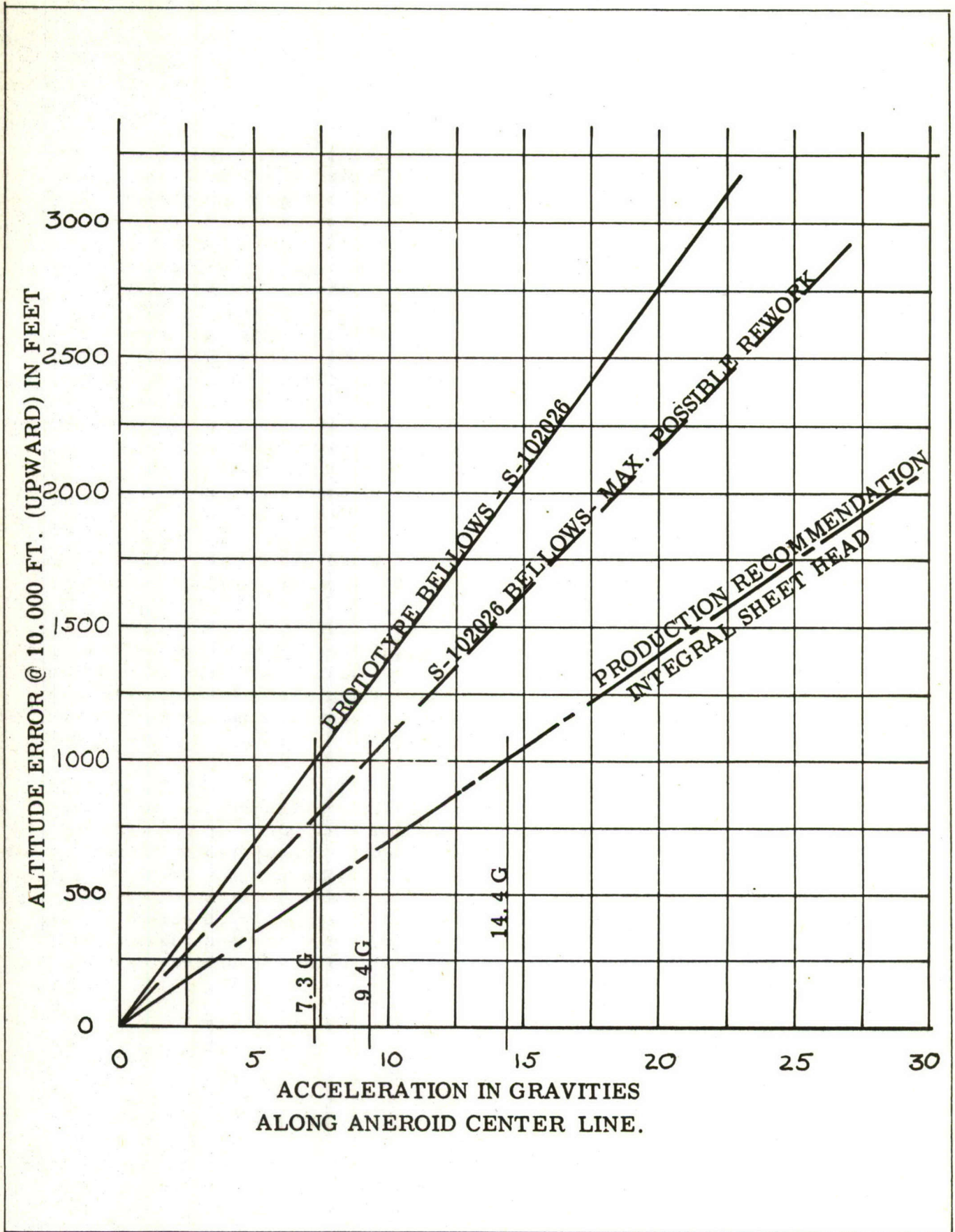
Figure 6. ALTITUDE ERROR VS ACCELERATION
