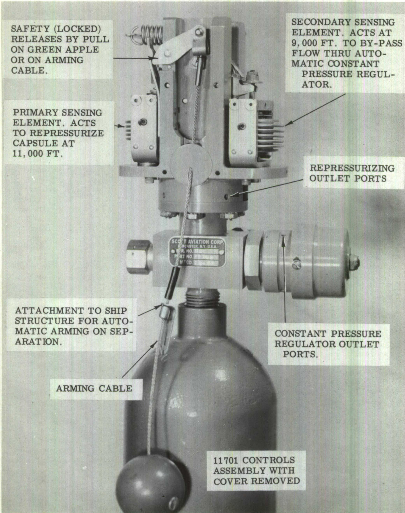
Figure 3. CONTROL ASSEMBLY, COVER REMOVED, CABLE SIDE
