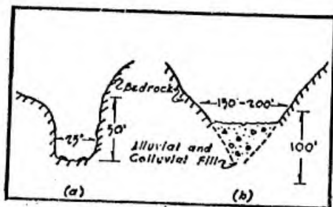
Figure 43. Diagrammatic sketches of contrasting canyon floors of White Mountain drainages. (a) Floor of lower Lone Tree Creek; (b) Floor of lower Silver Canyon.
