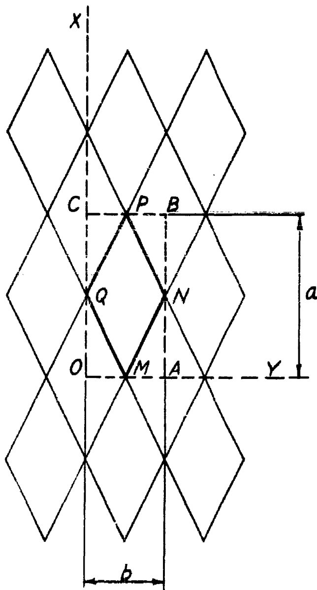
Figure 2. -- Nodal lines of assumed diamond-shaped buckling pattern.
