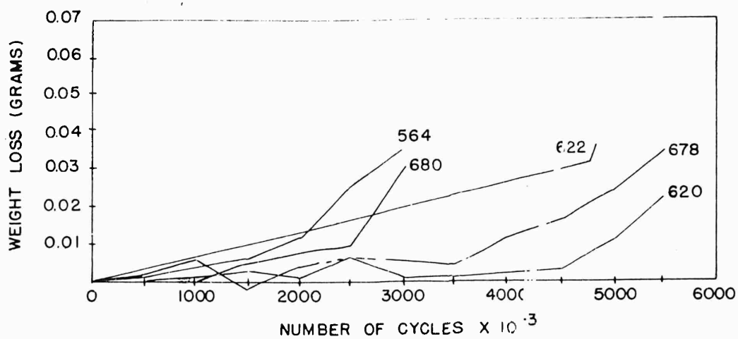
SHOES FOR SEVERELY COLD ROLLED SPECIMENS
