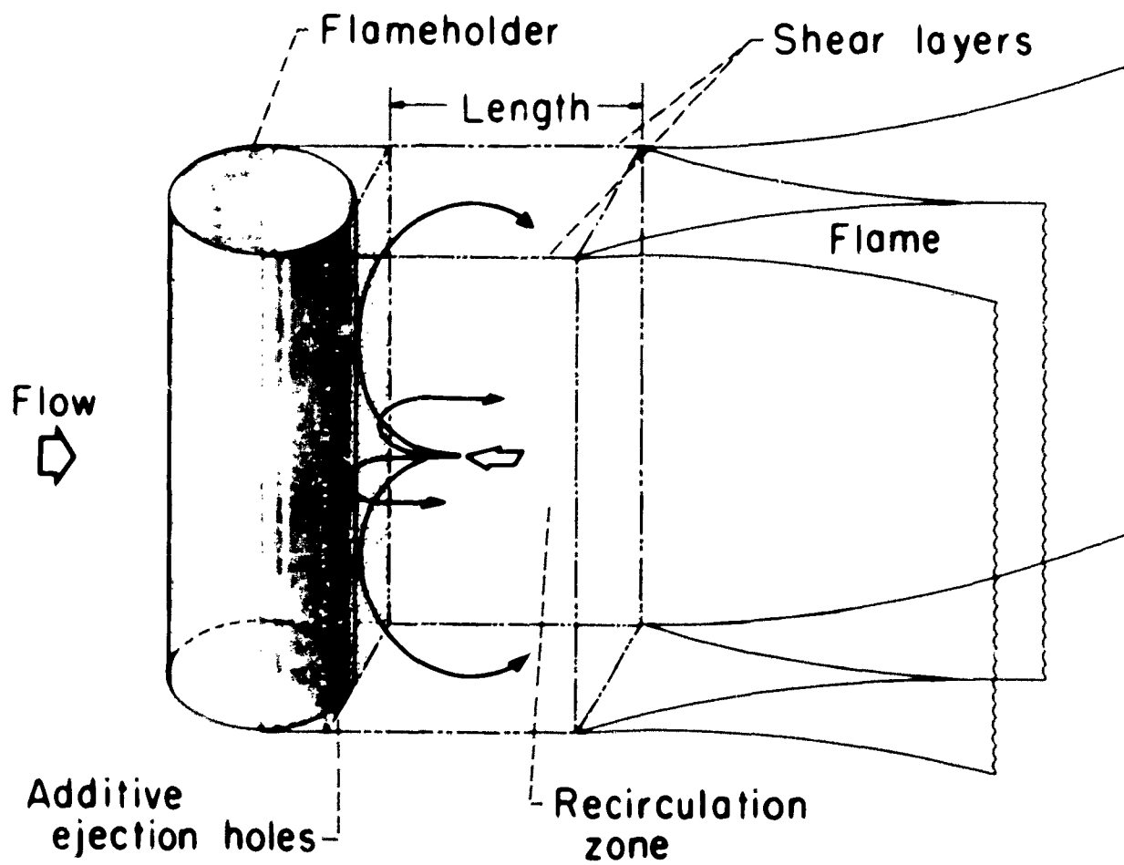
Figure 1. - Zukoski and Marble flameholding model.
