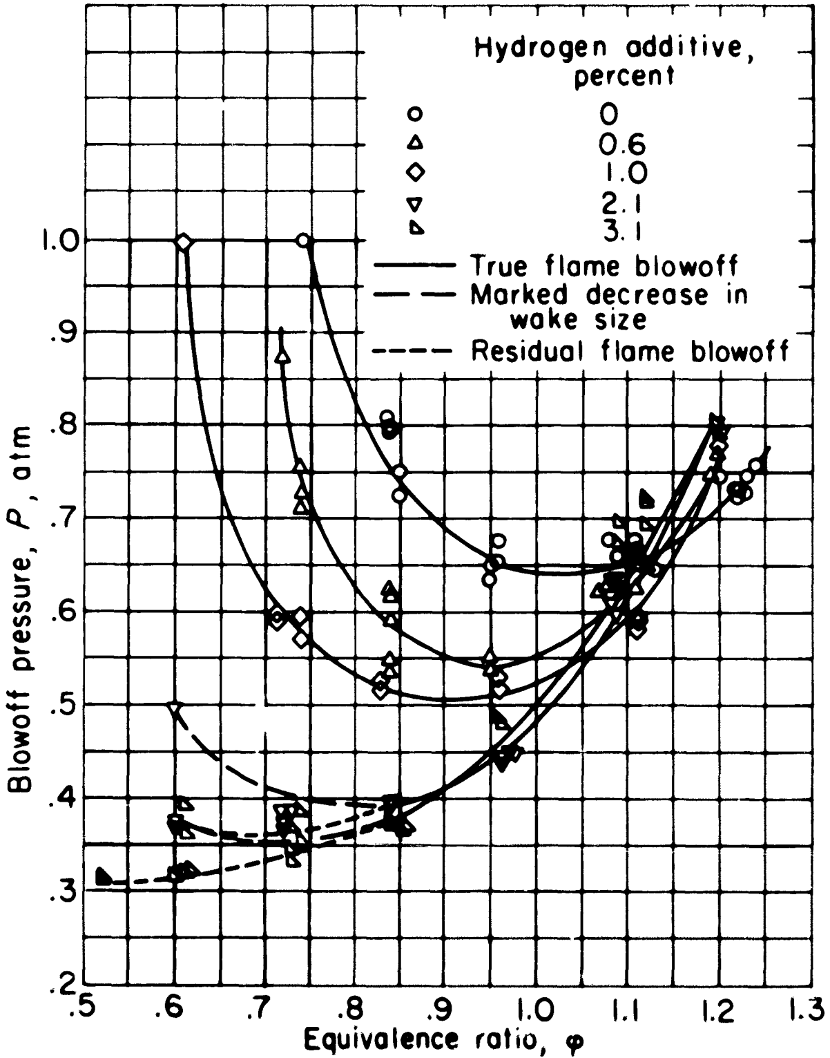
Figure 4. - Effect of hydrogen additive on propane-air flame stability. Upstream injection; Reynolds number, 4.3 \cdot 10^4 ; mean velocity, 153 feet per second at a pressure of 1 atmosphere
