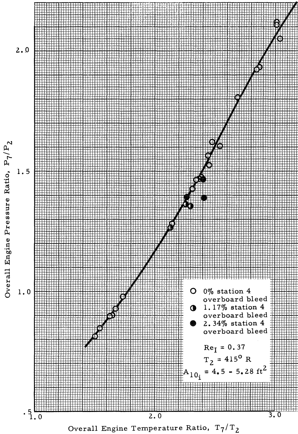
Fig. 13 Engine Pumping Characteristics
