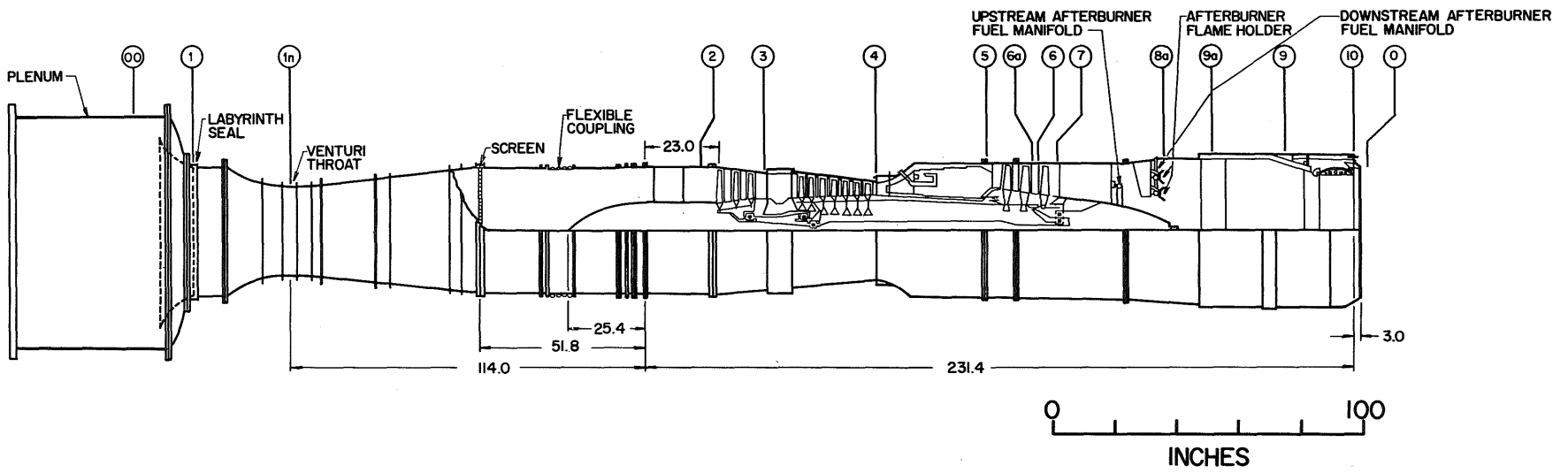
Fig. 5 Test Article Station Locations
