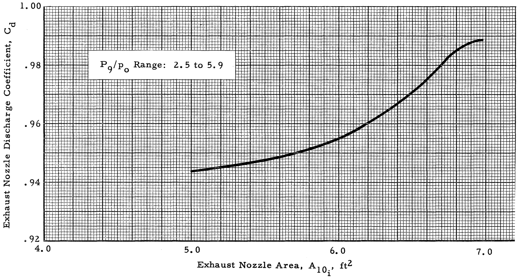
Fig. 17 Exhaust Nozzle Discharge Coefficient
