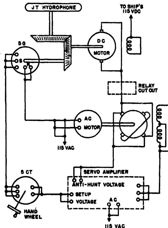
FIGURE 10. Schematic diagram of JT power training system.
