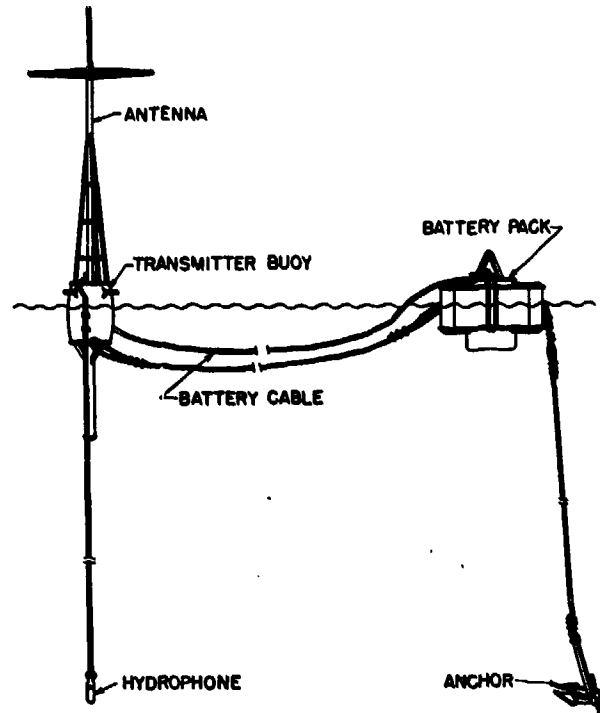
FIGURE 11. Diagram of JM-1 buoy in the water.
