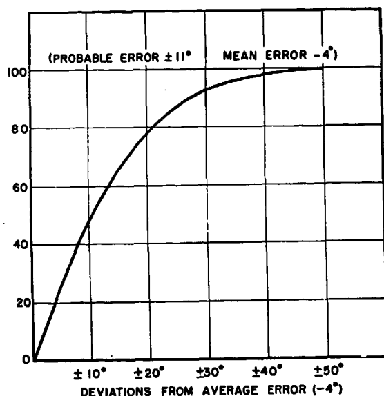
FIGURE 41. Bearing accuracy of DRSB.
