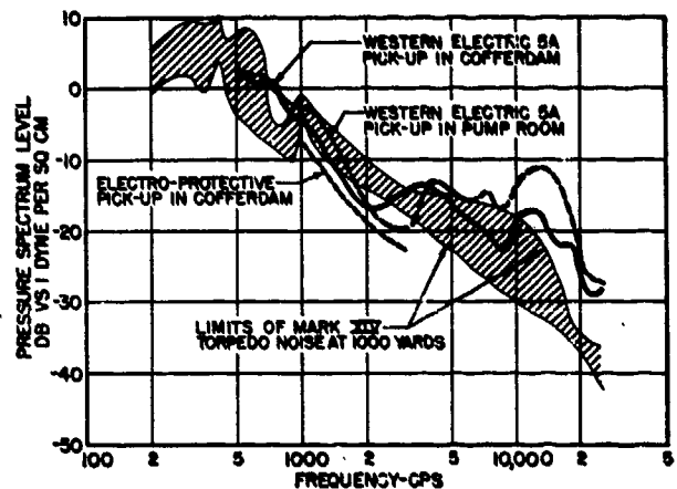
FIGURE 7. Variation of self-noise of SS Colorado at 17 knots with type and location of pickup units, compared with U.S. Mark XIV torpedo noise.
