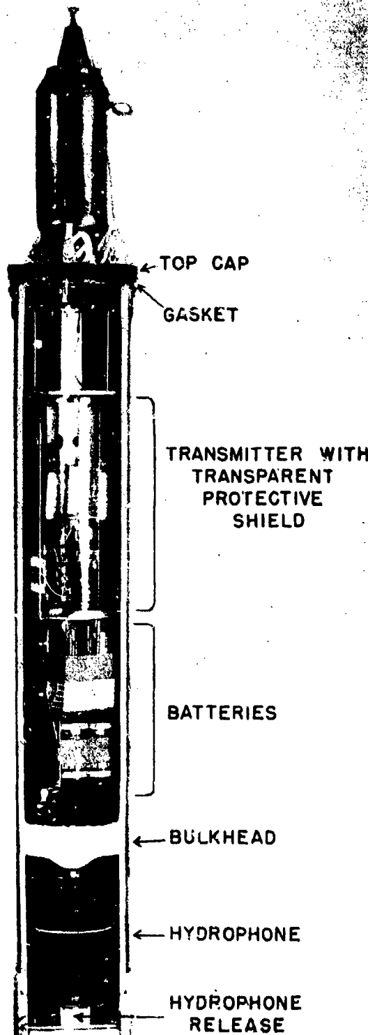
FIGURE 6. Section view of AN/CRT-1A buoy.
