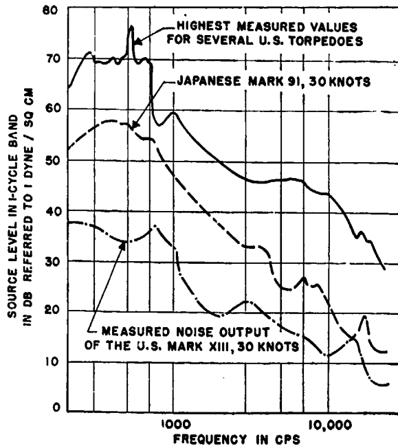
FIGURE 4. Noise measurements for several types of torpedoes.
