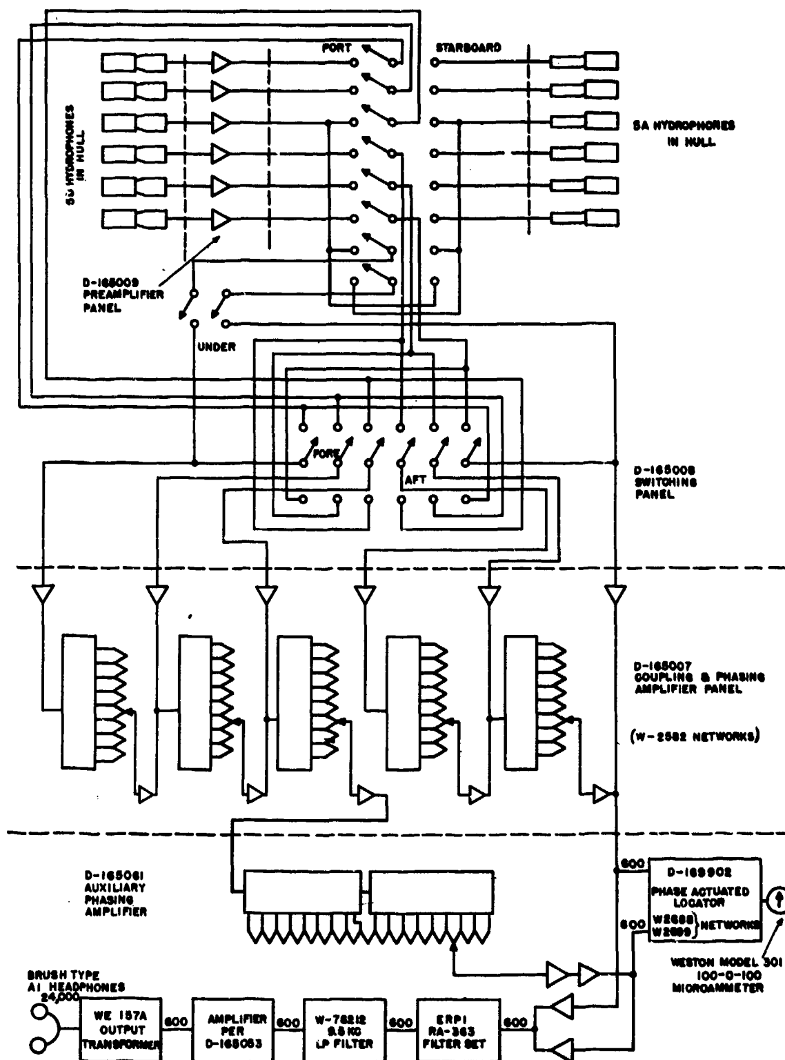
FIGURE 3. Electrically steered sonic listening equipment on Elcobel .
