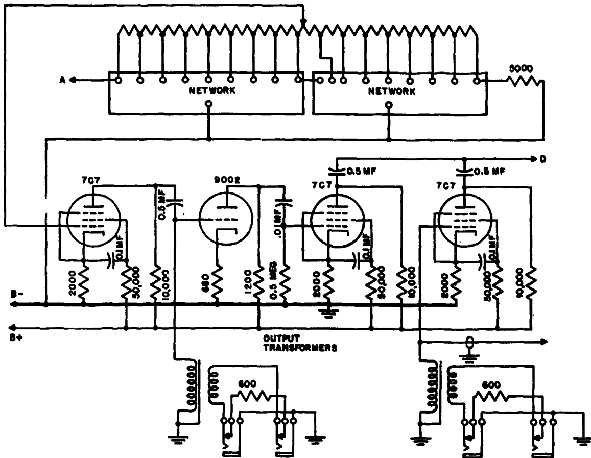
FIGURE 4. Schematic diagram of auxiliary phasing amplifier.
