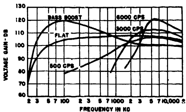
FIGURE 33. Frequency response of amplifier for through-the-hull equipment.
