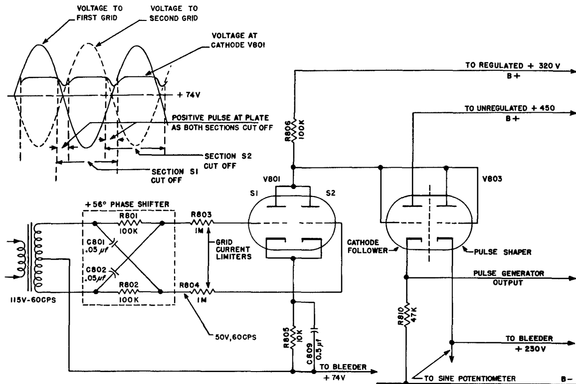
FIGURE 44. Indicator schematic; pulse generator portion.
