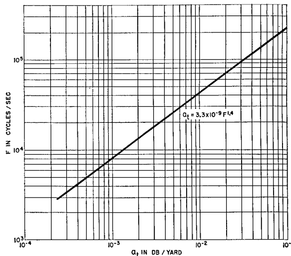
FIGURE 5. Average attenuation coefficient a_t increases approximately as 1.4 power of frequency F .
