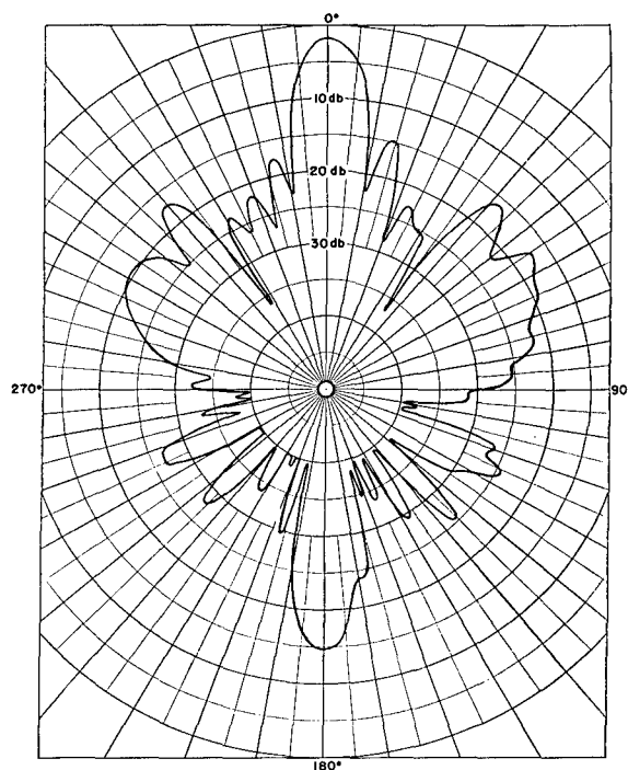
FIGURE 18. Directivity pattern of CP10Z-2 (used as a projector) measured at 40 kc in a plane perpendicularly bisecting the long axis.
