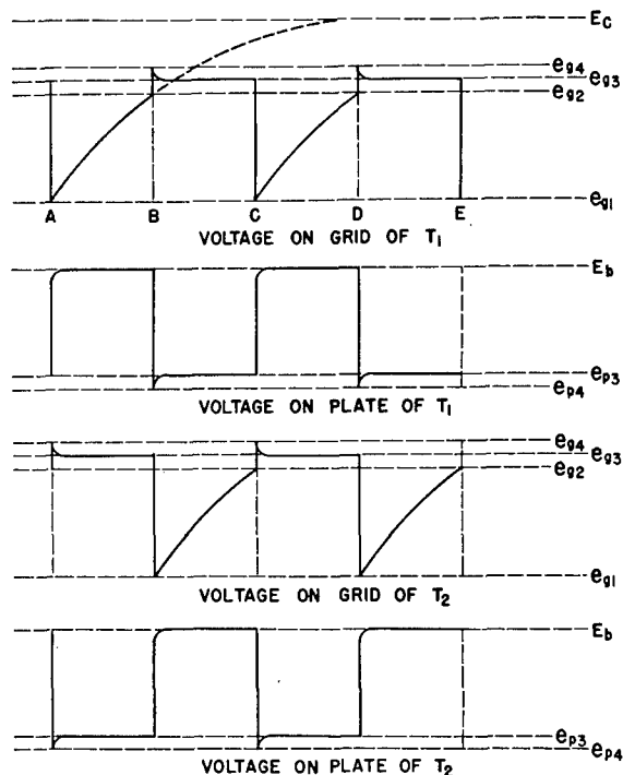
FIGURE 19. Positive bias multivibrator, time relationships.
