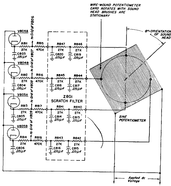
FIGURE 45. Sweep generator simplified diagram.
