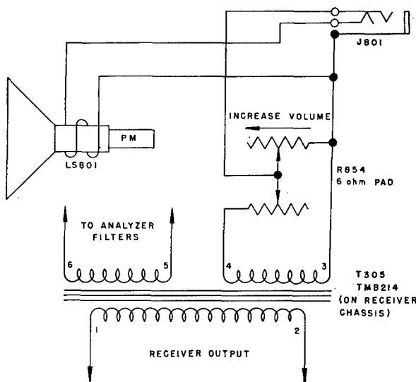
FIGURE 49. Loudspeaker schematic.
