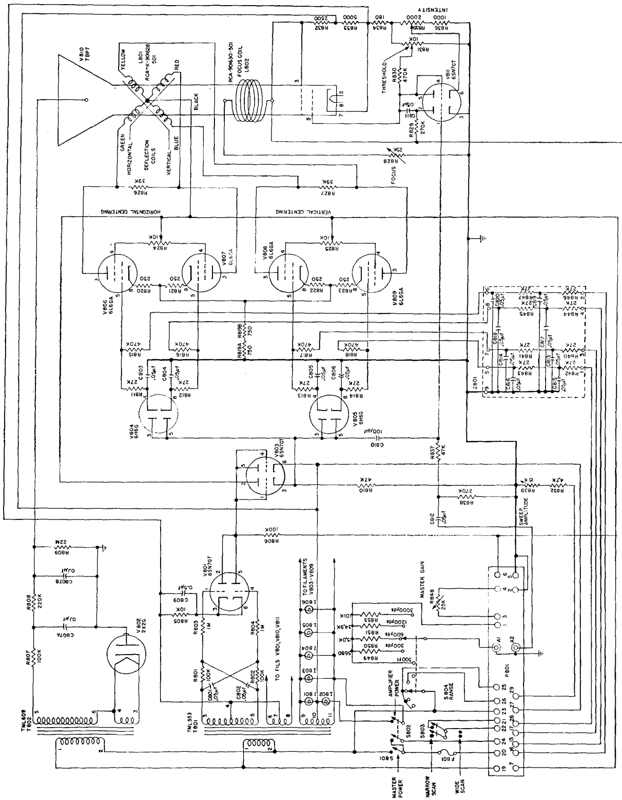
FIGURE 43. Indicator wiring diagram.
