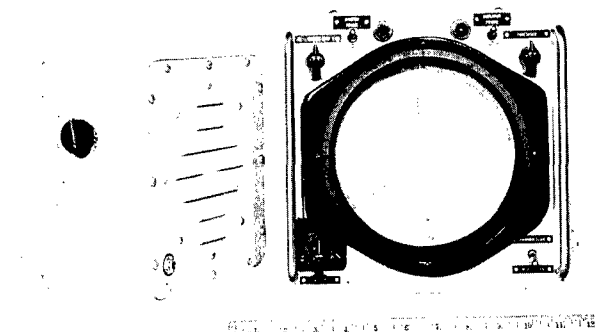
FIGURE 1. FM systems (here, QLA) differ from older types of underwater sound equipment in the method of presenting information: Both audibly (left) by tones through a loudspeaker, and visually (right) on a cathode-ray oscilloscope [CRO] screen.
