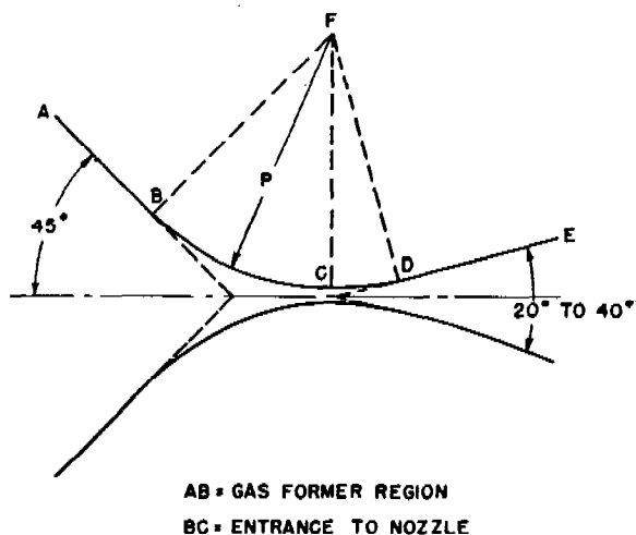
FIGURE 2. Geometry of nozzle and nozzle entrance area.
