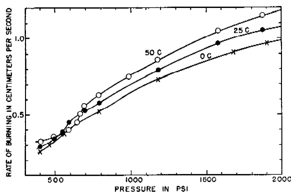
FIGURE 14. The burning rate of the propellant taken from a German 21-cm rocket.
