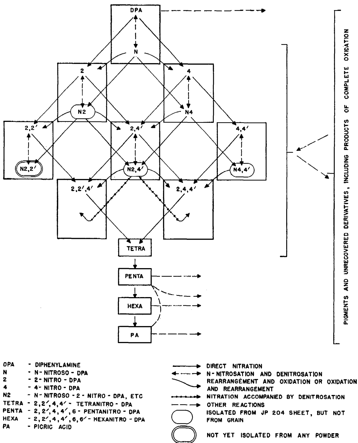
FIGURE 10. Possible relations among diphenylamine derivatives.
