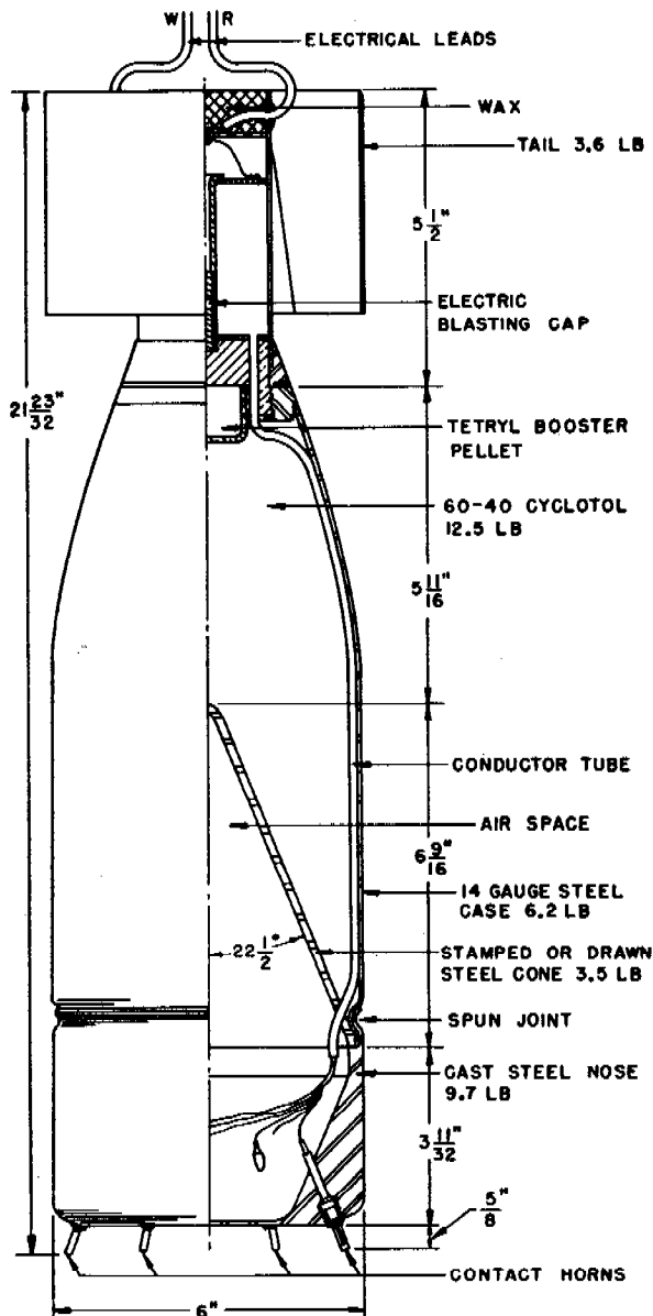
FIGURE 1. Antisubmarine shaped-charge bomb.
