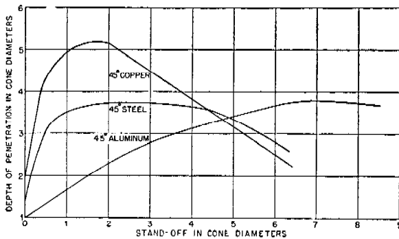
FIGURE 4. Depth of penetration versus stand-off, M6 steel and copper cones (2.36-in. diameter, 0.062-in. wall 1½-in. diameter aluminum 45° cones (0.064-in. wall), all charges steel confined.
