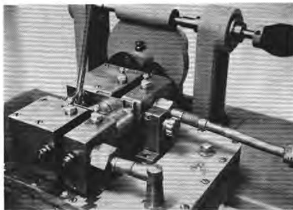
FIGURE 7. Small powder-rolling mill, close-up view.
