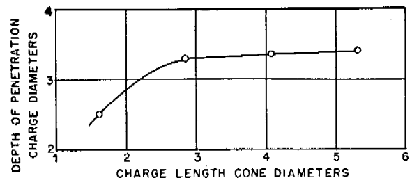
FIGURE 1. Depth of penetration versus charge length unconfined, 1\frac{3}{8} -in. diameter charges bearing M9A1 steel cones at 3-in. stand-off.
