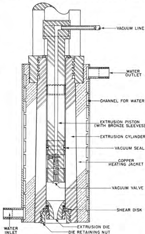
FIGURE 9. One-inch extrusion press, three-quarter size.
