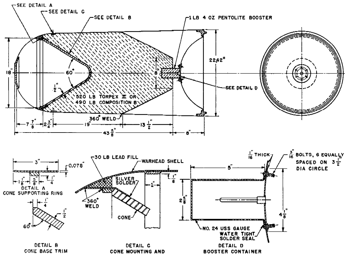
FIGURE 3. Shaped-charge torpedo warhead.
