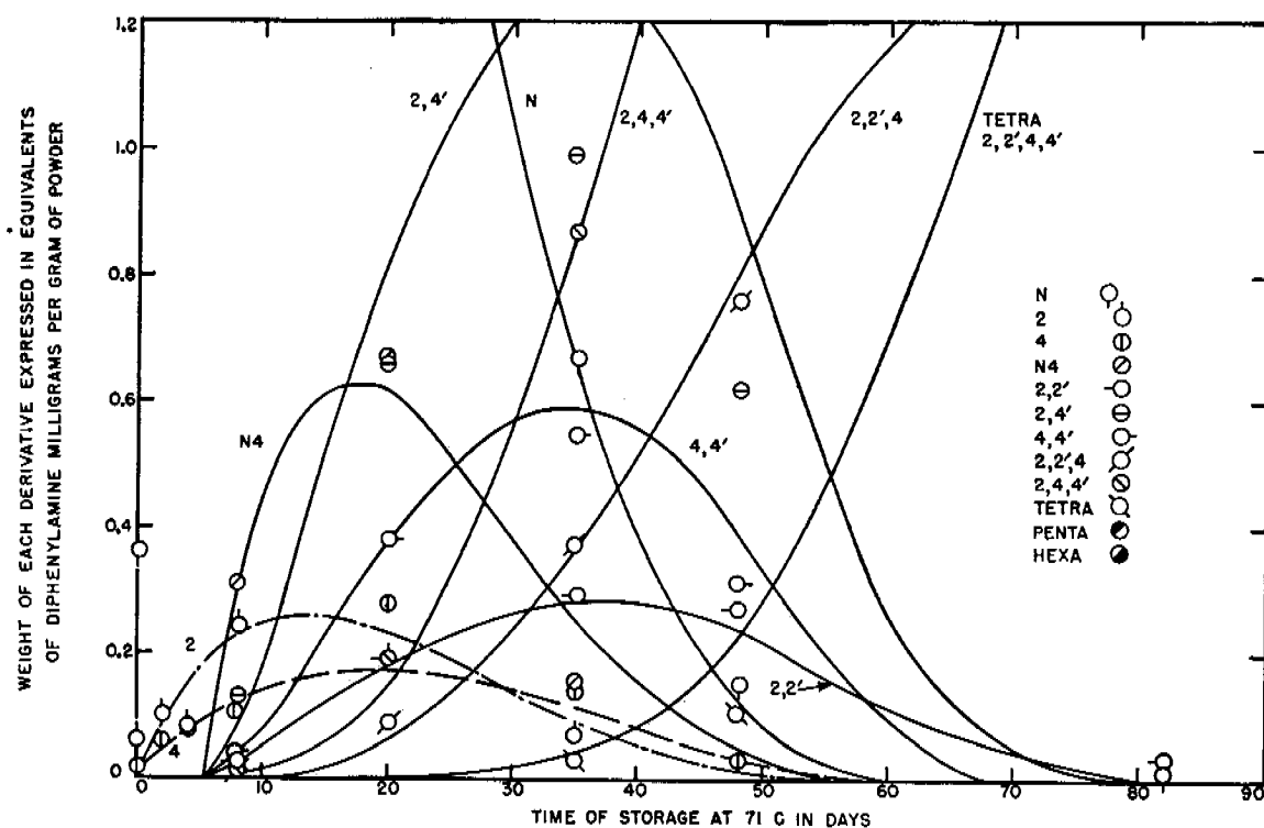
FIGURE 11. Transformation of diphenylamine in grains of ballistite JP 204 stored at 71 C. Comparison of theoretical curves with experimental data.
