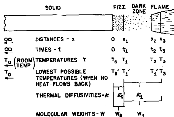
FIGURE 1. Schematic sketch of a stick of burning powder.
