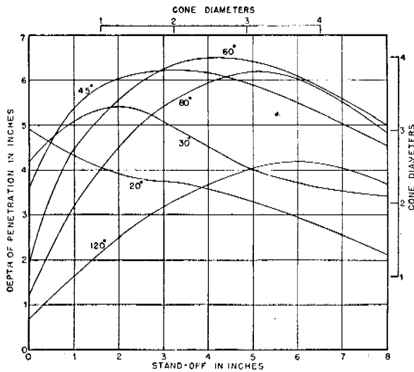
FIGURE 2. Effect of stand-off on depth of penetration, 1½-in. diameter unconfined cone charges.
