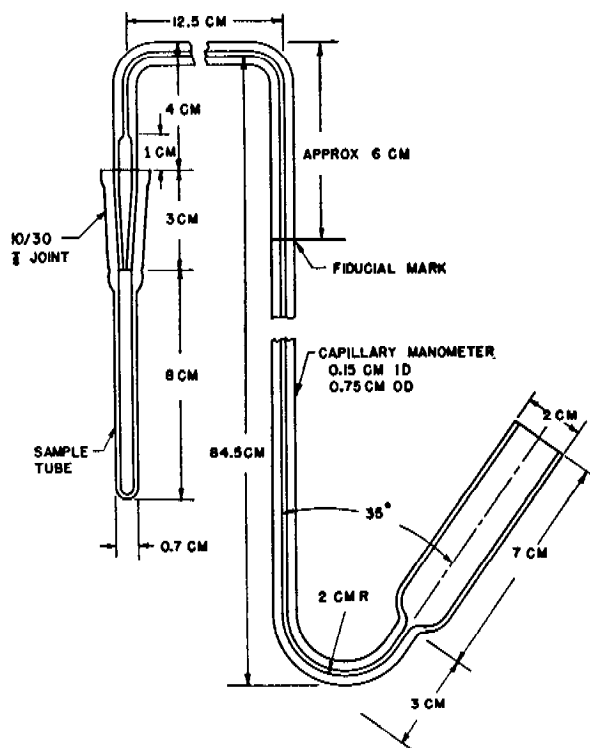
FIGURE 13. Standard-taper units for vacuum stability tests.
