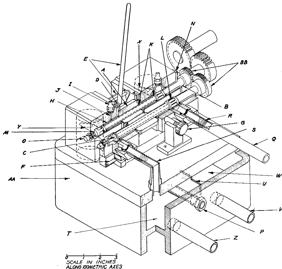
FIGURE 5. Small powder-rolling mill.
