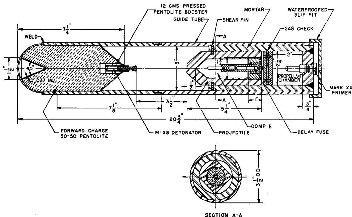
FIGURE 2. Antisubmarine shaped-charge follow-through bomb.
