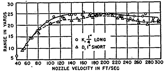
FIGURE 6. Comparison of effects of short 1-in. and long 1/4-in. straight sections on range of 7.8 per cent Napalm gels, unignited, issuing from a 1/8-in. nozzle.
