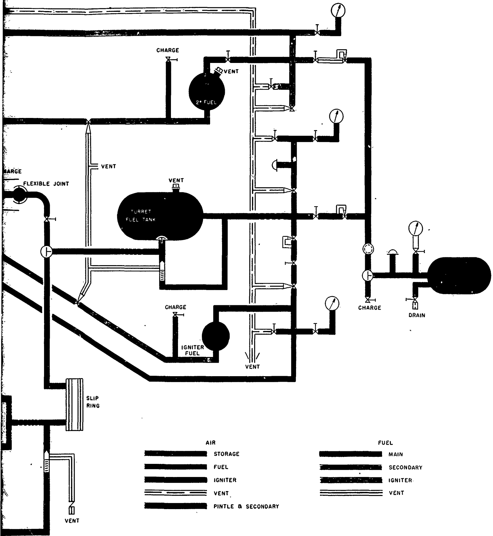
Sheet and wiring diagram for E13R1-13R2 flame thrower.
