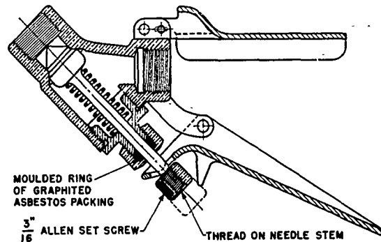
FIGURE 2. Cutaway of quick-opening Y valve for M1A1 portable flame thrower.
