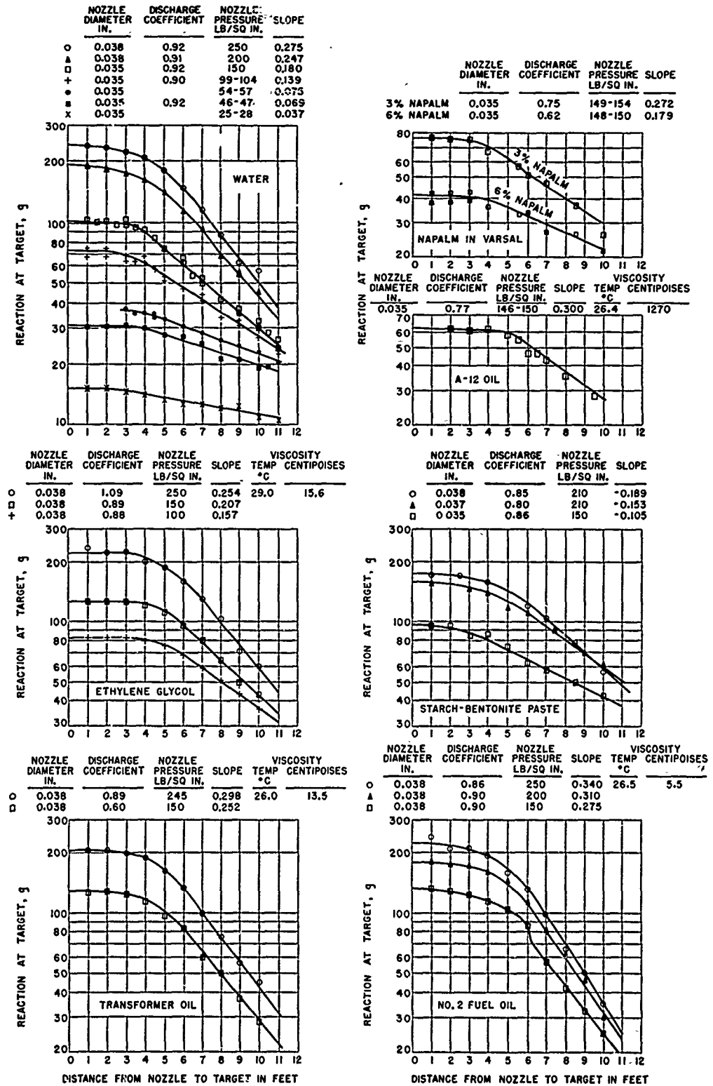
FIGURE 26. Jet reaction data.
