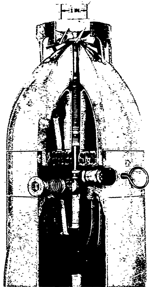
FIGURE 25. Detail of nose end of E9 incendiary bomb.
