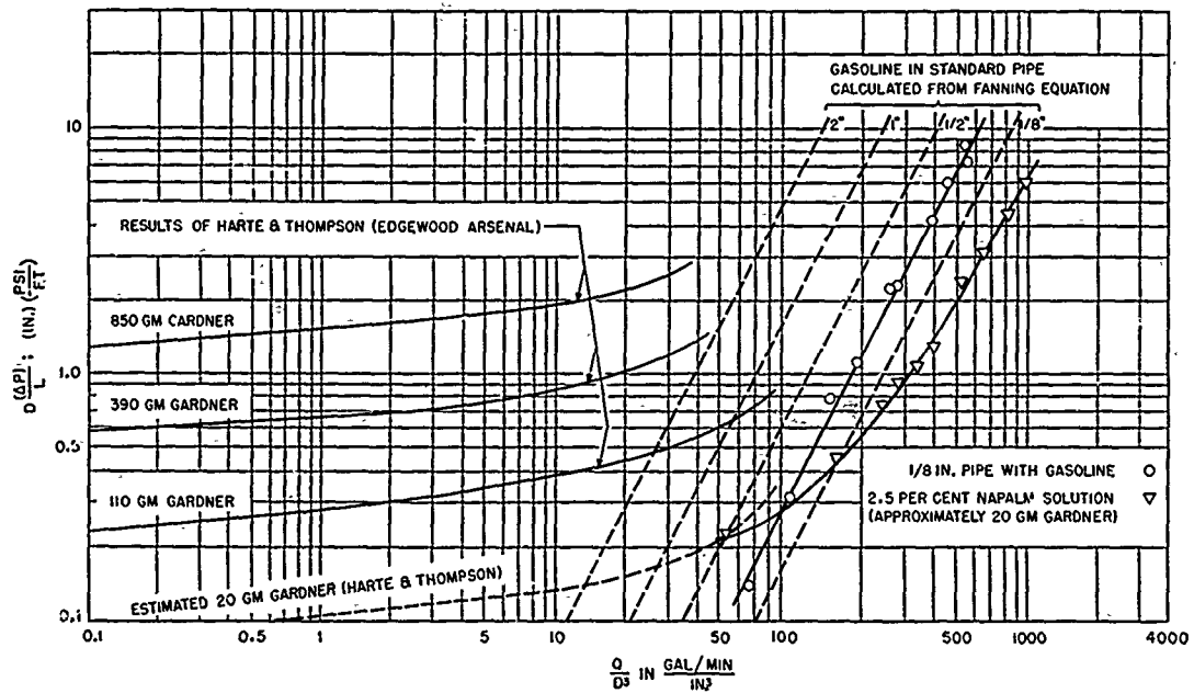
FIGURE 11. Flow characteristics of Napalm solutions in gasoline.
