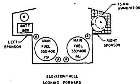
FIGURE 39. Flame-thrower tank T-33 (E20-20) in M4A3E2 medium tank showing schematic layout of hull.
