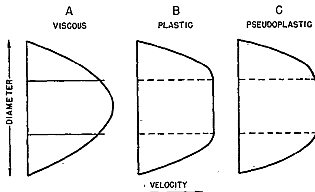
FIGURE 2. Various types of flow.
