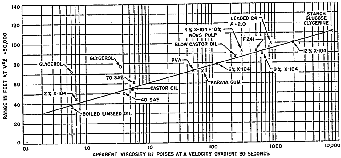
FIGURE 24. Range versus apparent viscosity for 1/8-in. nozzle.
