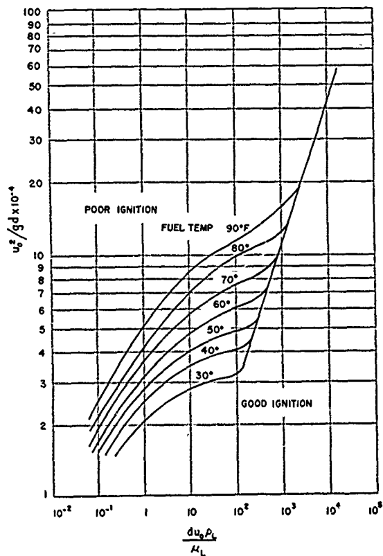
FIGURE 30. Relation among Reynolds number, Froude number, and fuel temperature, defining regions of good and poor ignition.
