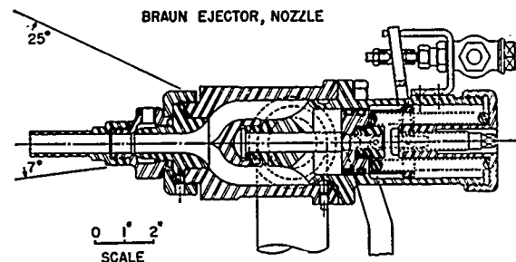
FIGURE 21. Cutaway of Braun ejector nozzle showing pintle valve in open position.
