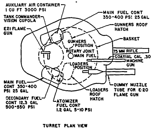
FIGURE 40. Flame-thrower tank T-33 (E20-20) in M4A3E2 medium tank showing schematic layout of turret.
