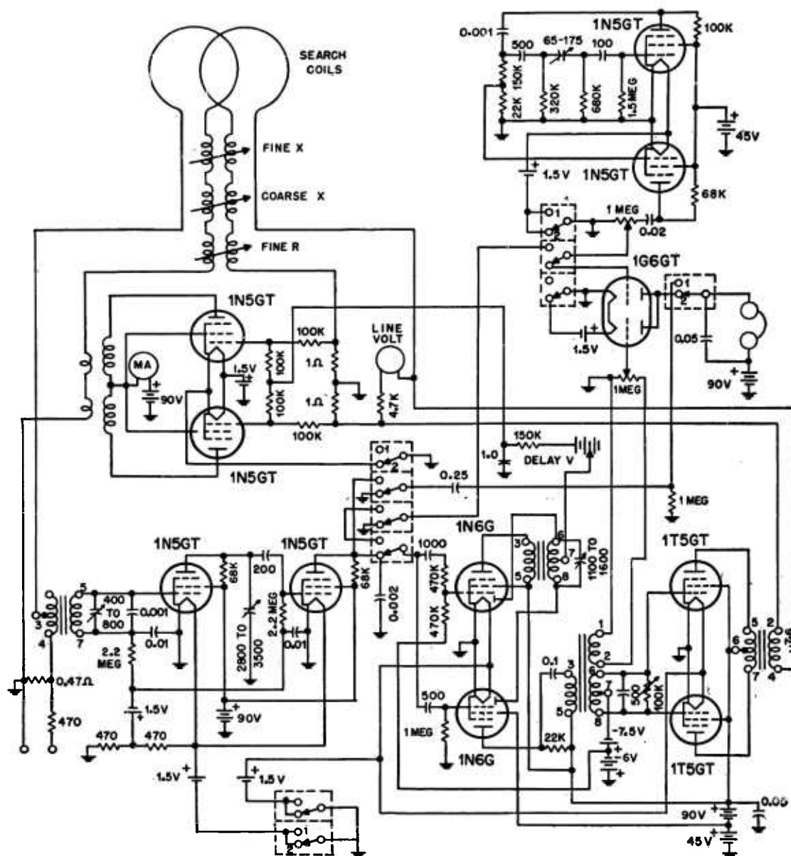
FIGURE 5. Circuit diagram.
