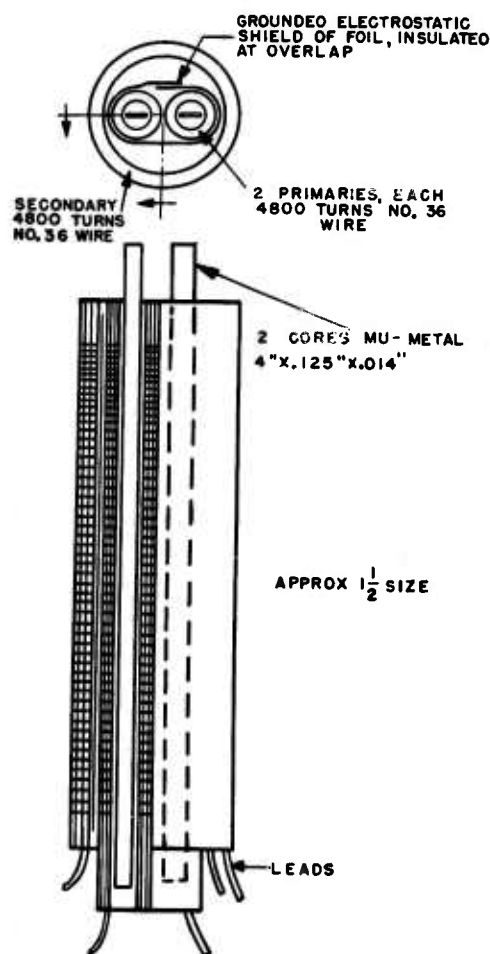
FIGURE 5. Magnetic-detector coil.
