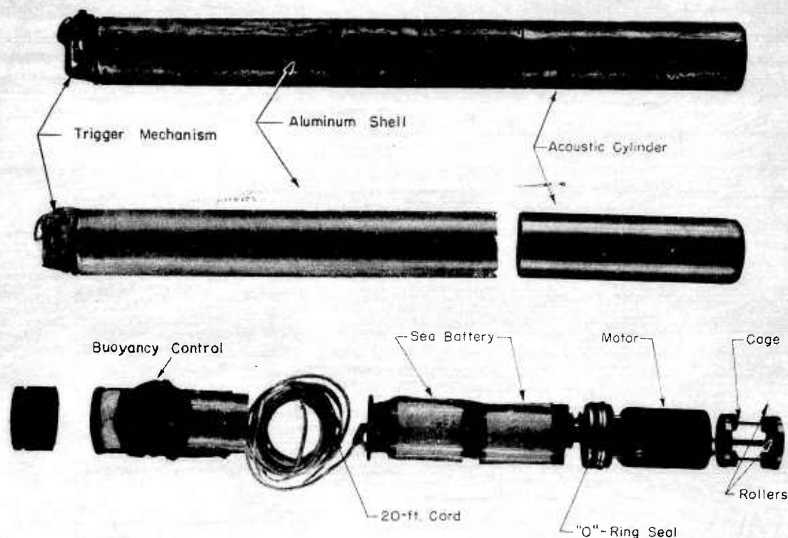
FIGURE 6. NAE sound beacon Mk 1.
