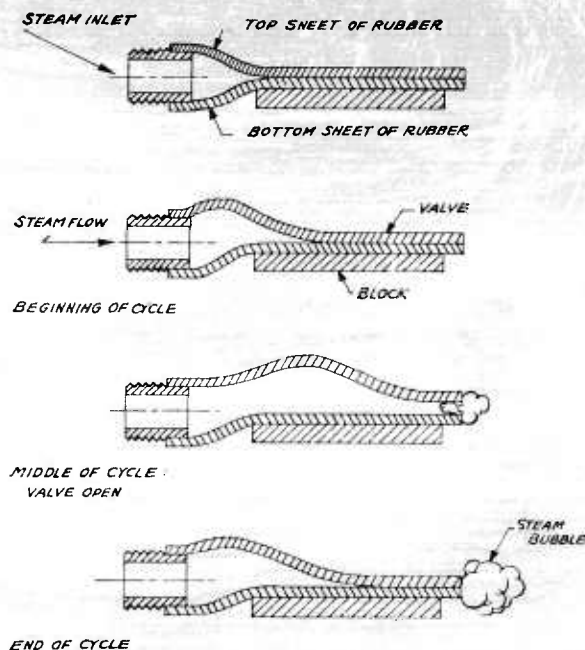
FIGURE 5. Diagram of razzzer operation.
