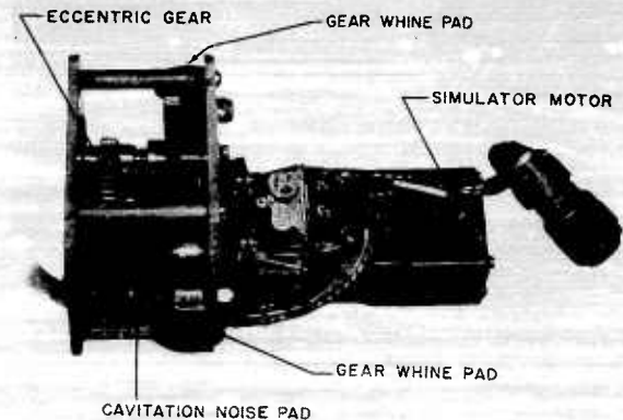
FIGURE 27. Self-noise simulator mechanism.
