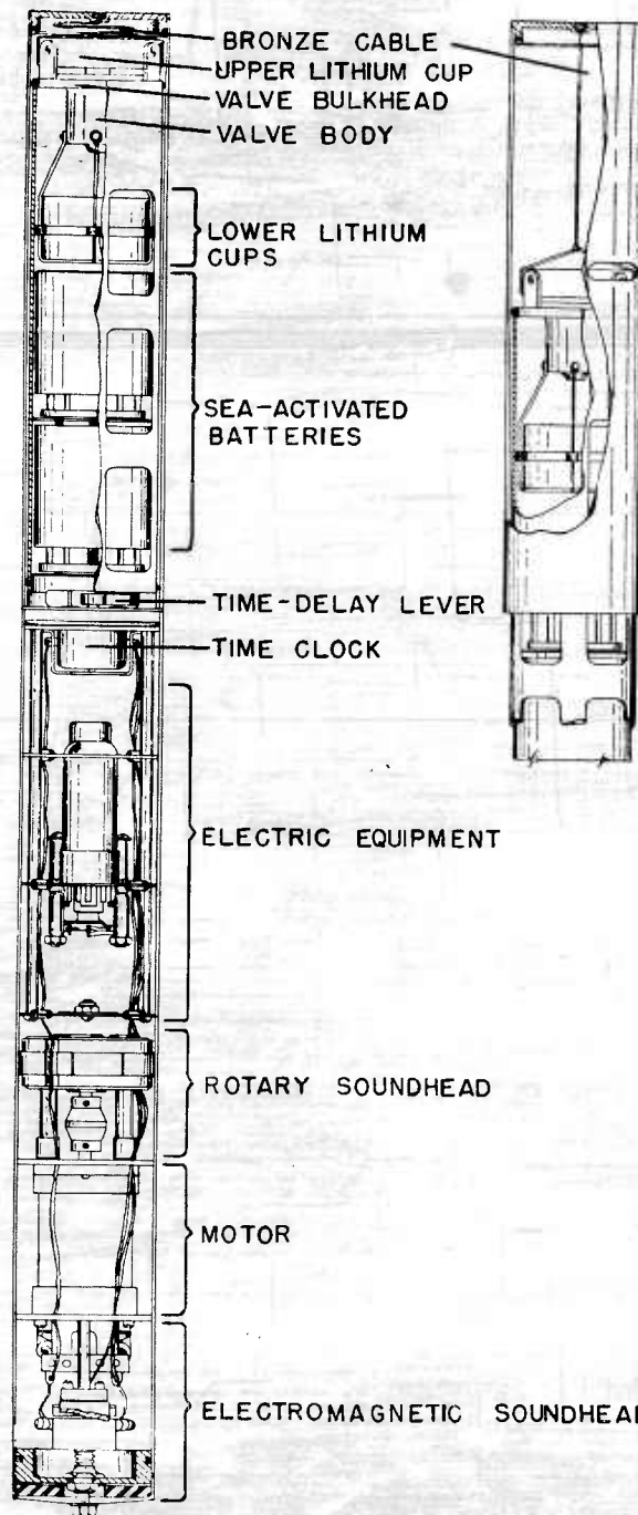
FIGURE 31. Drawing of XNAG sound beacon.
