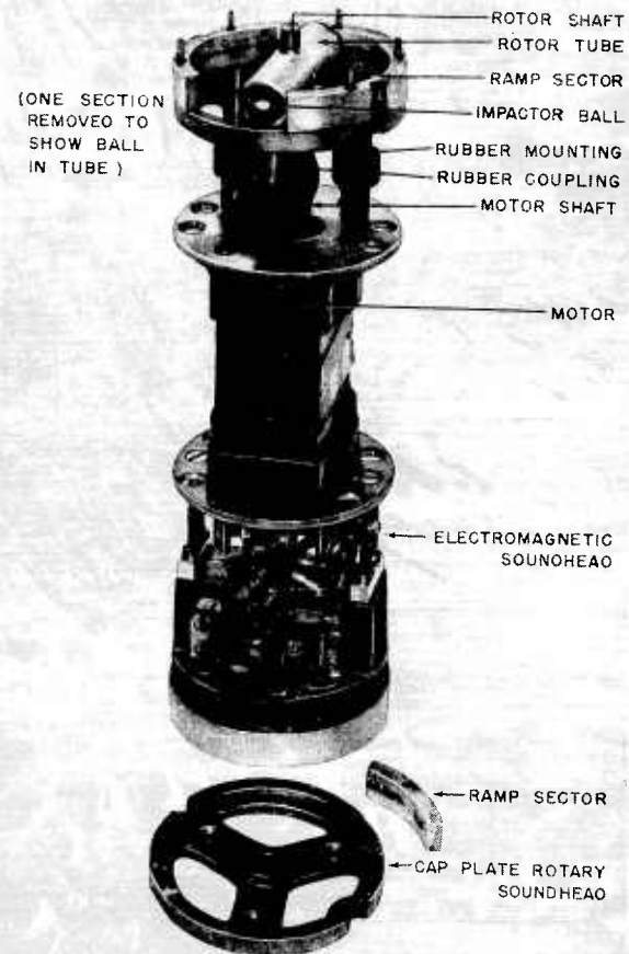
FIGURE 33. XNAG ball-impactor soundhead and motor.
