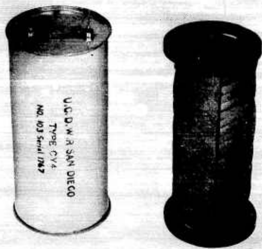
FIGURE 4. NAC crystal projector.
