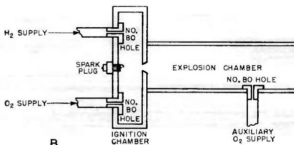
FIGURE 8. Photograph and drawing of hydrogen-oxygen noisemaker.
