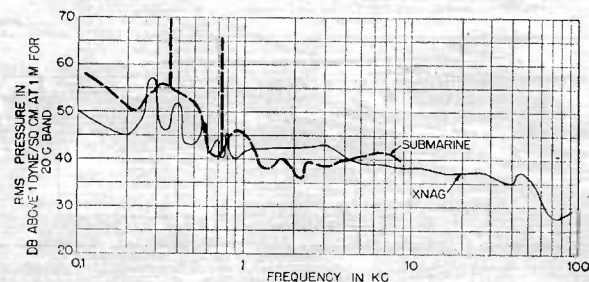
FIGURE 36. Output of XNAG compared with USS Spot at 6 knots.
