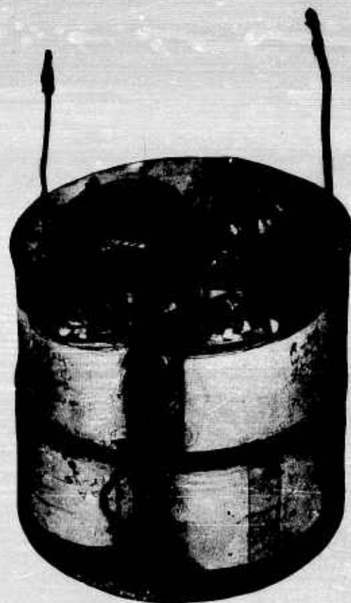
FIGURE 5. Burgess 24-volt sea battery.
