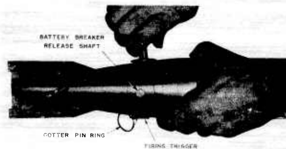
FIGURE 13. NAD-3 afterbody.
