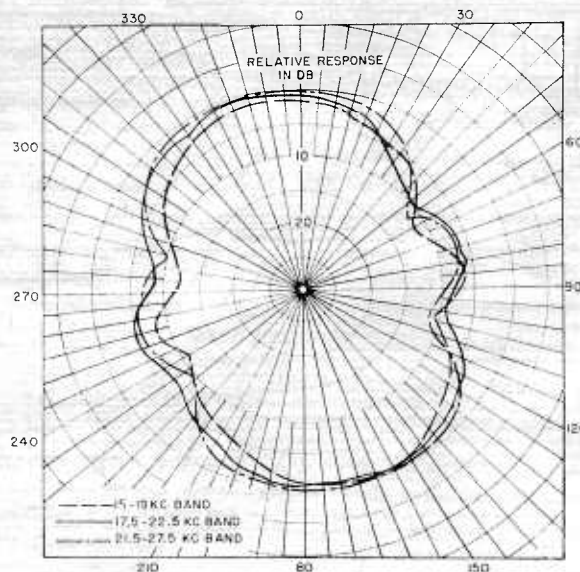
FIGURE 6. Horizontal directivity pattern of NAC.
