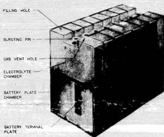
FIGURE 7. Edison I-type 8-cell battery.
