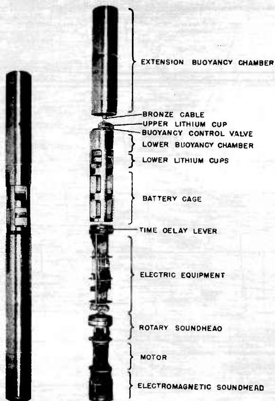
FIGURE 30. Construction of XNAG sound beacon.
