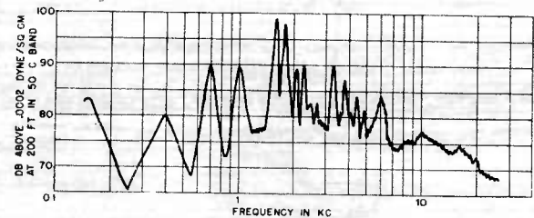
FIGURE 28. Frequency characteristic of NAD-6 noise output.
