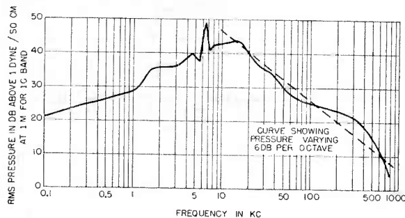
FIGURE 8. Frequency characteristic of NAE Mk 1.
