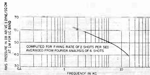
FIGURE 25. Frequency characteristic of pepper signal.
