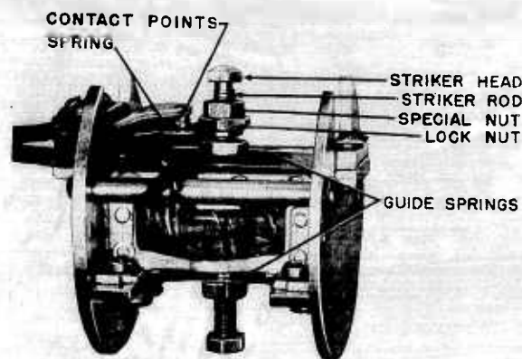
FIGURE 18. Striker-impactor soundhead.
