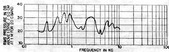
FIGURE 24. Frequency characteristic of roller impactor Model 2.
