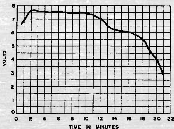
FIGURE 4. Discharge characteristic of Burgess 5cc133 sea battery.
