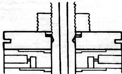
FIGURE 22. Top plate assembly.
