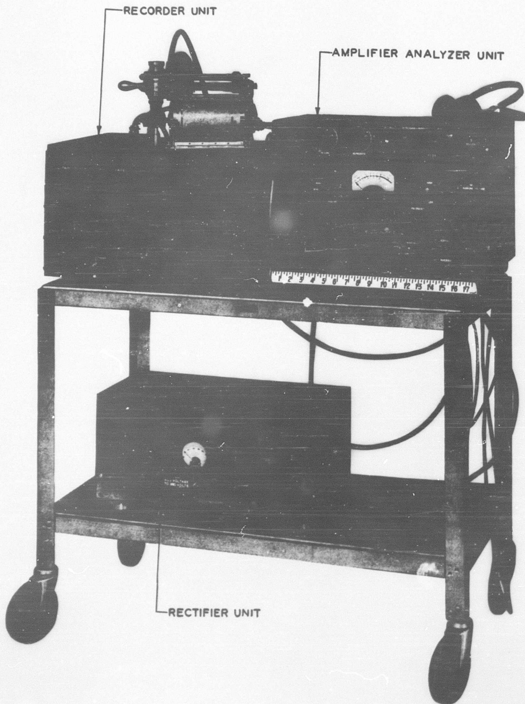
FIGURE 22. Sound spectrograph (D-165529) on a "push-around."
