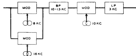
FIGURE 7. One form of superposition decoding.
