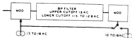
FIGURE 2. Band-shift filter; an important decoding tool.
