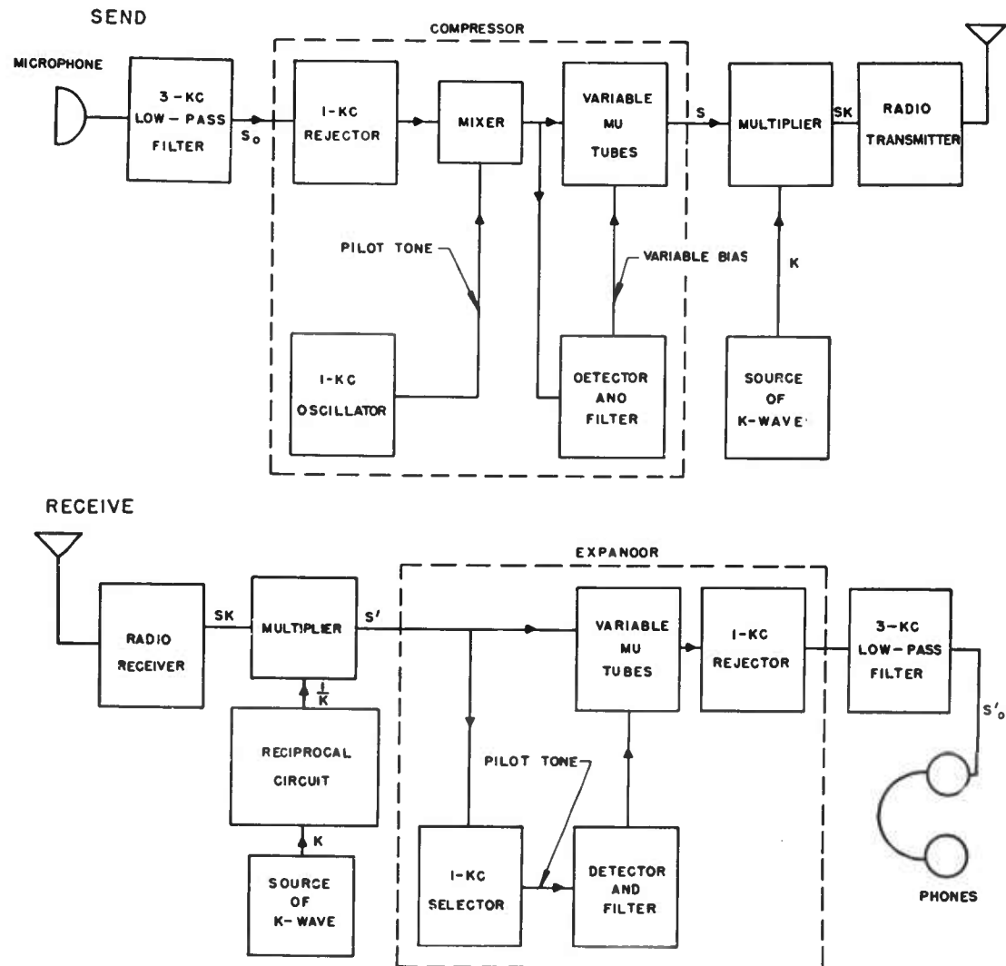
FIGURE 2. Block diagram showing compandor in RCA-Bedford privacy system.
