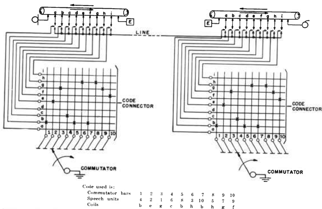
FIGURE 5. TDS coding connections. Transmit machine codes on "reproduce," while receive machine decodes on "record."
