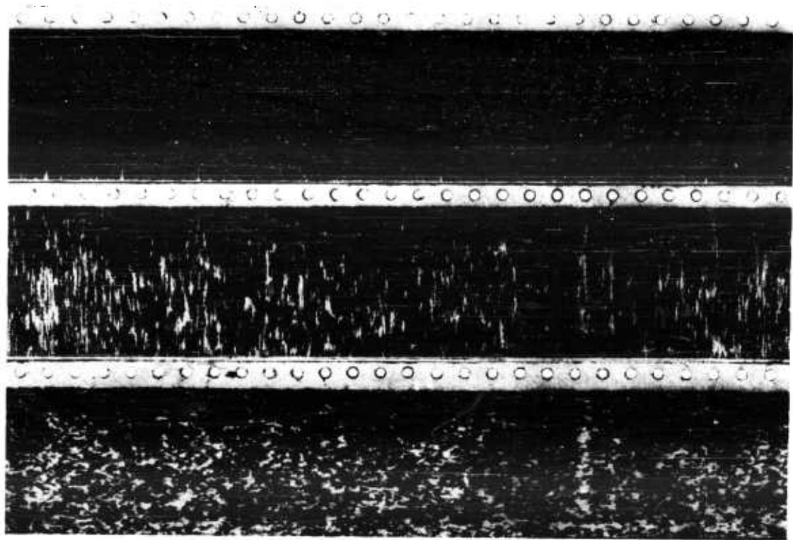
FIGURE 36. Thermal noise as example of steady sound. Two upper records made with wide filter, two levels, 12-db apart. Lower spectrograph made with narrow filter. These are 11-kc records.
