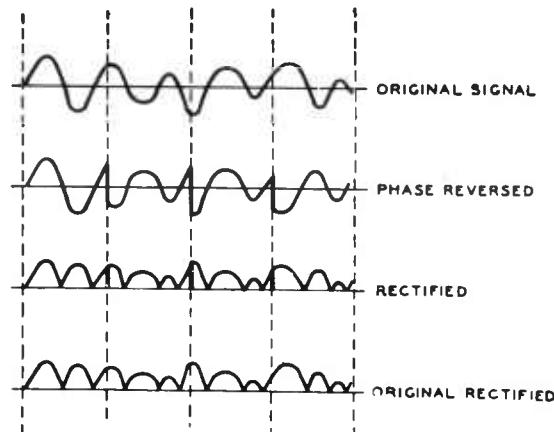
FIGURE 6. Action of rectifier, useful in breaking down multiplication scrambles.
