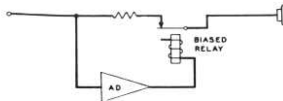
FIGURE 9. Use of relay to disconnect receiver from line during heavy bursts of noise.
