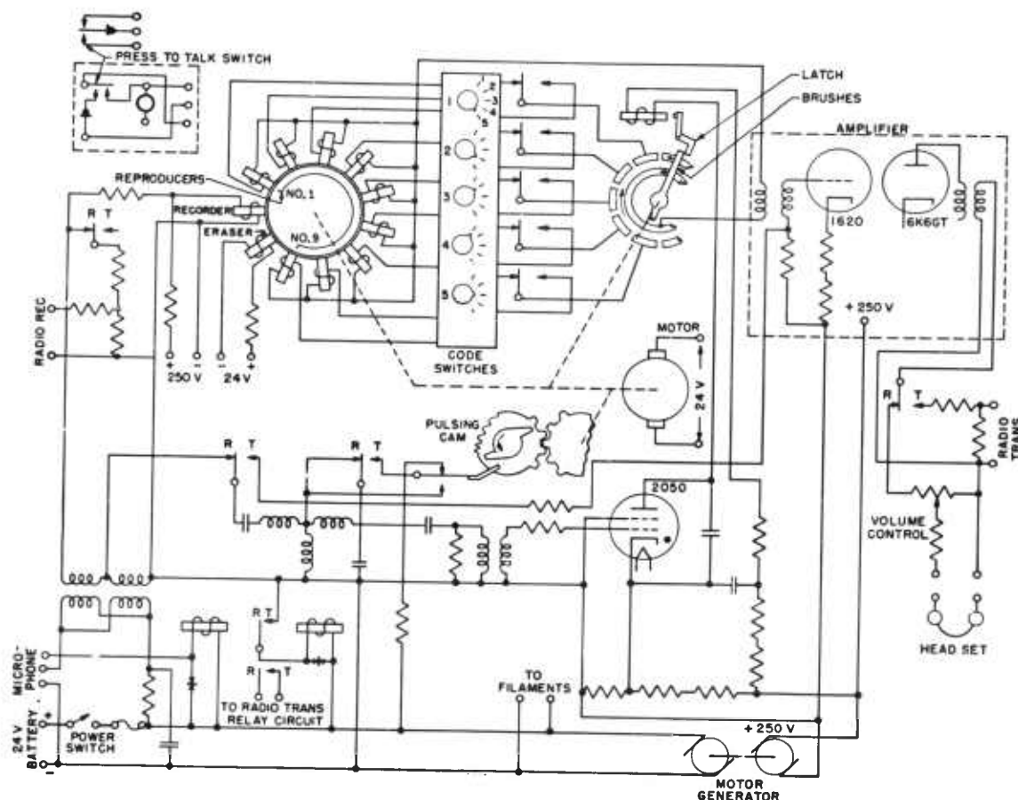
FIGURE 4. Simplified circuit diagram of C-1 TDS system.
