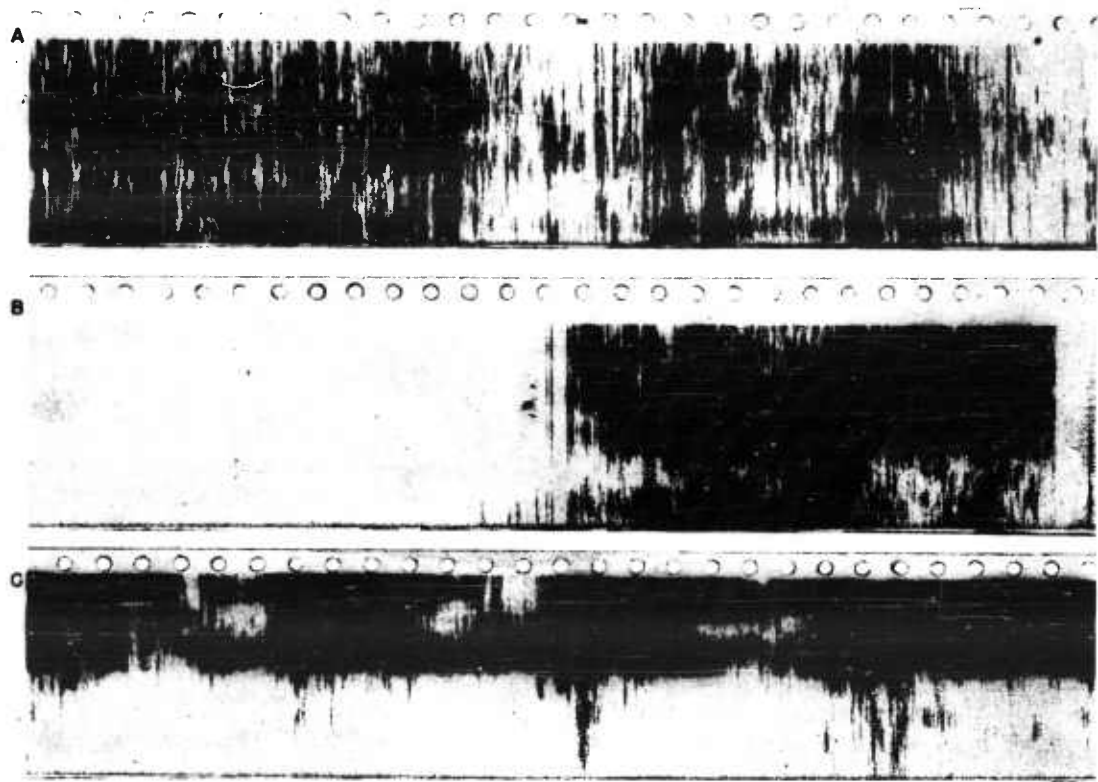
FIGURE 33. Spectrographs showing that sounds exist in high-frequency region. These are 11-kc, 1,000-cycle filter records. A, sound of crumpling paper; B, sound of tearing cloth; C, jingling keys.
