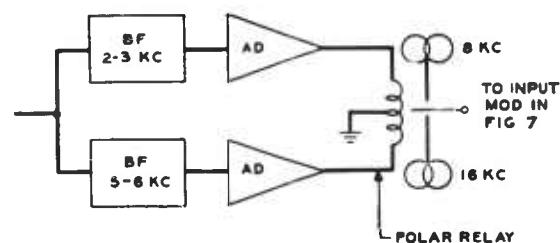
FIGURE 11. Automatic decoding system depending upon energy-frequency distribution.
