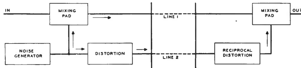
FIGURE 16. Noise masking requiring use of two telephone lines.
