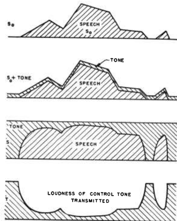
FIGURE 3. Envelopes of speech and tone in comparator.
