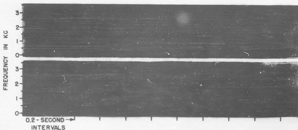
FIGURE 24. Spectrograms of normal speech, words being "one, two, three, four, five, six." In this case, spectrograms are somewhat smaller than normal size due to photographic reduction and some trimming at ends.
