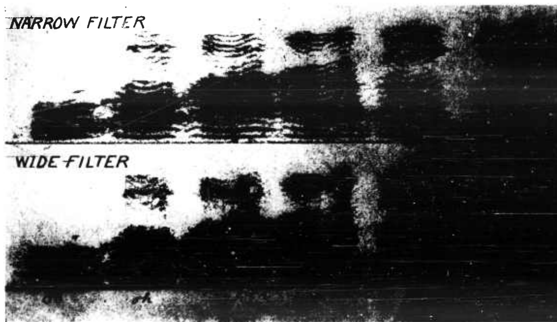
FIGURE 38. Patterns of vowel sounds showing effect of wide and narrow filters.
