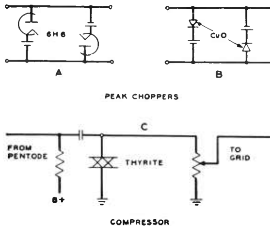
FIGURE 4. Elementary circuits of peak choppers and compressor.
