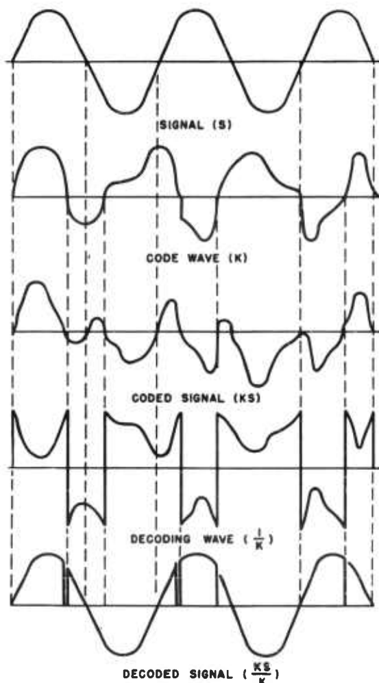
FIGURE 13. Example of multiplication system.
