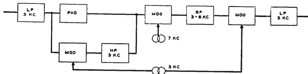
FIGURE 5. System involving re-entrant inversion.
