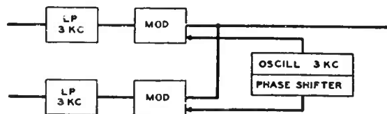
FIGURE 3. Split-phase multiplex used as two-channel system.
