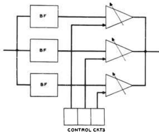
FIGURE 15. Level modulation system in which speech is first divided into subbands, each of which is subjected to level changes.
