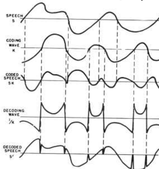
FIGURE 1. Coding and decoding processes involved in RCA-Bedford multiplication privacy system.
