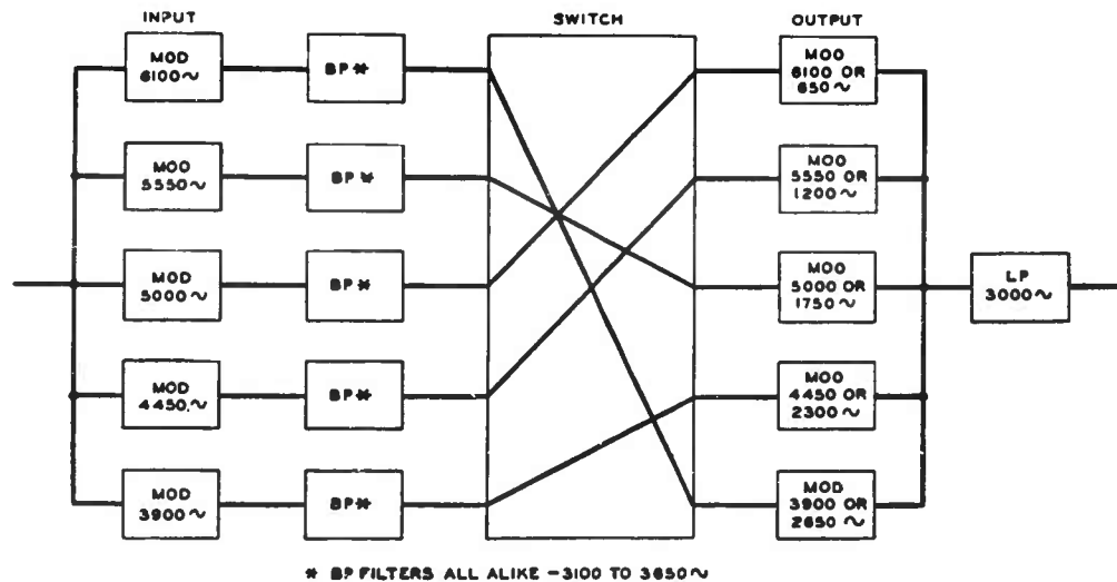
FIGURE 6. One form of split-band system in commercial use.
