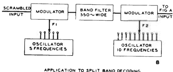
FIGURE 19. Band-shift detector.
