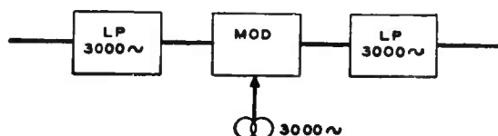
FIGURE 2. Simple inversion produced by single modulation.
