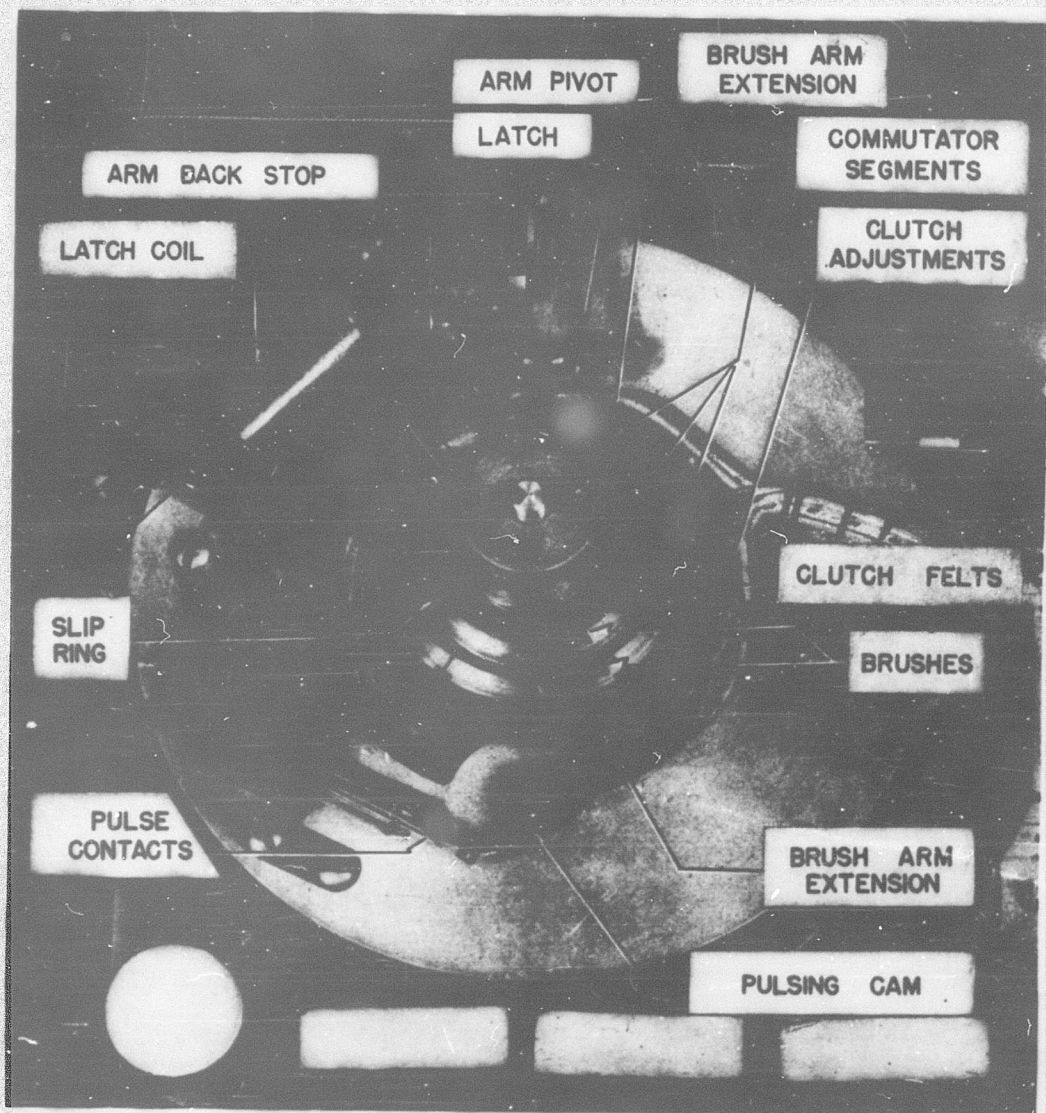
FIGURE 3. Commutator details.
