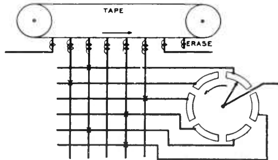
FIGURE 9. One form of time division scrambling [TDS].
