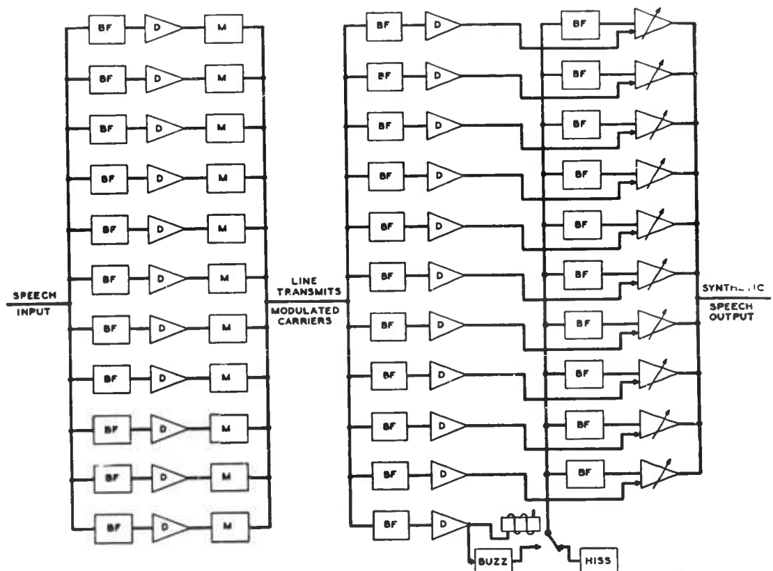
FIGURE 18. Vocoder system which may be made basis of privacy systems of various kinds.
