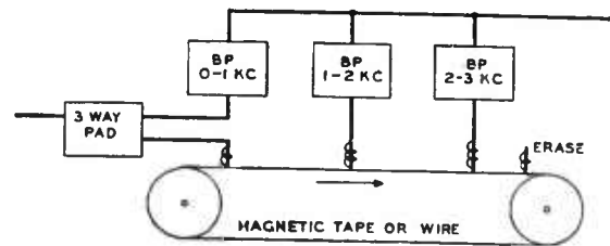
FIGURE 8. Variable subband delay system using magnetic tape.
