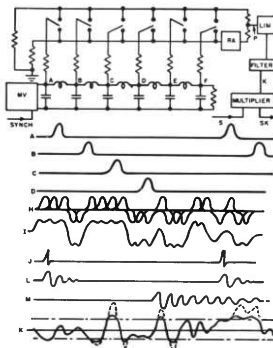
FIGURE 4. Generation of coding wave K .
