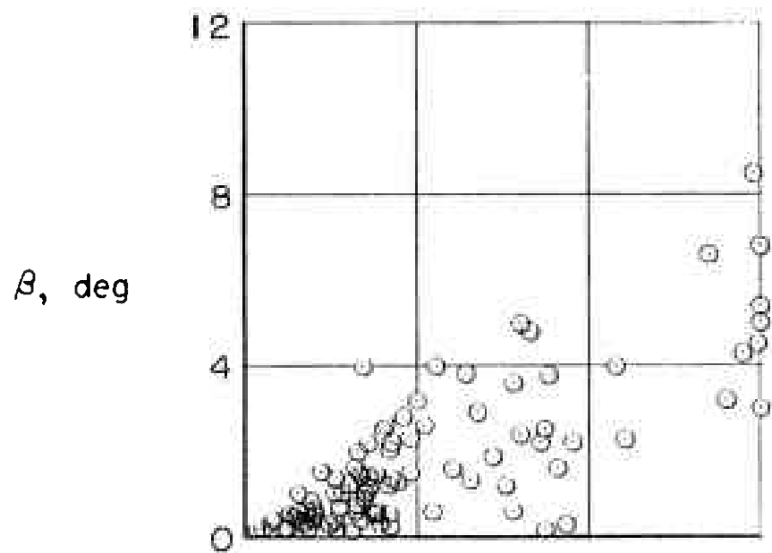
(c) Angle of sideslip.
