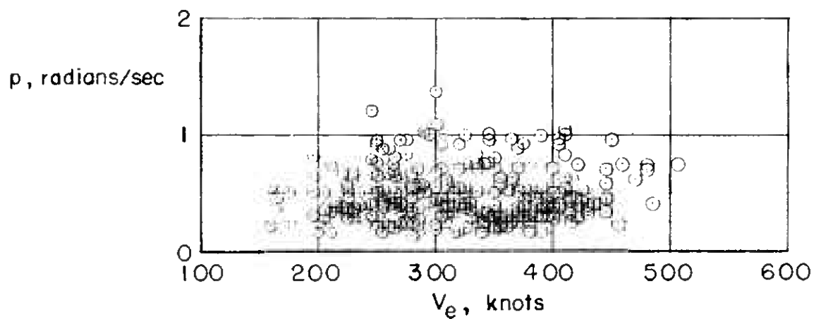
(b) Rolling velocity.
