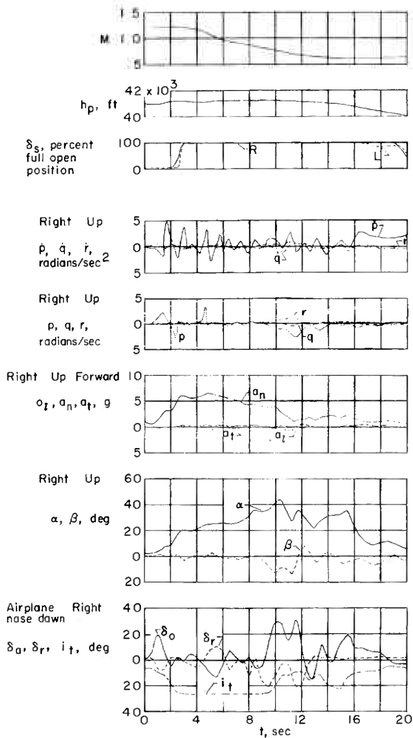
Figure 6.- Time history of an extreme evasive maneuver as performed in air combat maneuvers.
