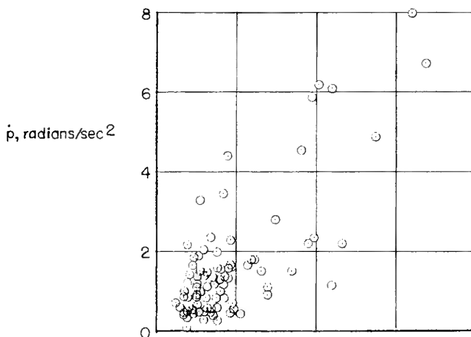
(a) Rolling acceleration.
