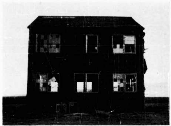
FIGURE 184. Barracks 1 after Test 4; east elevation
