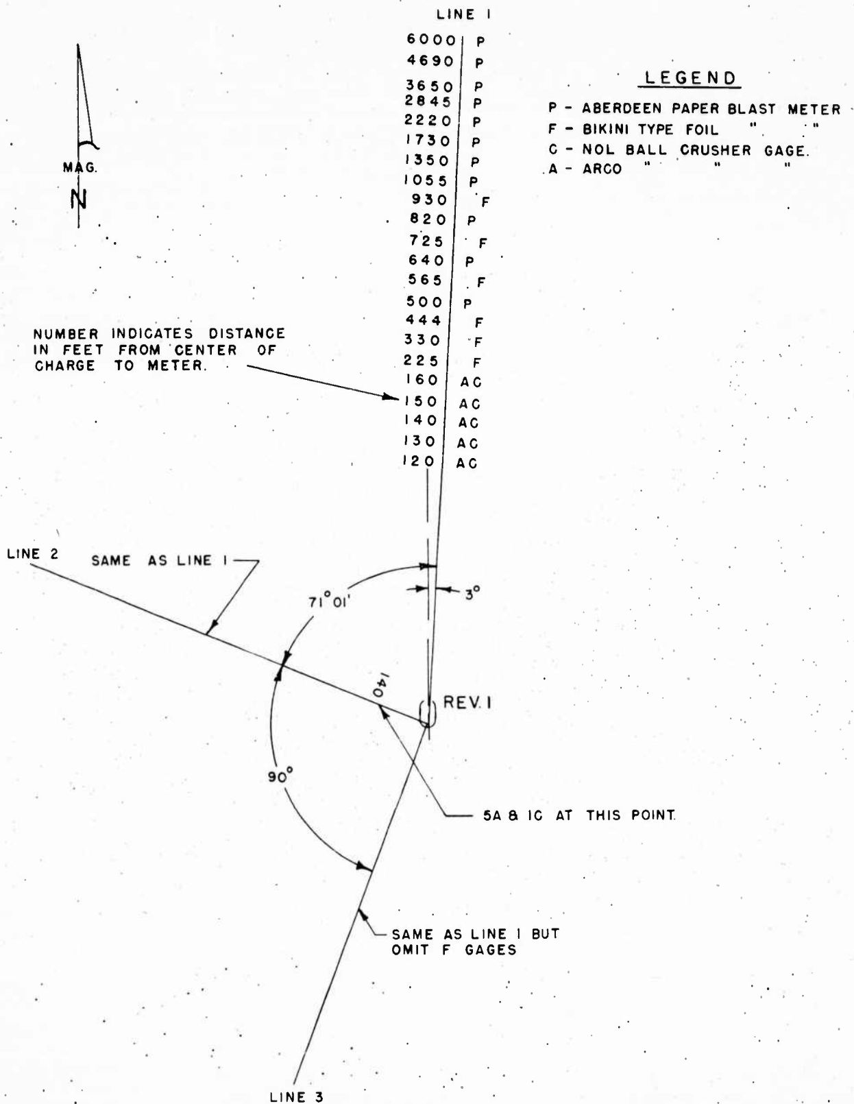
FIGURE 22. Blast Meter Layout, Test 4
