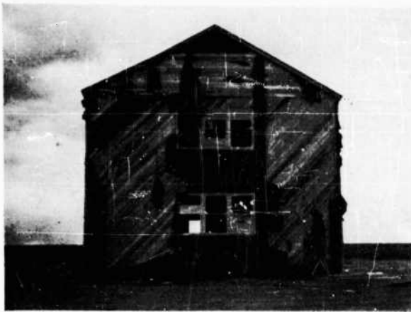
FIGURE 183. Barracks 1 after Test 4; north elevation
