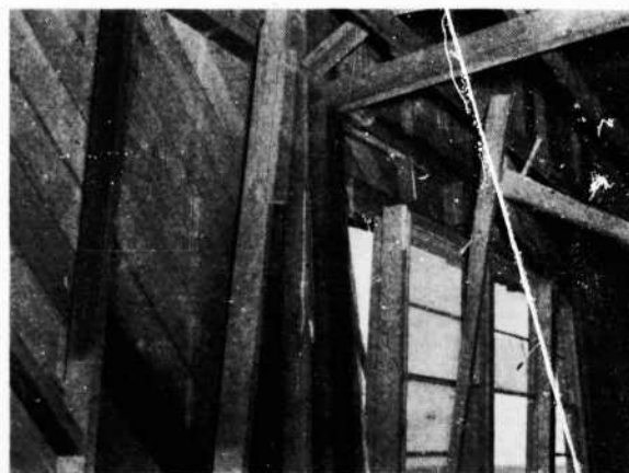
FIGURE 127. Broken and displaced studs, north wall, second story, Barracks 2 after Test 2
