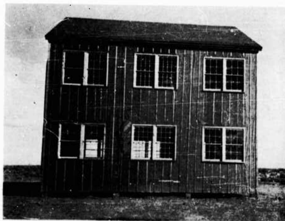
FIGURE 194. Barracks 3 after Test 4; west elevation
