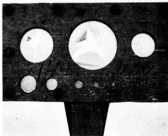
FIGURE 25. Close-up of an Aberdeen paper blast meter, after blast
