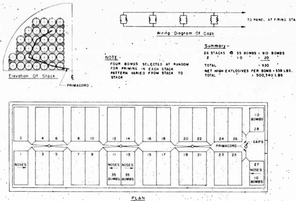
FIGURE 14. Stacking and Priming Plan, Igloos D and E, Tests 1 and 2
