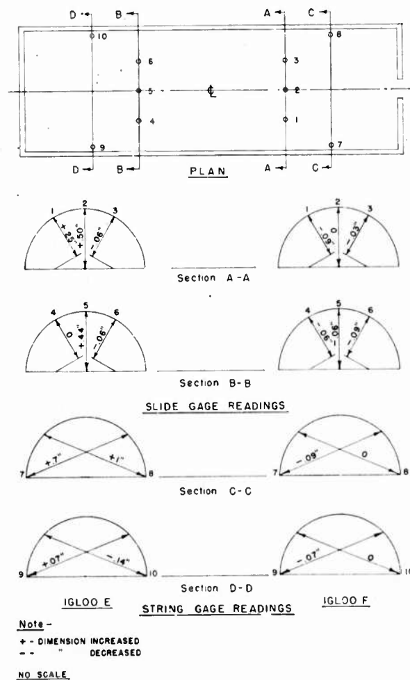
FIGURE 41. Permanent Changes in Internal Dimensions of Igloos E and F as Measured by Deflection Gages, Test 1
