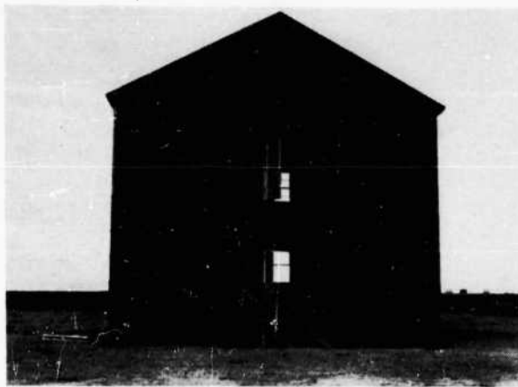
FIGURE 157. South elevation of Barracks 2 after Test 3
