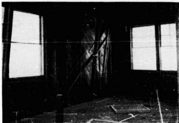
FIGURE 70. Interior, Barracks 2 after Test 1. Ground floor, northeast corner, showing broken and displaced studding and brace
