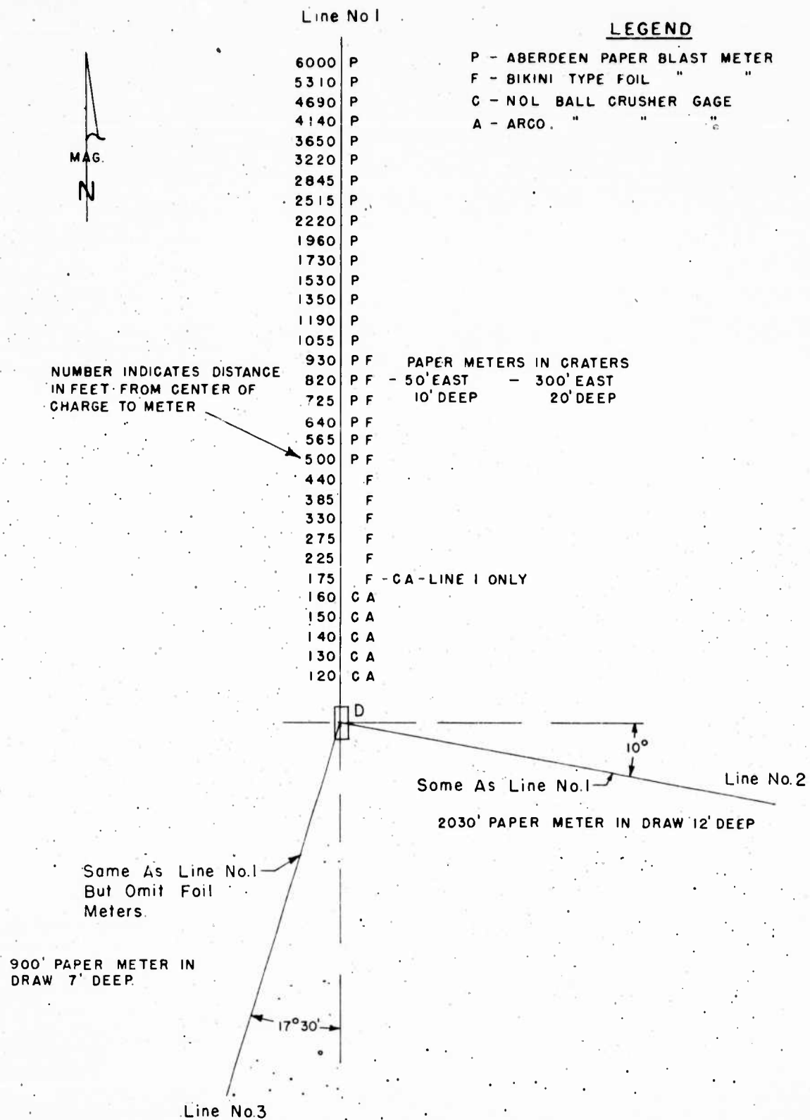
FIGURE 19. Blast Meter Layout, Test 1
