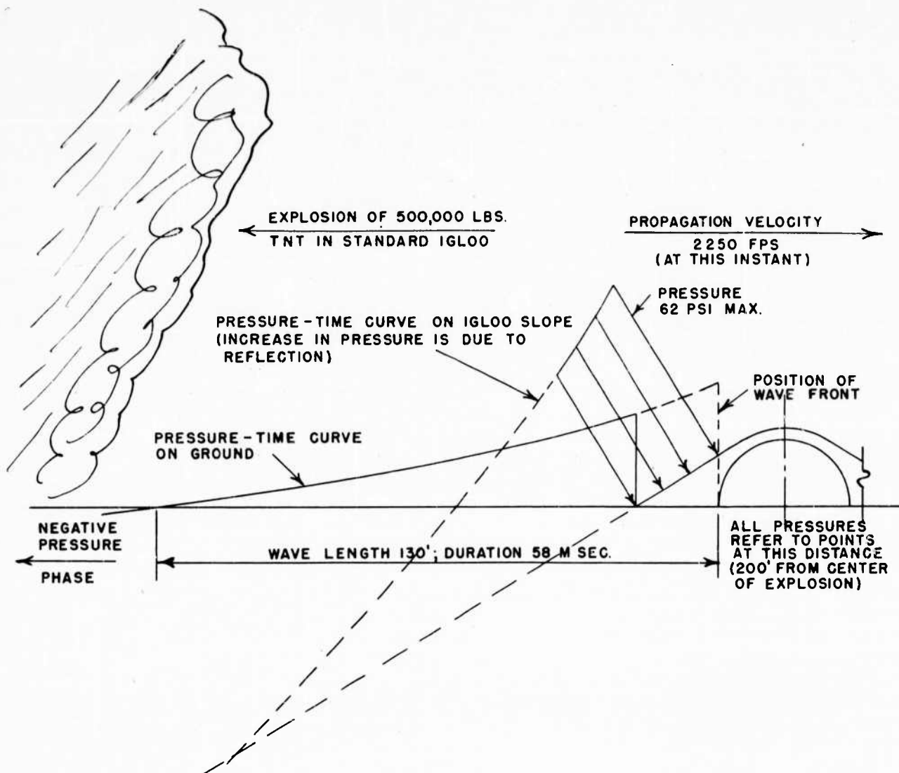
FIGURE 224. Blast loading on near side of igloo
