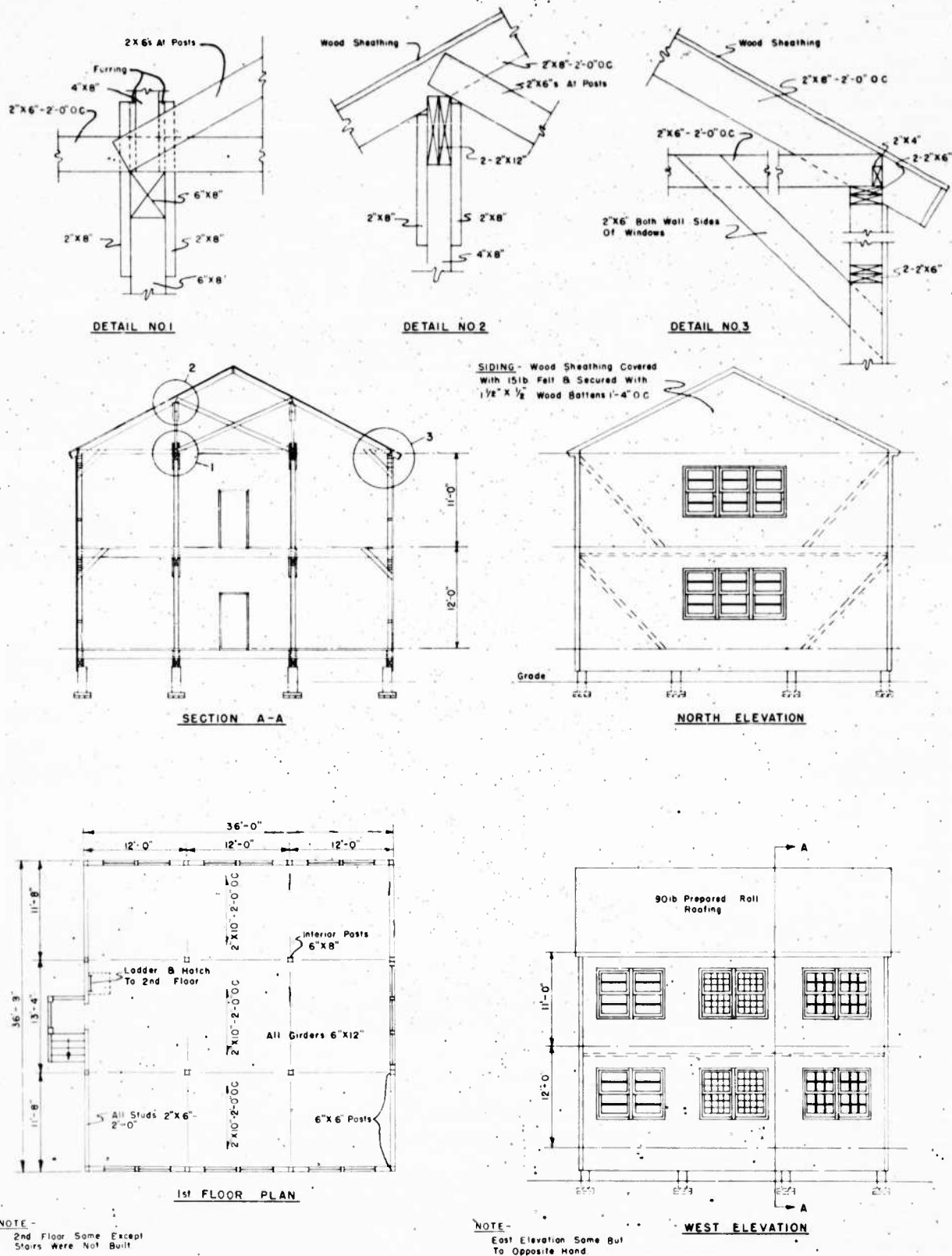
FIGURE 10. Construction Plans, Test Barracks .
