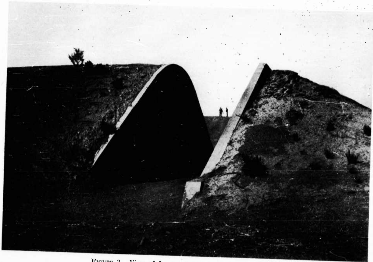
FIGURE 3. View of front end and door barricade, Igloo D
