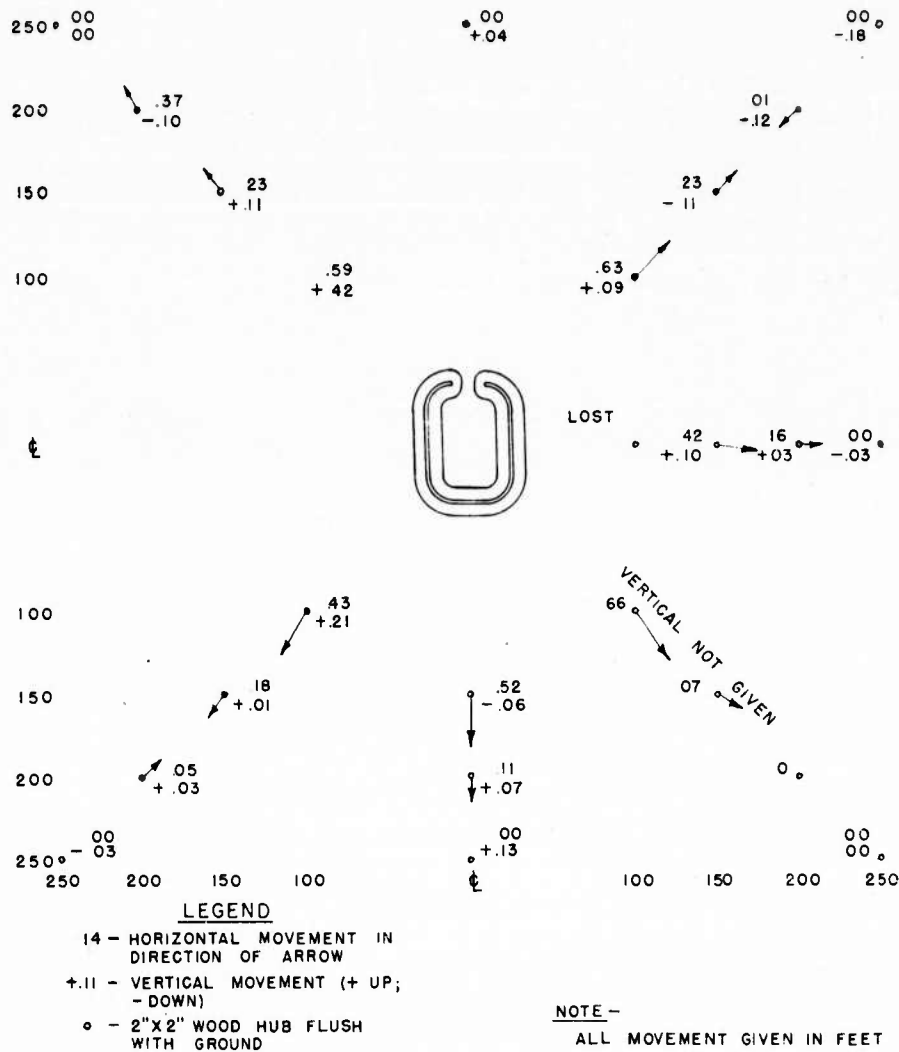
FIGURE 180. Permanent Horizontal and Vertical Earth Displacement, Revetment No. 1, Test No. 4
