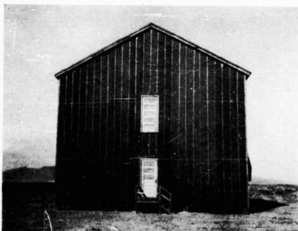
FIGURE 214. South elevation of Barracks 3 after Test 5
