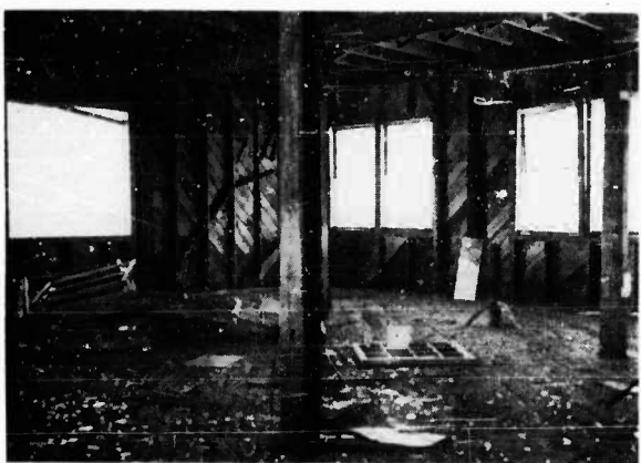
FIGURE 64. Interior of Barracks 1 after Test 1. Ground floor, looking northeast
