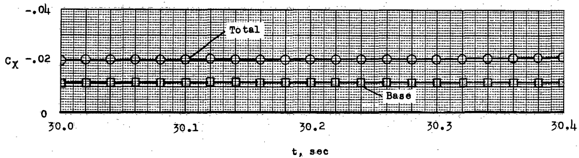
(c) Total axial-force and base axial-force coefficients.
