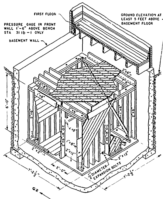
Fig. 1.4—Sketch of basement corner-room shelter.
