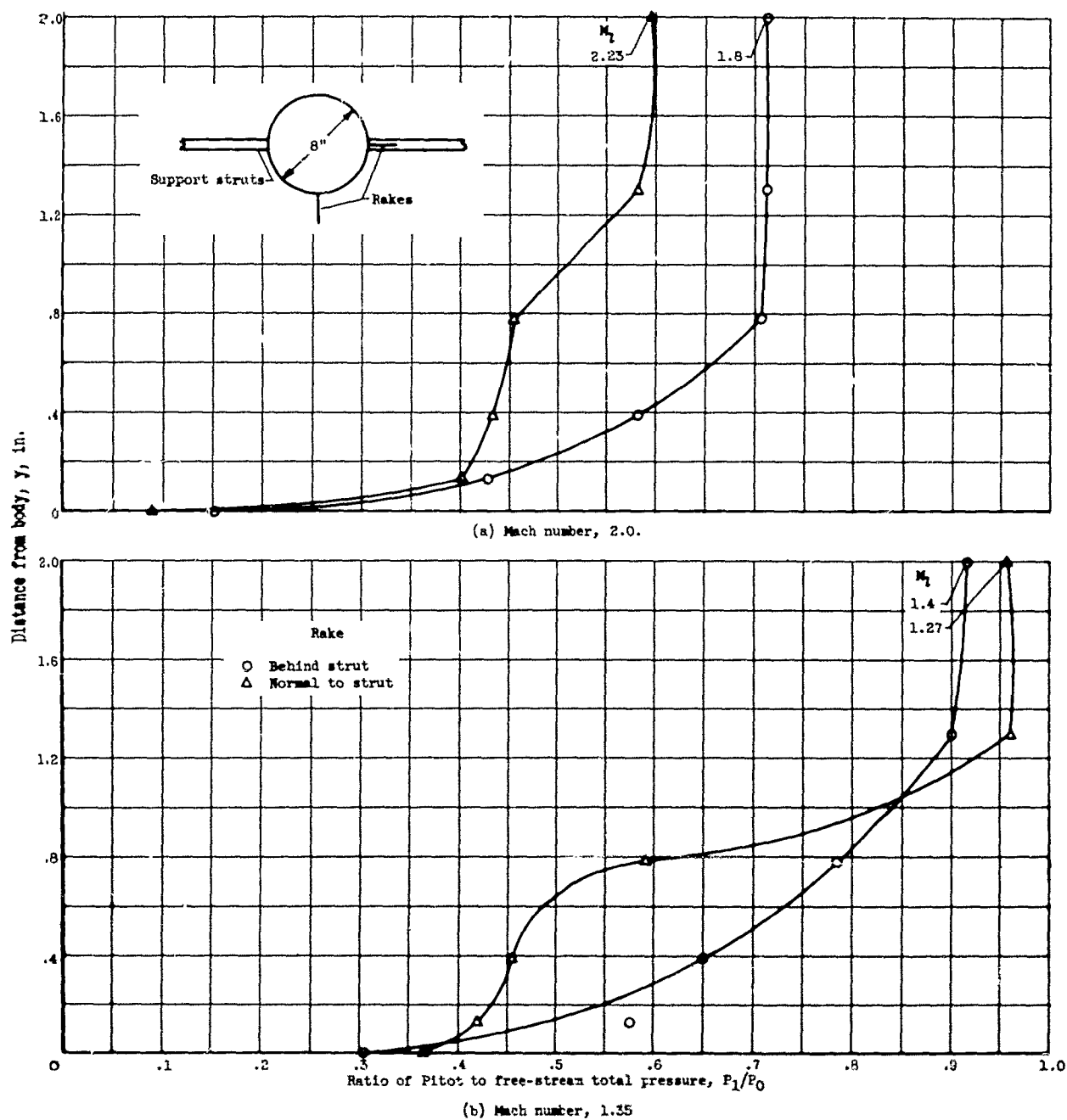
Figure 3. - Pitot pressure profiles upstream of boattail.
