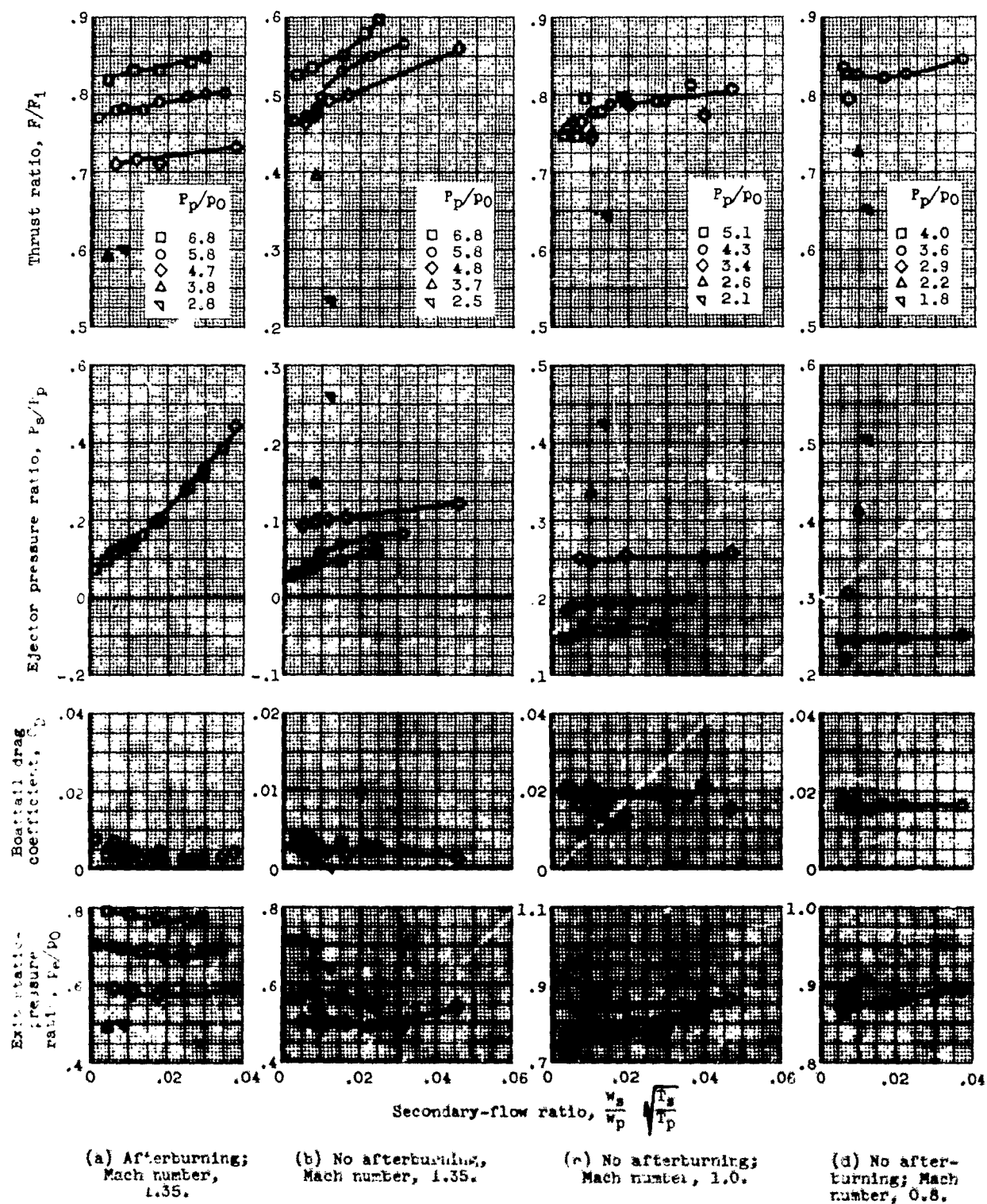
Figure 9. - Performance of ejector 4.
