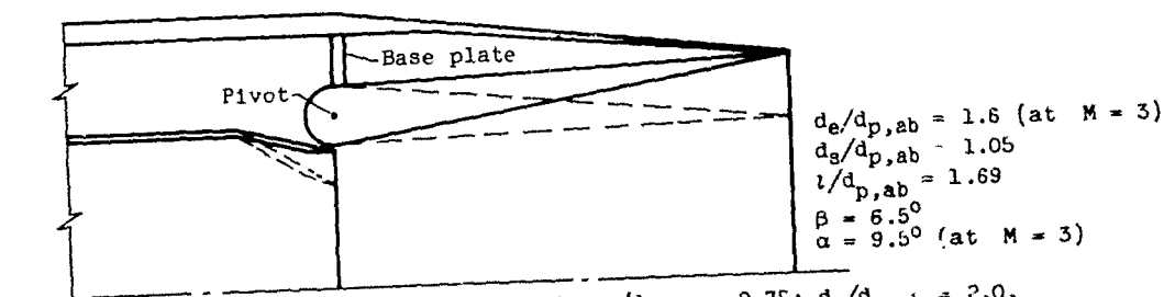
(g) Ejector 8: d_{p,nb}/d_{p,ab} = 0.75 ; d_m/d_{p,ab} = 2.0 .
