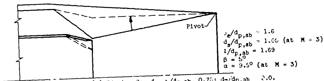
Figure 1. - Continued. Ejector geometries.
