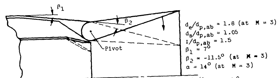
(f) Ejector 7: d_{p,nb}/d_{p,ab} = 0.75 ; d_m/d_{p,ab} = 2.0 .
