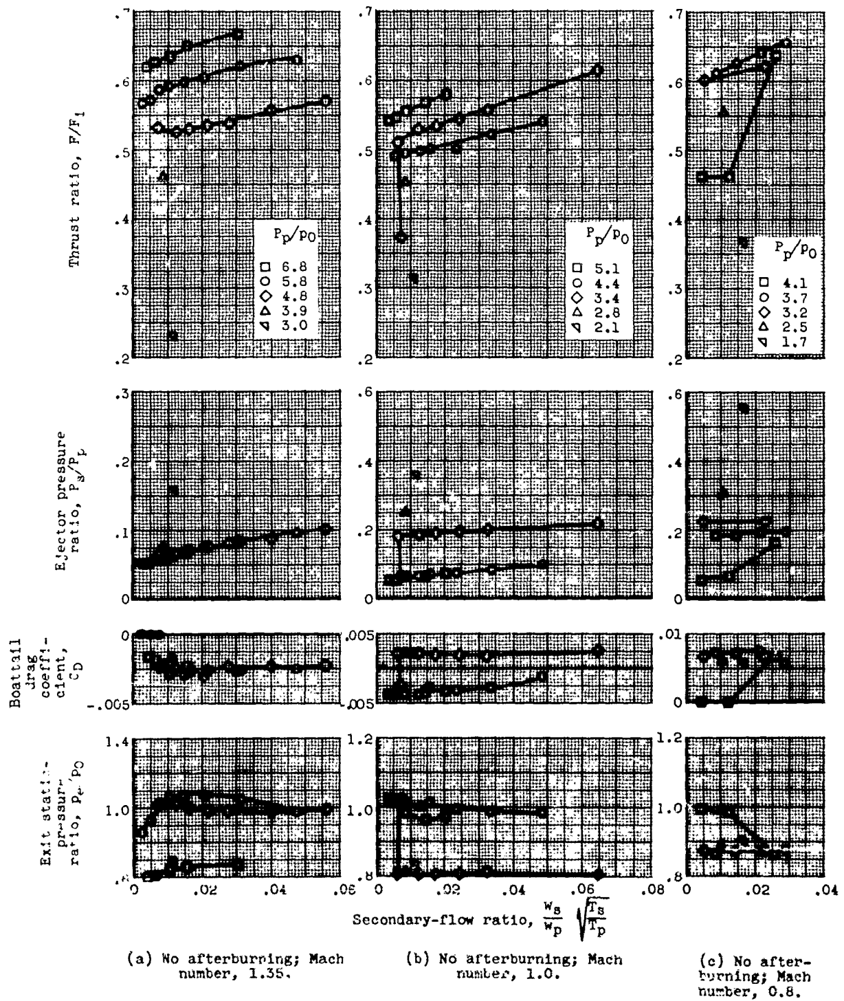
Figure 7. - Performance of ejector 2.
