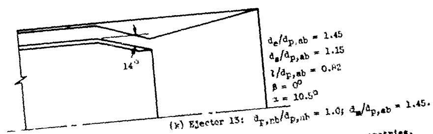
Figure 1. - Concluded. Ejector geometries.
