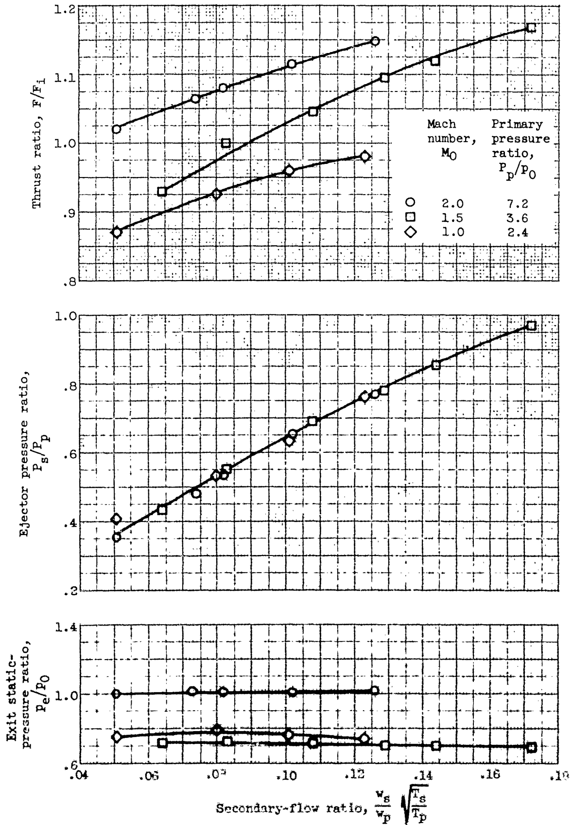
Figure 23. - Performance of ejector 17.
