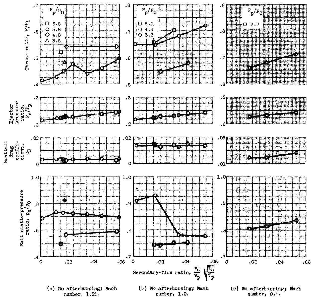
Figure 12. - Performance of ejector 1 with spoilers.
