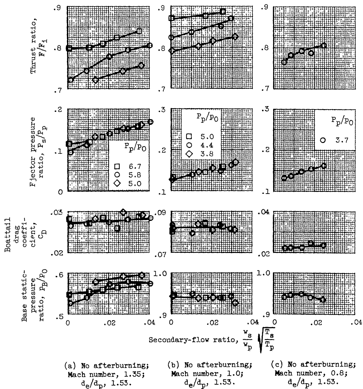
Figure 17. - Performance of ejector 8 without base flow.
