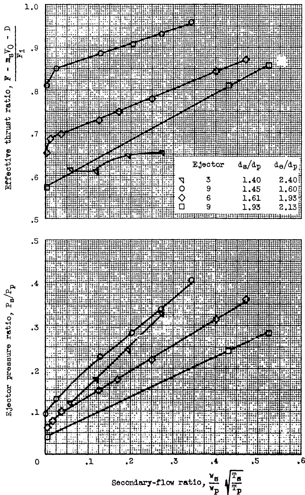
Figure 26. - Effect of secondary flow on fixed ejector performance at Mach 1.35.
