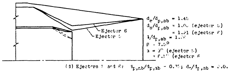
Figure 1. - Ejector geometries.
