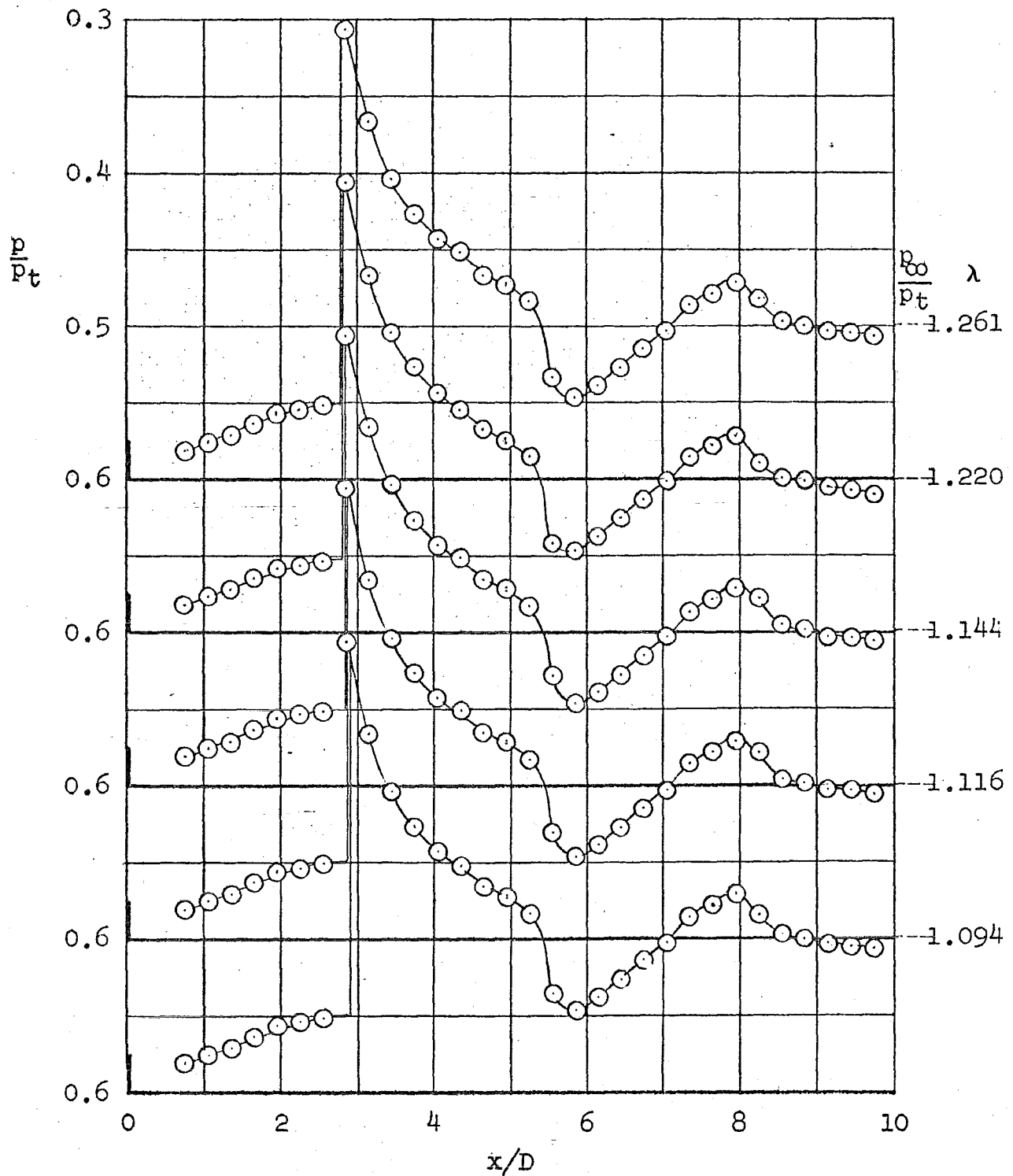
Fig. 10 Pressure Distributions on 10.0-diam Cone-Cylinder at M_\infty = 1.05
