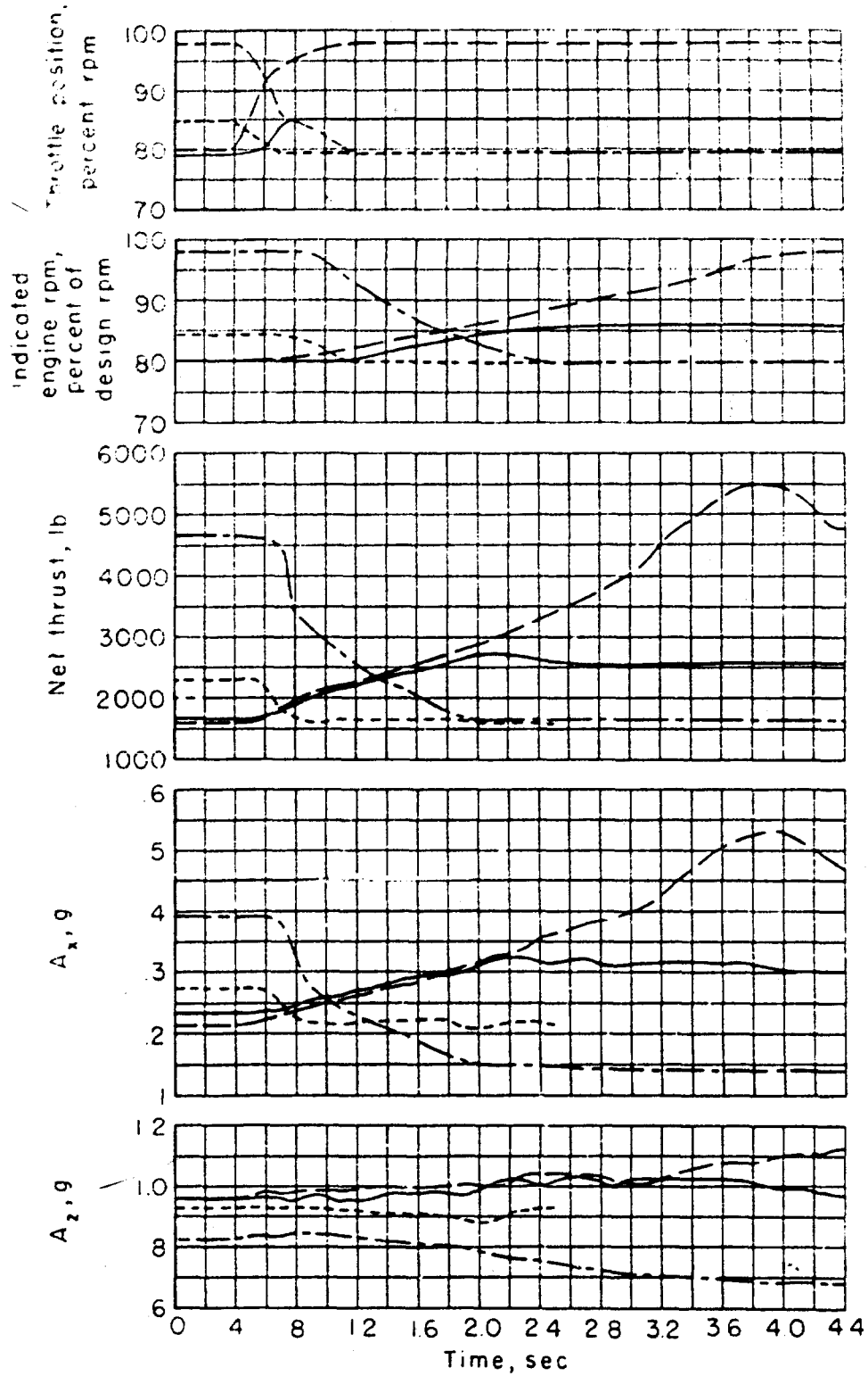
Figure 3.- Time histories of airplane and engine responses to step chrottle movements; FJ-3 airplane.
